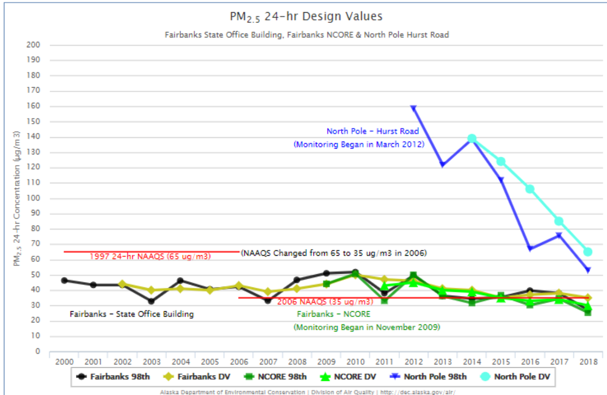
Figure 7.1-3 FNSB PM 2.5 Nonattainment Area Design Value and 98 th Percentile 24-hr PM 2.5 Concentrations 2000-2018
