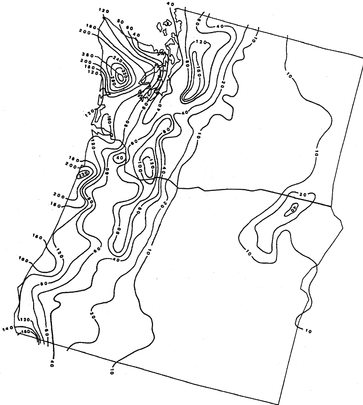
Figure 2-4. Isoerodent map of Oregon and Washington. Units are hundreds ft·tonf·in(ac·h·yr) -1 .
