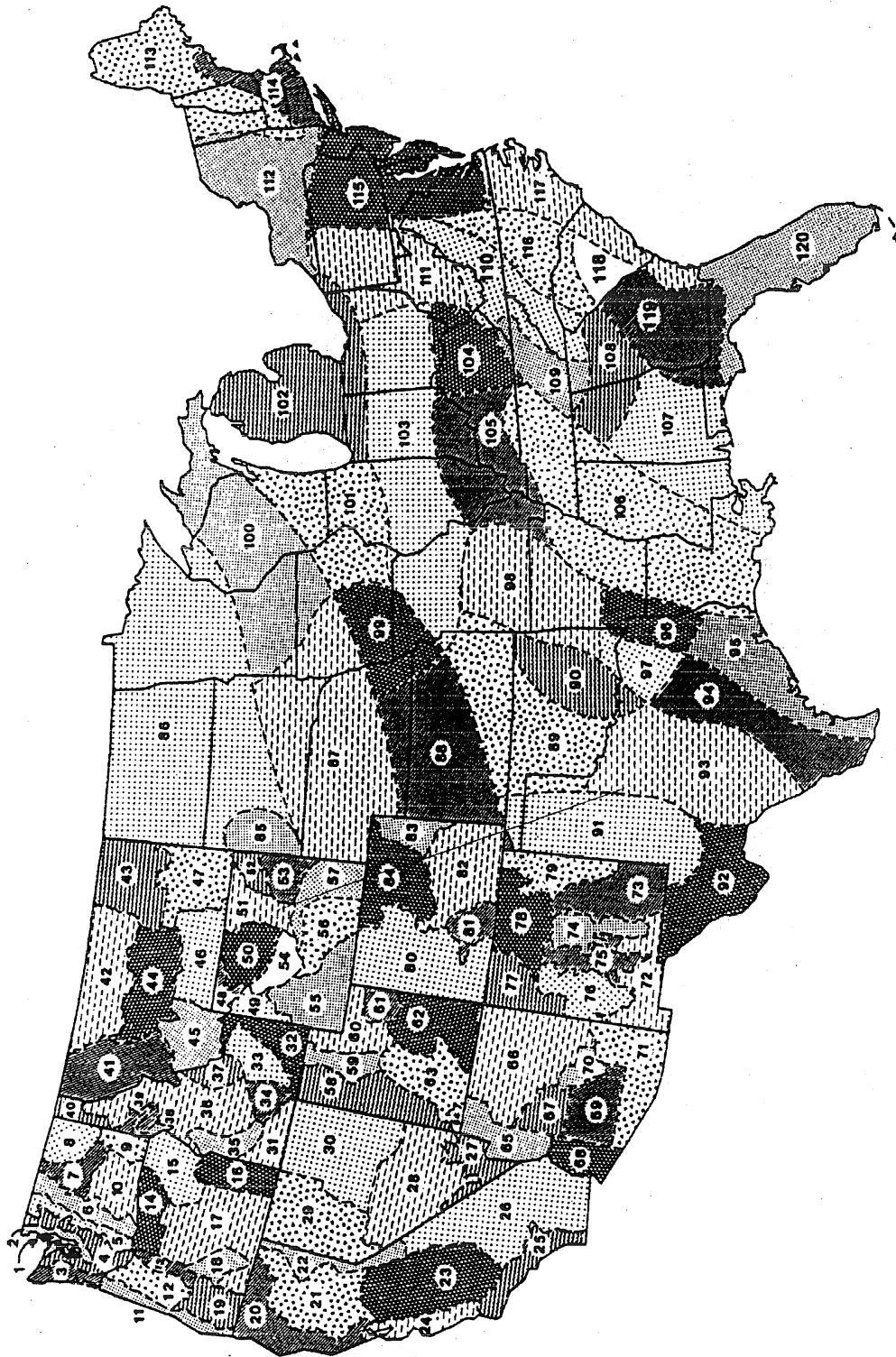
Figure 2-7. EI distribution zones for contiguous United States
