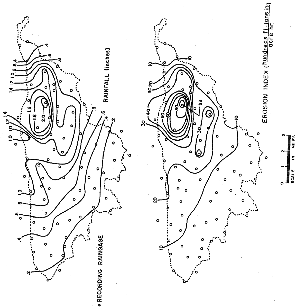
Figure 2-18. Annual precipitation (top) and iseroent (bottom) maps for 1964 on Walnut Gulch Experimental Watershed
