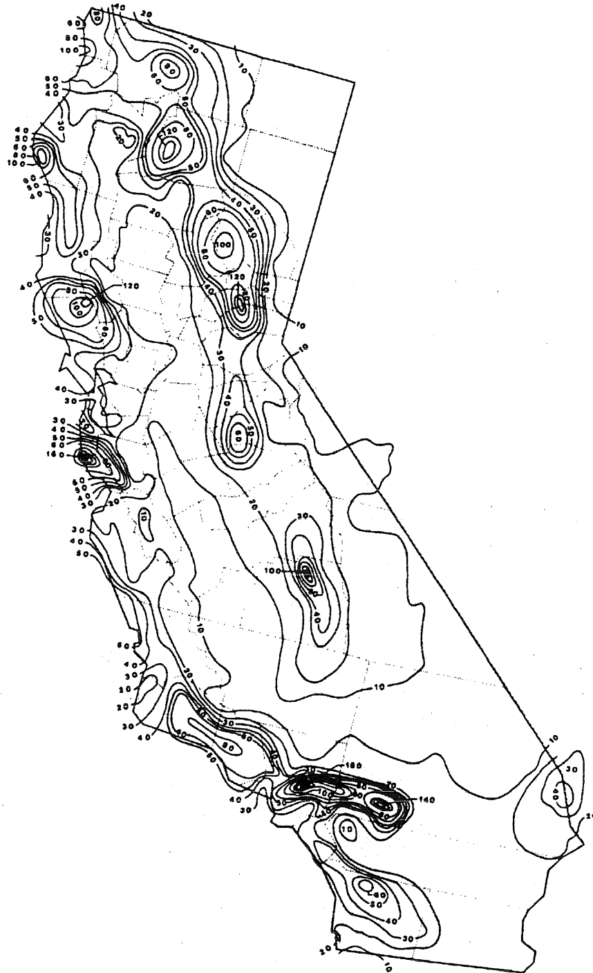
Figure 2-11. Ten-yr-frequency single-storm erosion index for California. Units are hundreds ft·tonf·in(ac·h) -1 .
