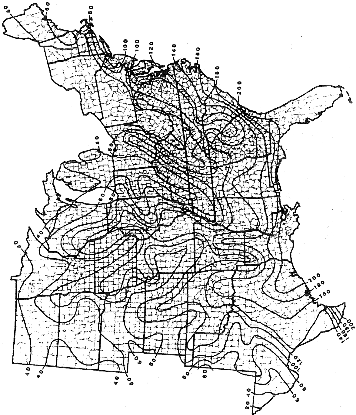
Figure 2-9. Ten-yr-frequency single-storm erosion index for eastern
