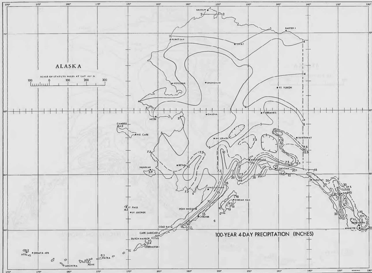
FIGURE 22—100-year 4-day precipitation (in.).
