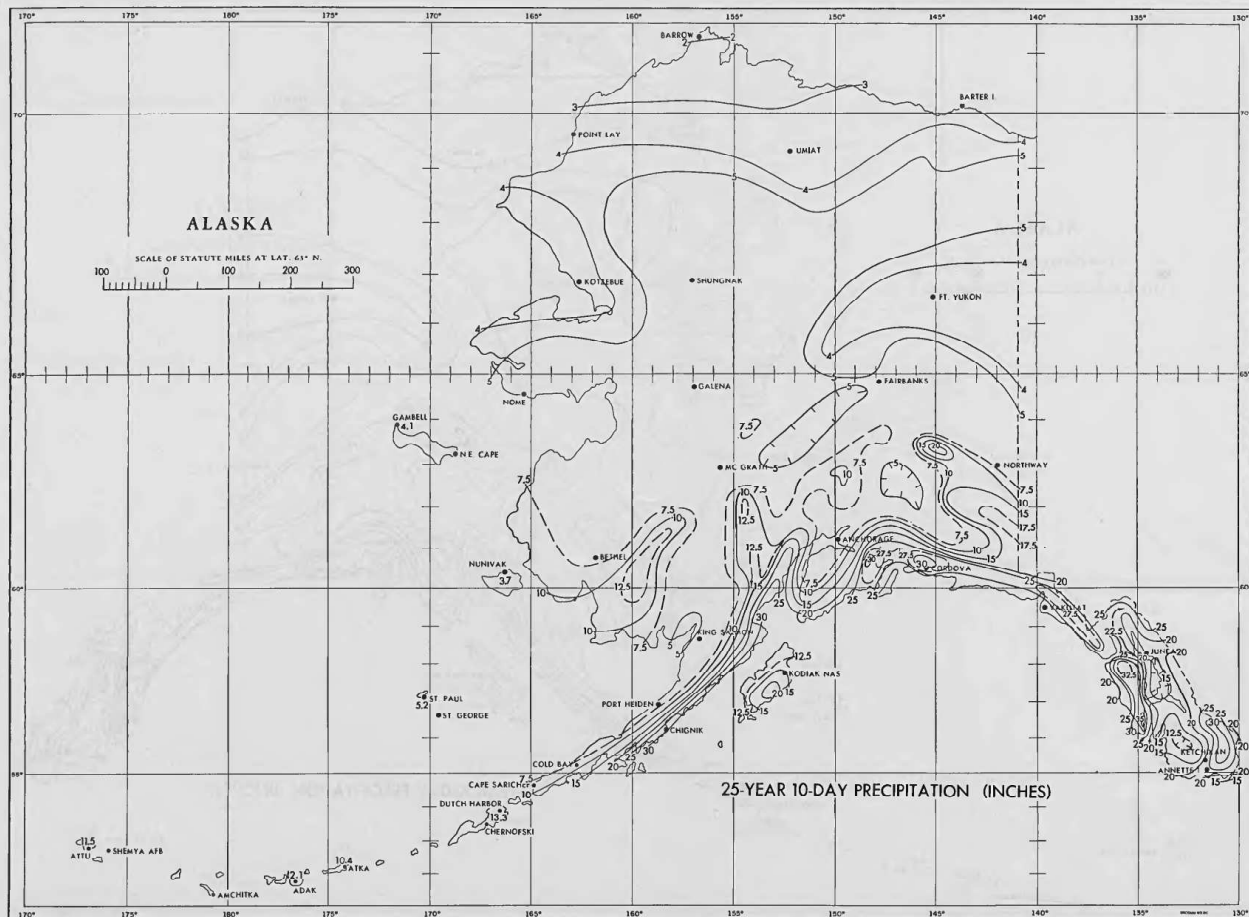
FIGURE 82.—25-year 10-day precipitation (in.).
