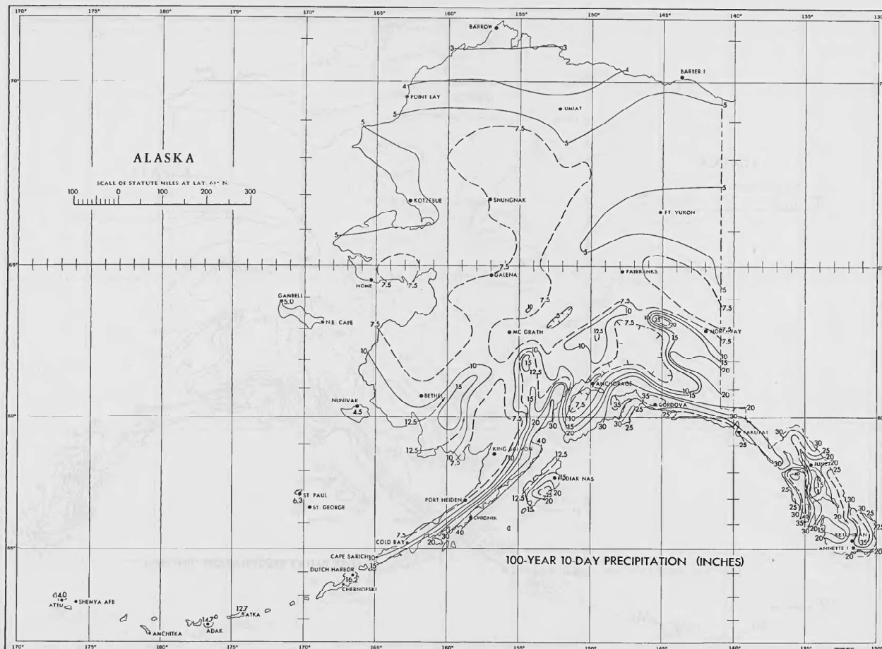
FIGURE 34.—100-year 10-day precipitation (in.).
