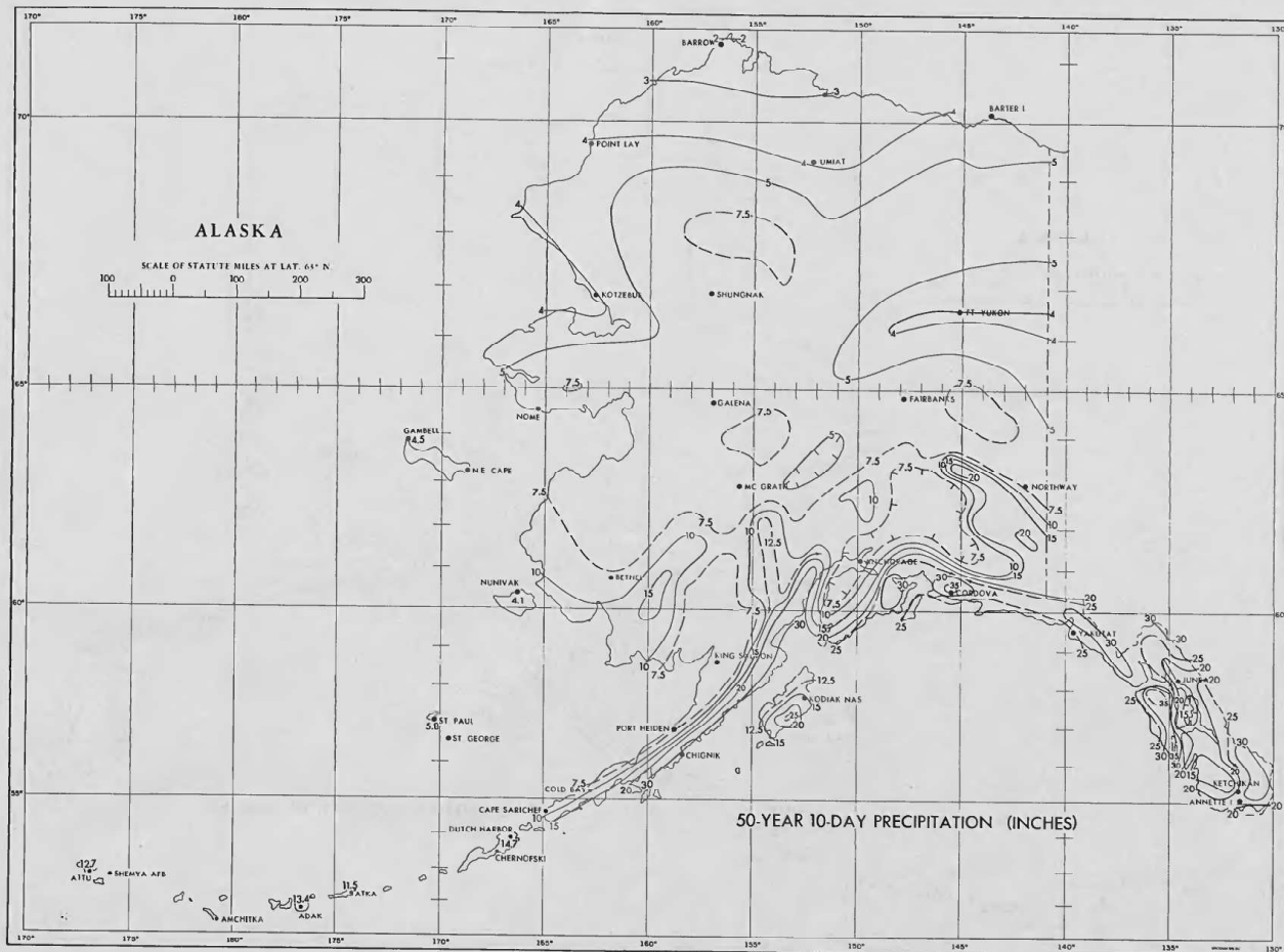
FIGURE 33.—50-year 10-day precipitation (in.).
