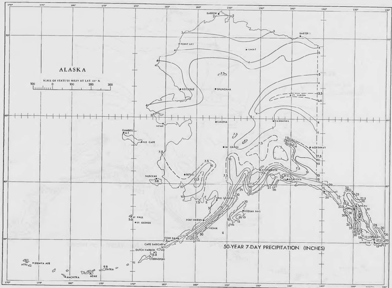
FIGURE 27.—50-year 7-day precipitation (in.).
