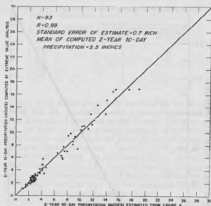
FIGURE 5.—Test of relation of figure 4.
