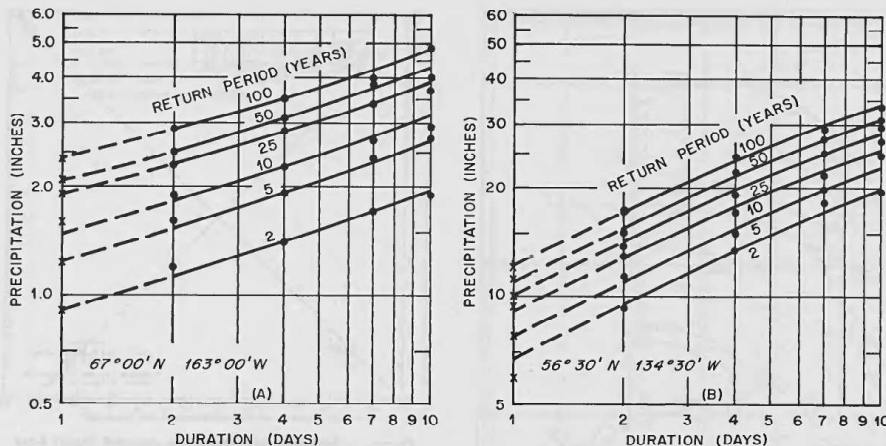
FIGURE 9.—Smoothing values read from isopluvial maps.
