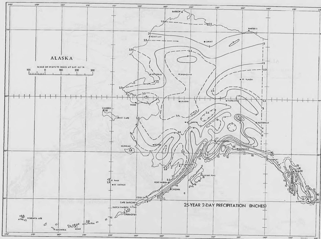
FIGURE 14.—25-year 2-day precipitation (in.).
