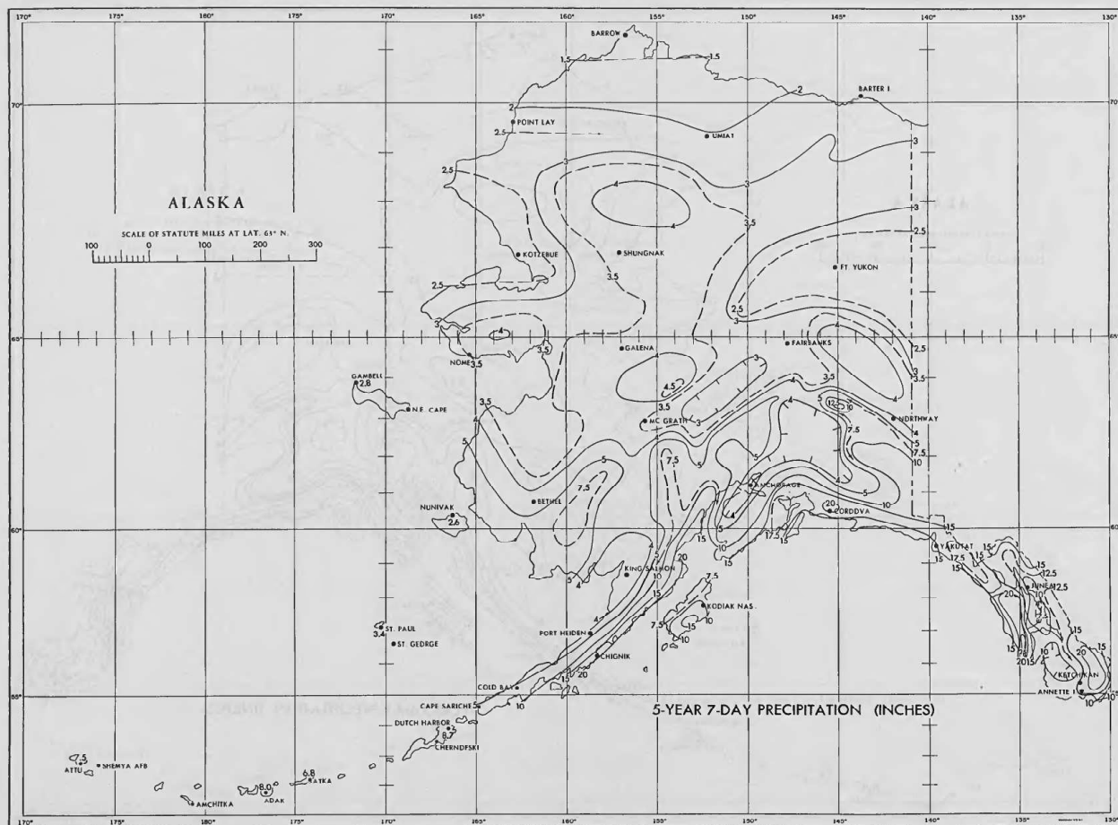
FIGURE 24.—5-year 7-day precipitation (in.).
