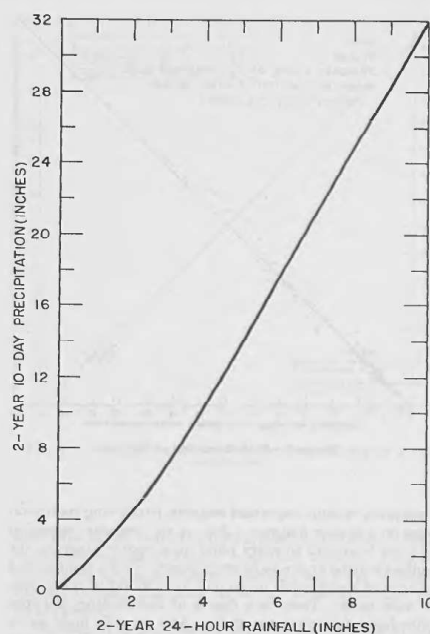
FIGURE 4.—Relation for estimating 2-year 10-day precipitation.
