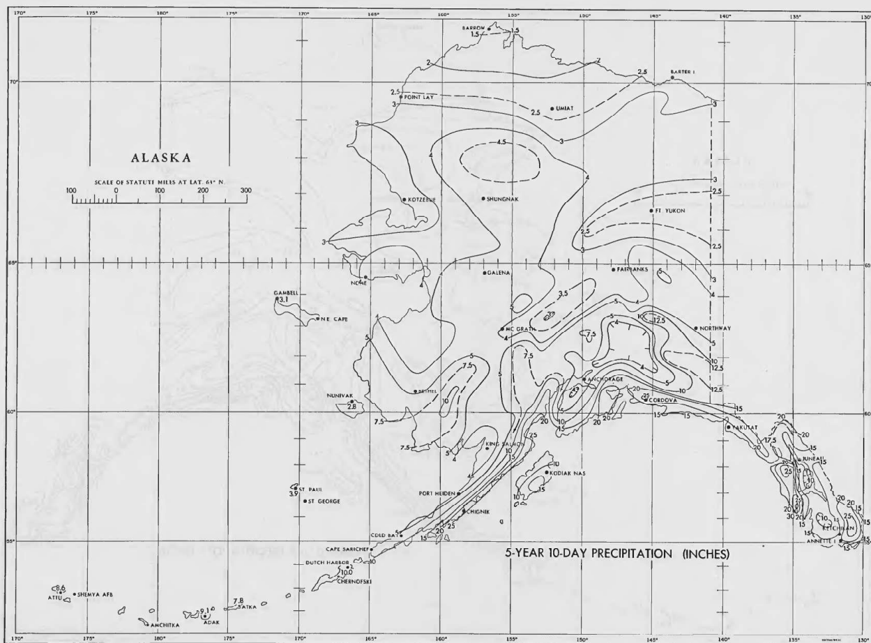
FIGURE 30.—5-year 10-day precipitation (in.).
