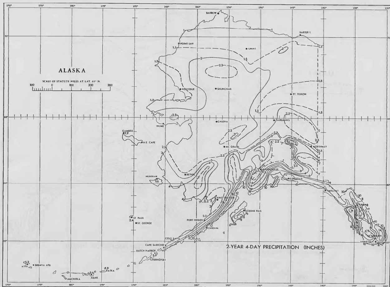
FIGURE 17.—2-year 4-dry precipitation (in.).
