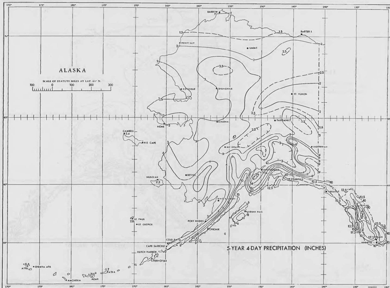
FIGURE 18.—5-year 4-day precipitation (in.).
