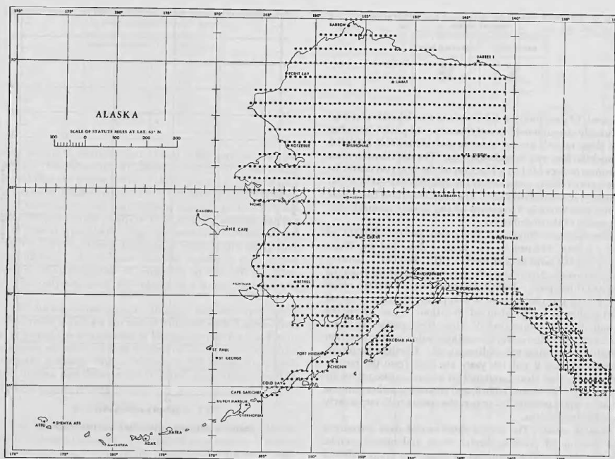
FIGURE 6.—Points for which precipitation-frequency data were computed.
