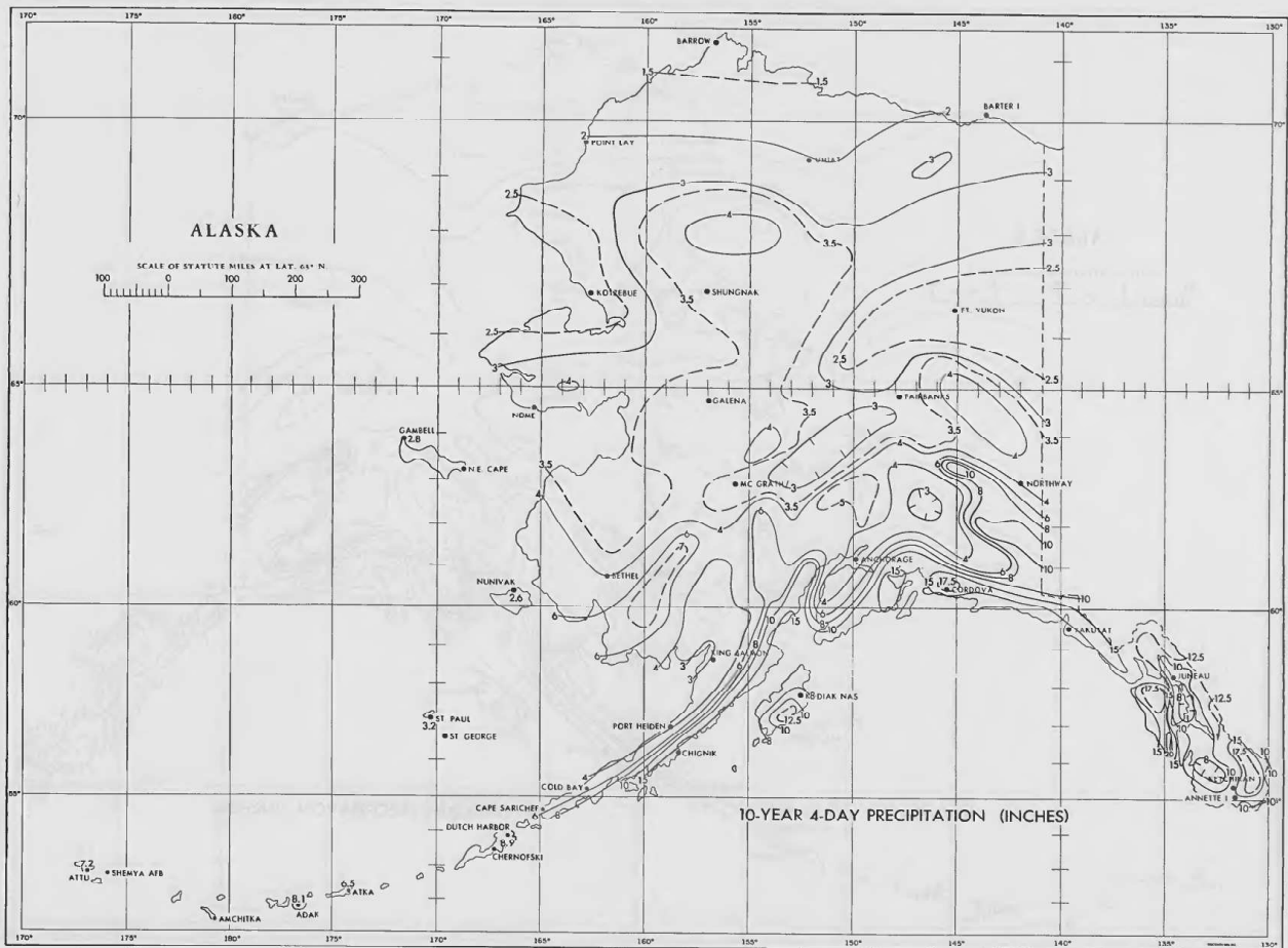
FIGURE 19.—10-year 4-day precipitation (in.).
