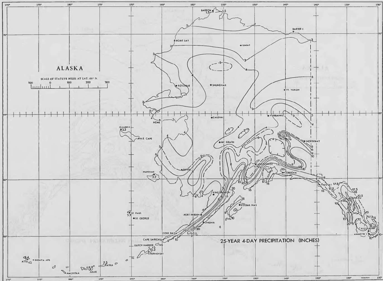
FIGURE 20.—25-year 4-day precipitation (in.).
