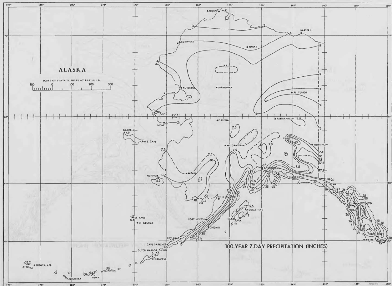
FIGURE 28.—100-year 7-day precipitation (in.).
