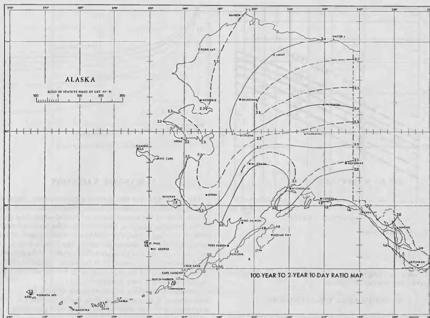
FIGURE 7.—100-year to 2-year 10-day ratio map.
