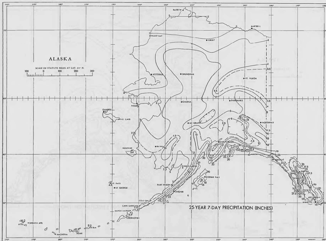
FIGURE 26.—25-year 7-day precipitation (in.).
