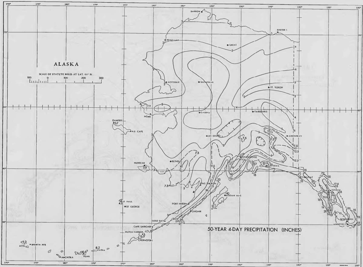
FIGURE 21.—50-year 4-day precipitation (in.).
