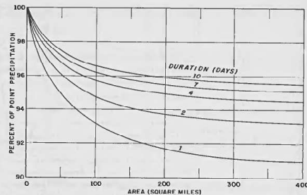
FIGURE 10.—Depth-area curves.
