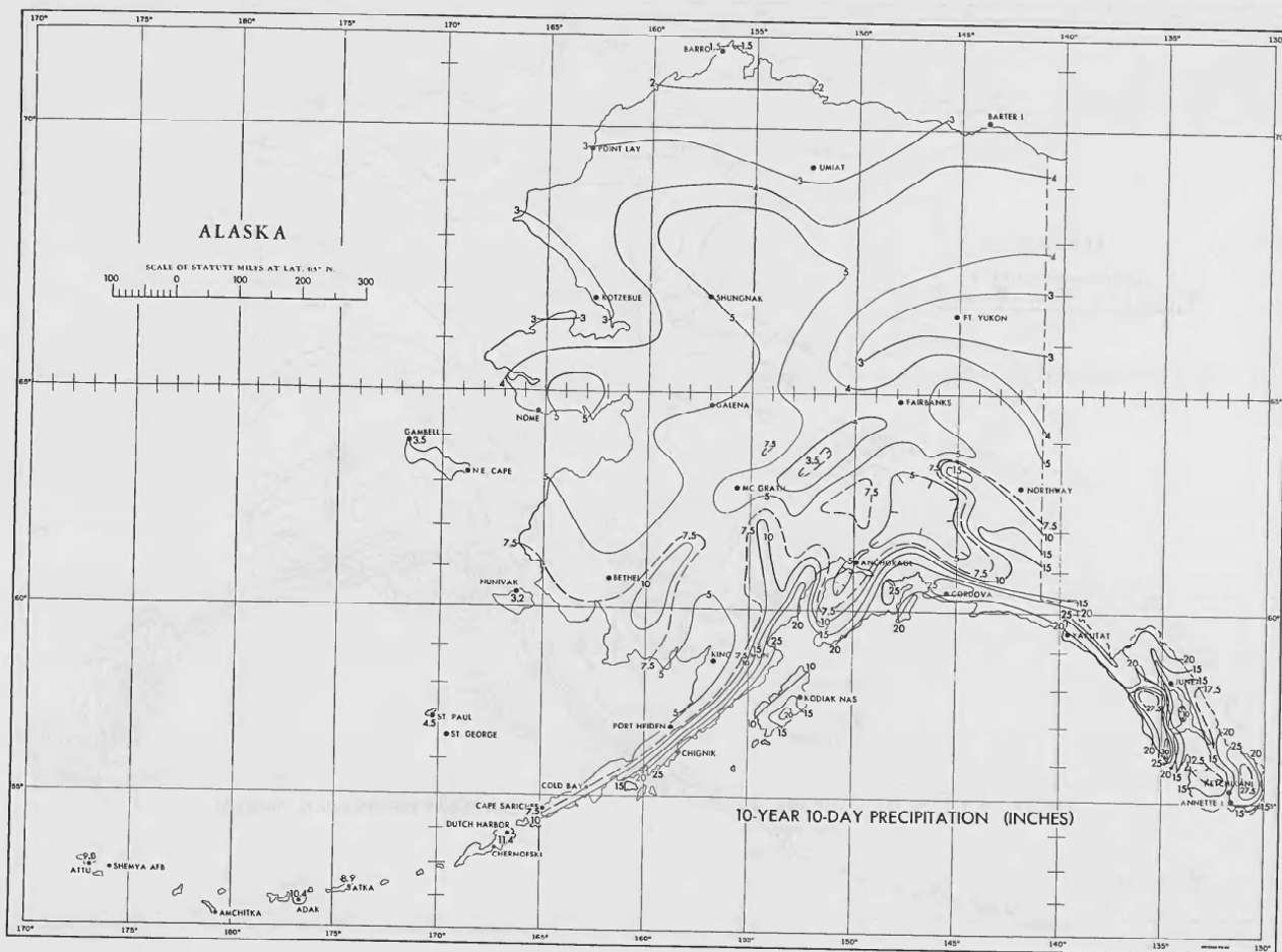
FIGURE 31.—10-year 10-day precipitation (in.).
