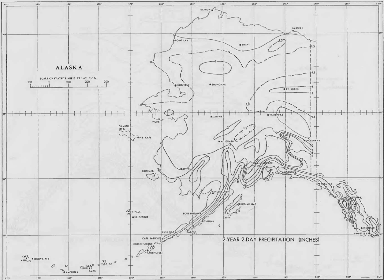
FIGURE 11.—2-year 2-day precipitation (in.).
