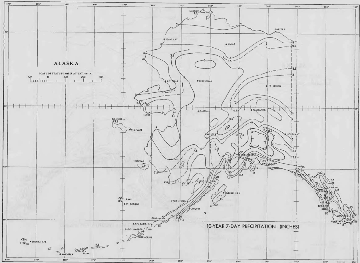
FIGURE 25.—10-year 7-day precipitation (in.).
