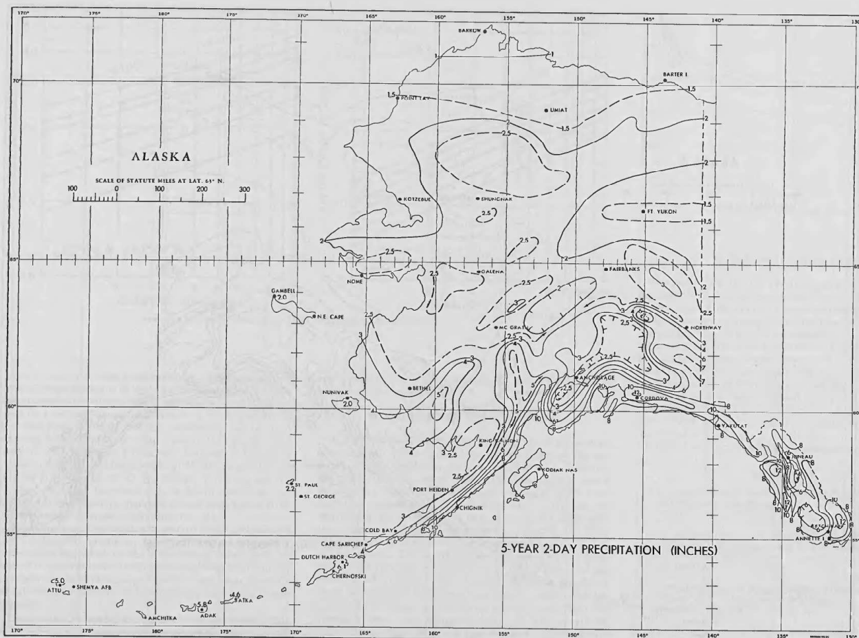
FIGURE 12.—5-year 2-day precipitation (in.).
