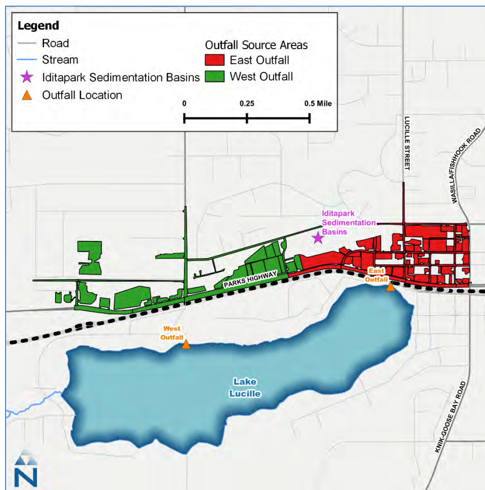
Figure 4-1. Land areas draining to the east and west Lake Lucile outfalls (ARRI, 2019).
