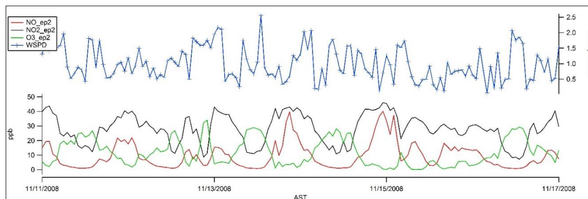
Figure 7.8-28. CMAQ modeling output for episode 2 for NO (red), NO 2 (black), O 3 (green) all in ppb and wind speed (blue) in m/s.
