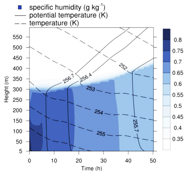
Figure 2. Modeled meteorological parameters include temperature (dashed contours), potential temperature (solid contours), and specific humidity (blue). The boundary layer height is initialized to be 300 m.
