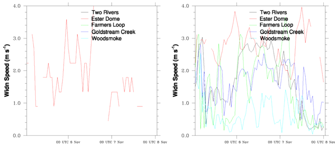
Figure 18: Same as Figure 17, but for wind speed.
