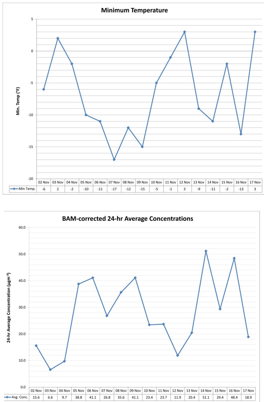
Figure 5 – Plot showing the daily minmun temperatures for the November episode in the Fairbanks region in Farenheit (top) and the BAM-corrected 24-hr average concentration of PM2.5 (bottom). Courtesy Bob Dulla, Sierra Research.
