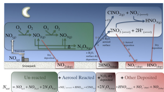
Figure 1. A nocturnal nitrogen schematic with emphasis on N 2 O 5 reactivity. The total nitrogen equation (N tot ) is a sum of the total column-integrated nitrogen from emitted NO x , divided into speciation fractions.
