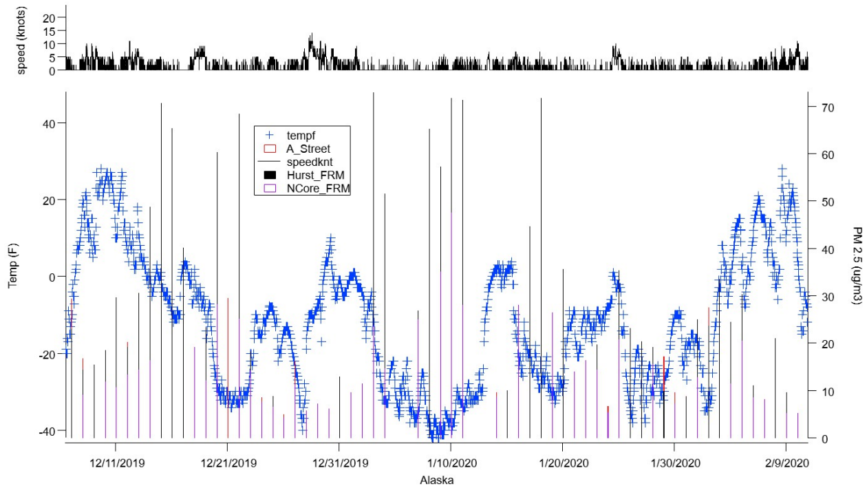
Figure 2.1. Proposed WRF episode for Fairbanks winter 2019-2020
