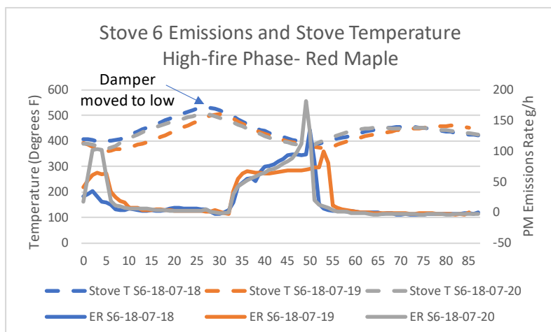
Figure 41. Stove 6—Red Maple IDC High-Fire Phase Emissions and Stove Temperature Profile
