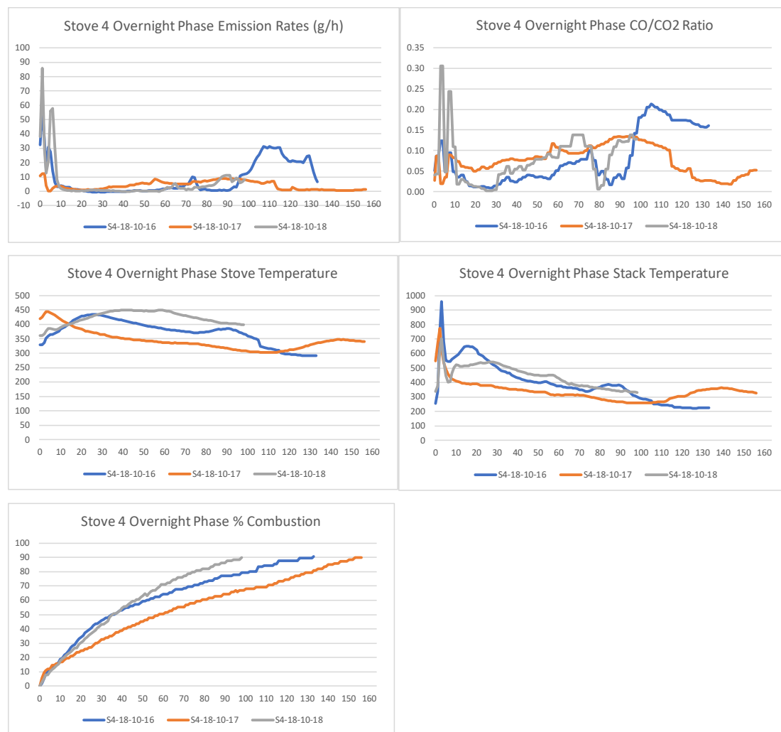
Figure 118. Stove 4 Overnight Phase Profiles
