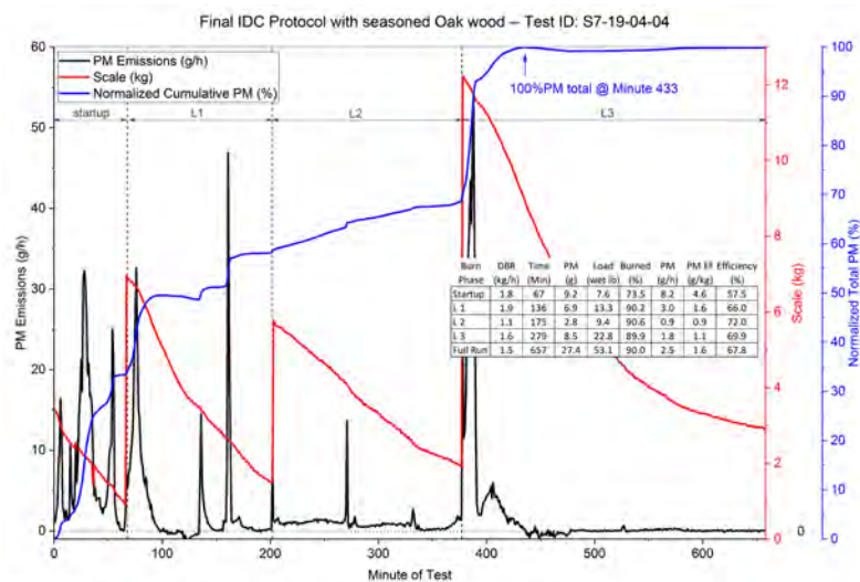
Figure 52. Stove 7—IDC Final Protocol Replicate Runs with Seasoned Oak Cordwood
