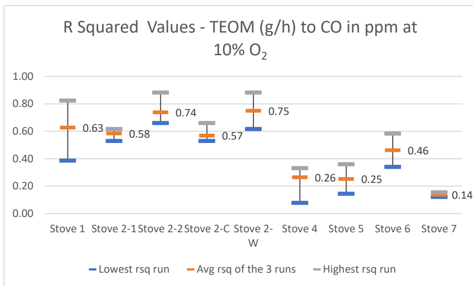
Figure 104. Correlation between One-Minute CO and PM Measurements by Stove
