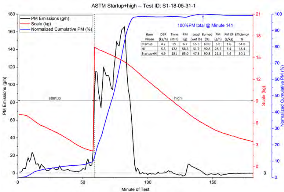
Figure 3. Stove 1—ASTM 3053-17 Runs—Start-Up and High-Fire Phases
