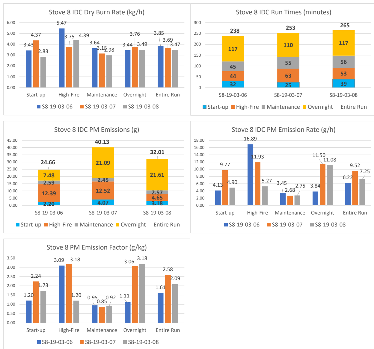
Figure 126. Stove 8 IDC Run Parameters
