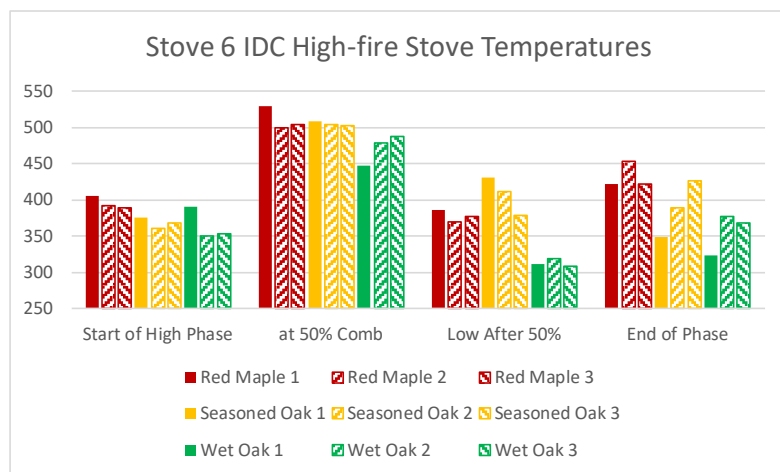
Figure 93. High-Fire Phase Stove Temperatures
