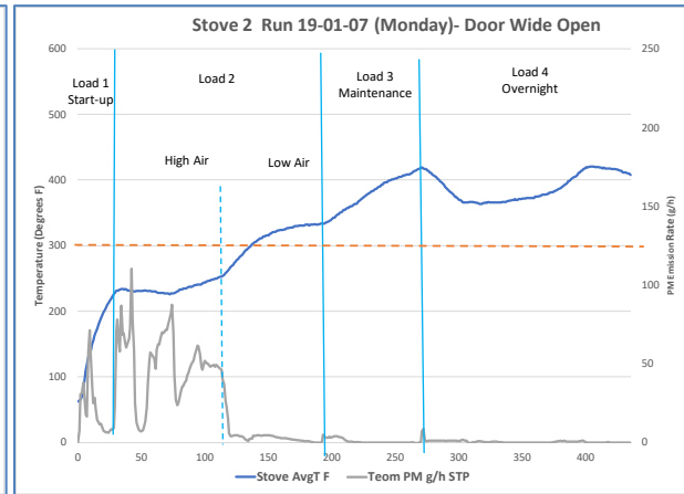
Stove 2—January 2019 IDC Runs
