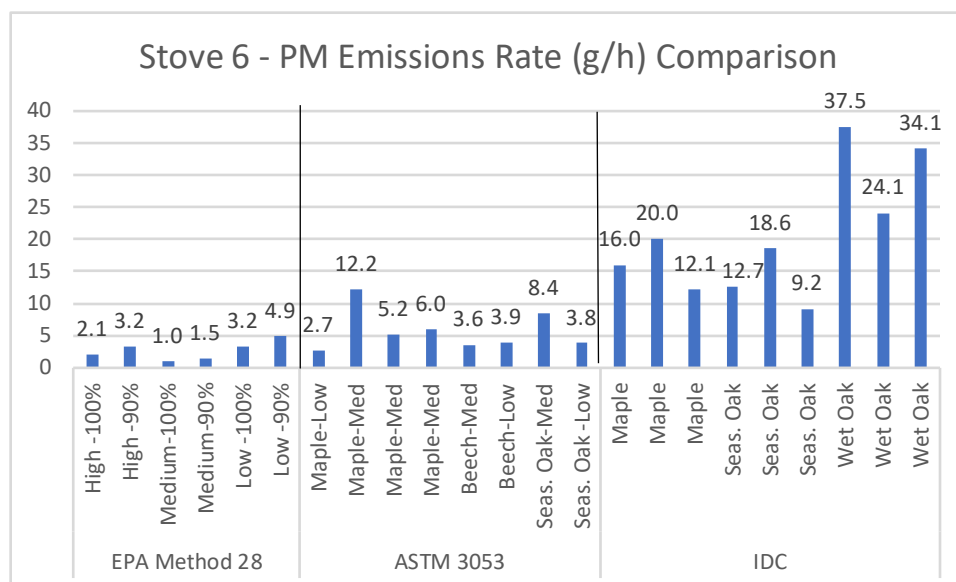
Figure 45. Stove 6—Comparison of Method 28, ASTM 3053-17, and IDC Final Protocol Emission Rate Measurements
