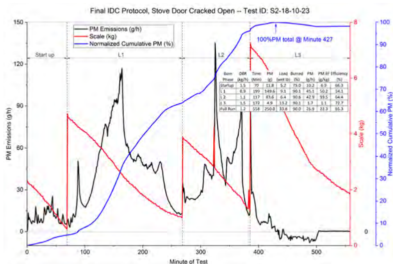
Figure 13. Stove 2—IDC Final Protocol Runs—October 2018
