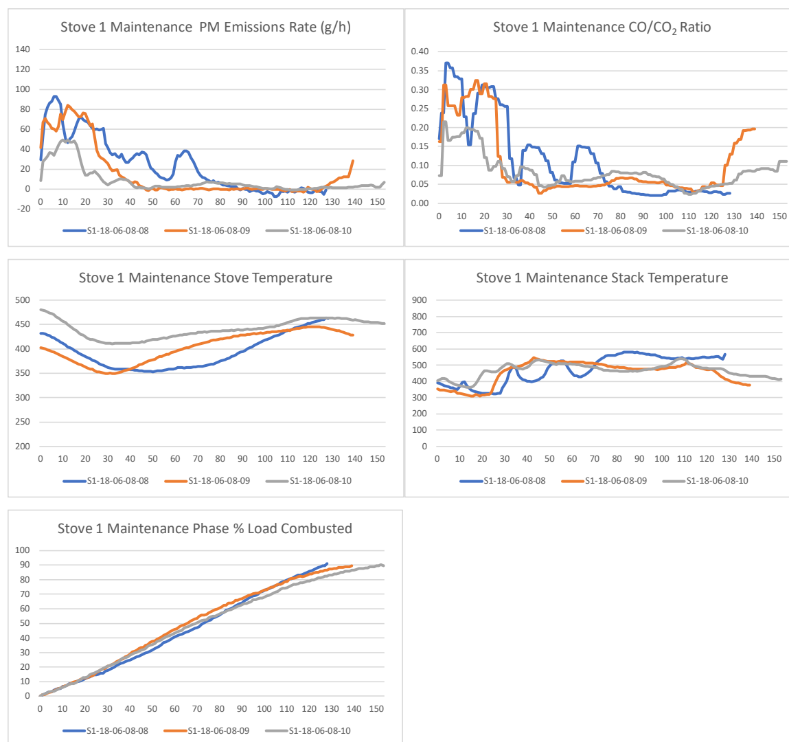
Figure 111. Stove 1 IDC Maintenance Phase Profiles
