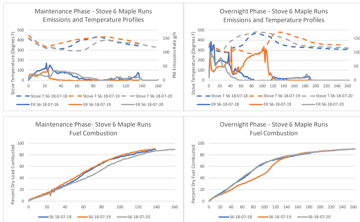
Figure 44. Stove 6—Comparison of Emission and Temperature Profiles and Fuel Combustion Curves for the Maintenance and Overnight Phases of the Red Maple IDC Runs
