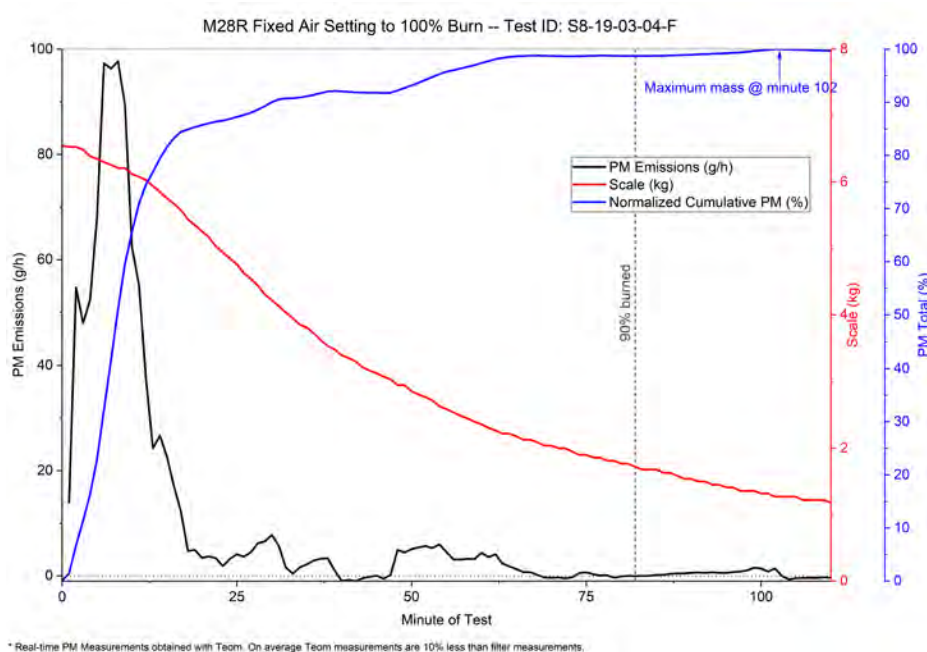
Figure 60. Stove 8—M28 Baseline Test Results
