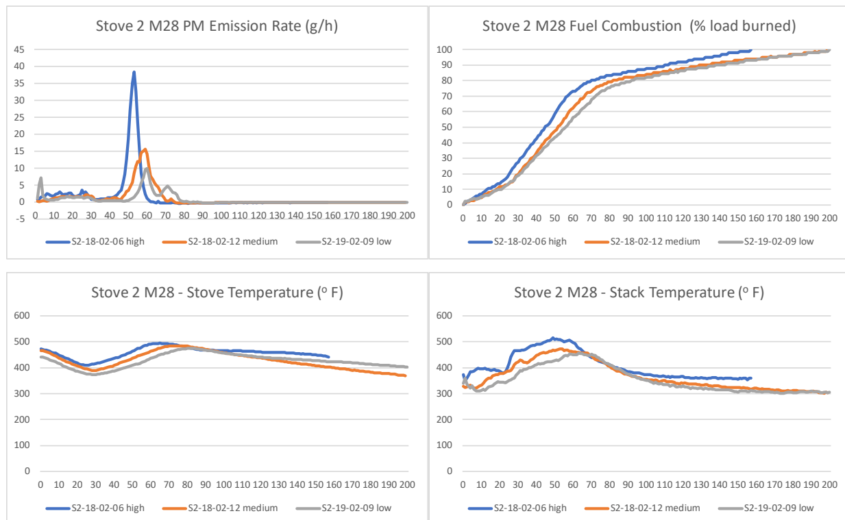
Figure 12. Stove 2—Baseline Runs—PM Emissions, Cumulative Fuel Consumption, and Stove and Stack Temperature Profiles
