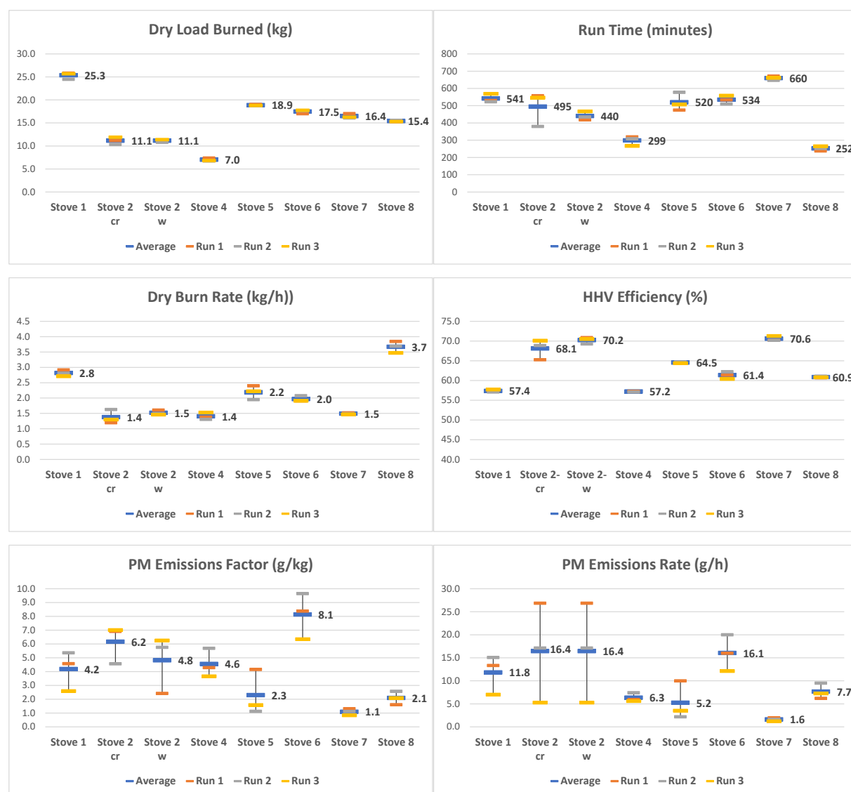
Figure 107. Run Parameters—Entire IDC Protocol
