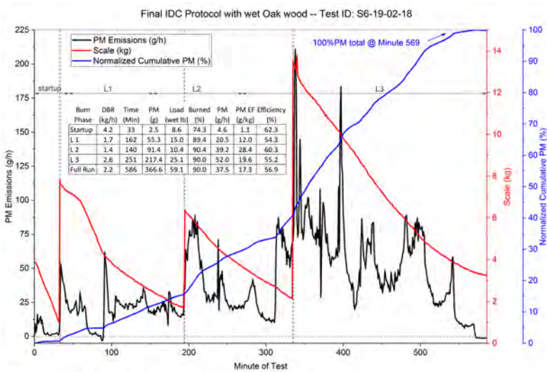
Figure 40. Stove 6—IDC Final Protocol Replicate Runs with Wet Oak Cordwood
