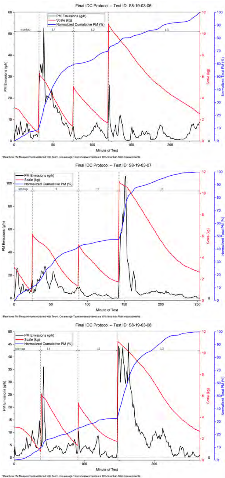
Figure 63. Stove 8—IDC Final Protocol Replicate Runs with Red Maple Cordwood
