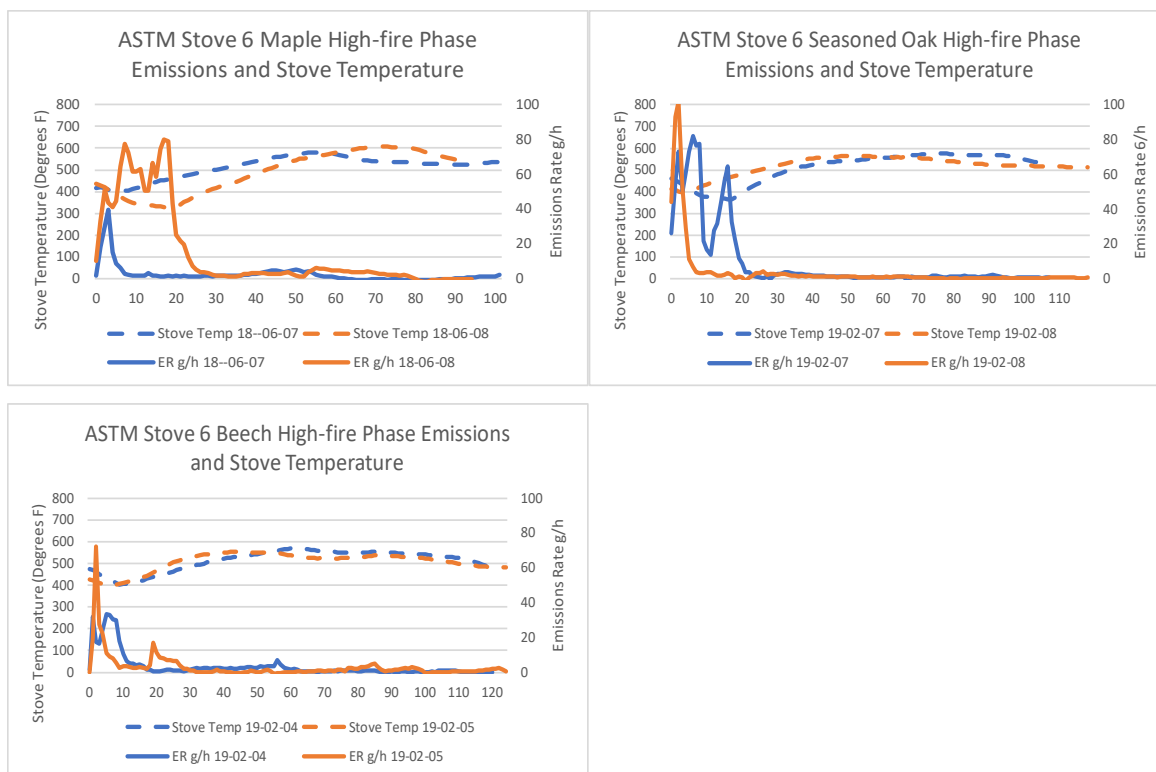
Figure 91. Stove 6—ASTM 3053-17 High-Fire Phase Emissions and Temperature Profiles
