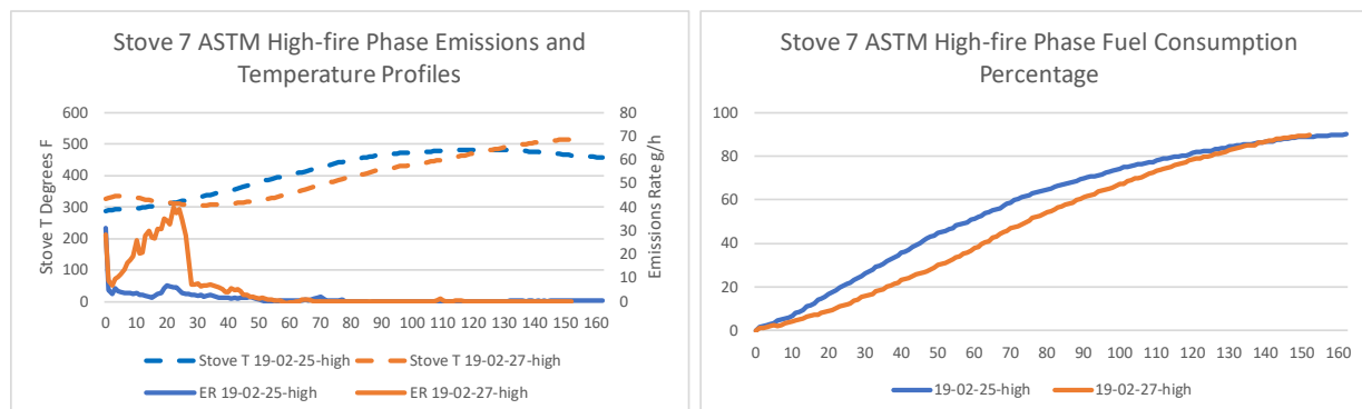
Figure 50. Stove 7—ASTM 3053-17 High-Air Phase Emissions, Stove Temperatures, and Fuel Combustion
