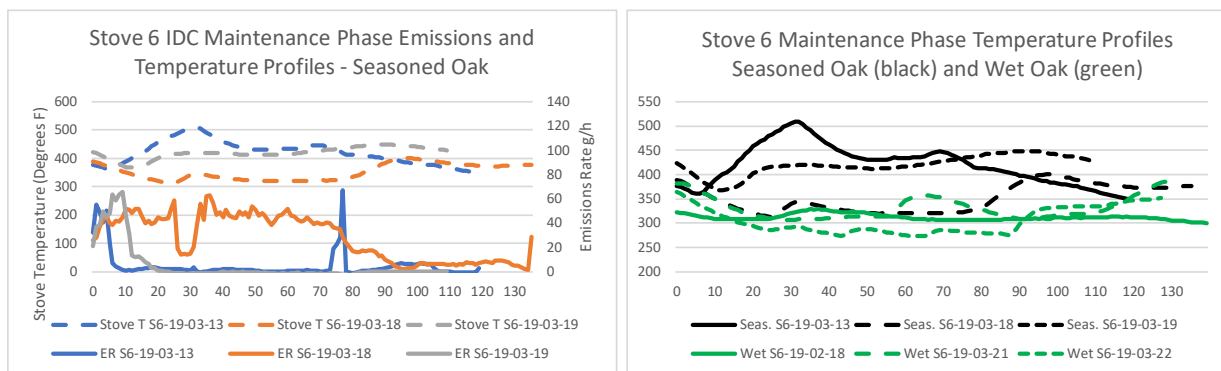
Figure 42. Stove 6—Variability in Seasoned Oak Maintenance Phase Emissions and Temperatures
