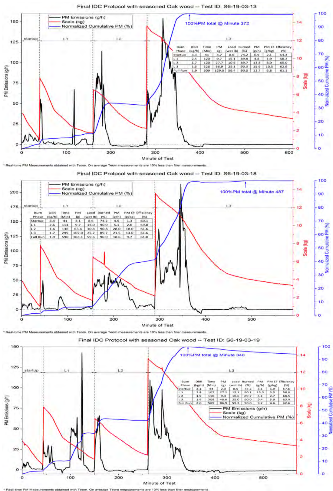
Figure 39. Stove 6—IDC Final Protocol Replicate Runs with Seasoned Oak Cordwood
