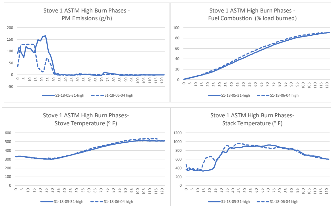
Figure 5. Stove 1—ASTM 3053-17 High-Burn Phases—PM Emission, Cumulative Fuel Consumption and Stove Temperature Profiles
