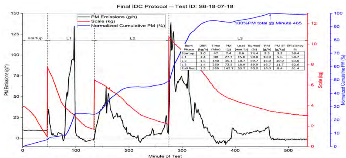
Figure 38. Stove 6—IDC Final Protocol Replicate Runs with Red Maple Cordwood
