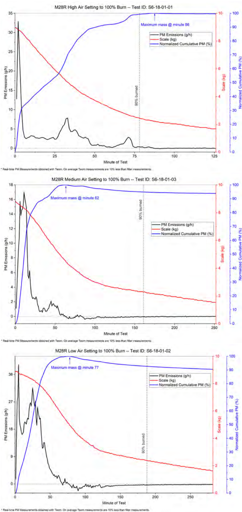
Figure 32. Stove 6—M28 Baseline Test Results
