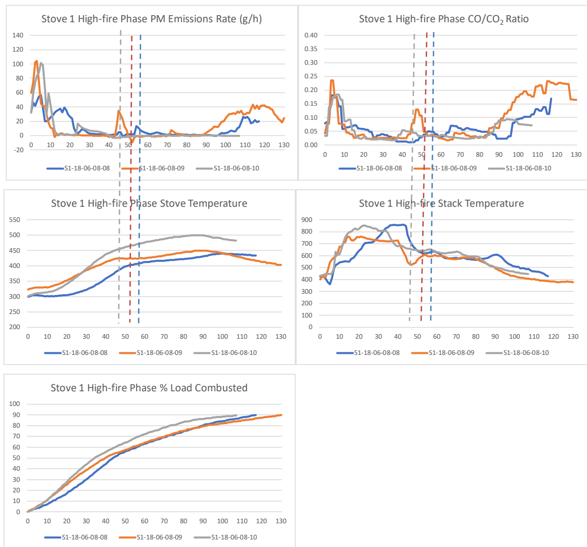
Figure 110. Stove 1 IDC Run Profiles for the High-Fire Phase
