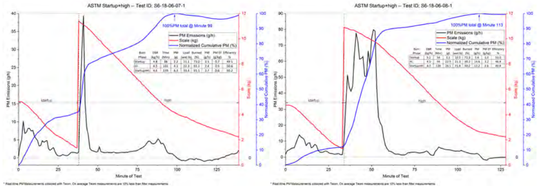
Figure 34. Stove 6—ASTM 3053-17 Runs—Start-Up and High-Fire Phases
