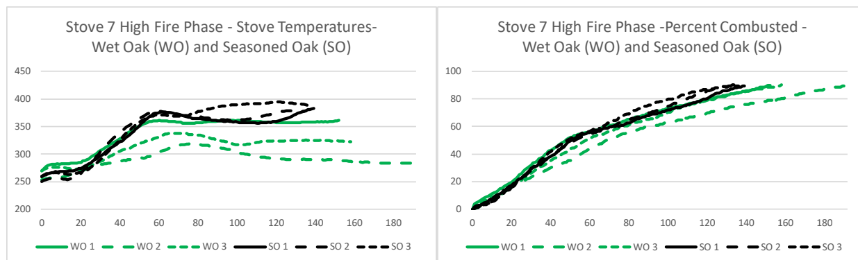
Figure 55. Stove 7—IDC High-Fire Phase—Seasoned and Wet Oak—Stove Temperatures and Fuel Consumption
