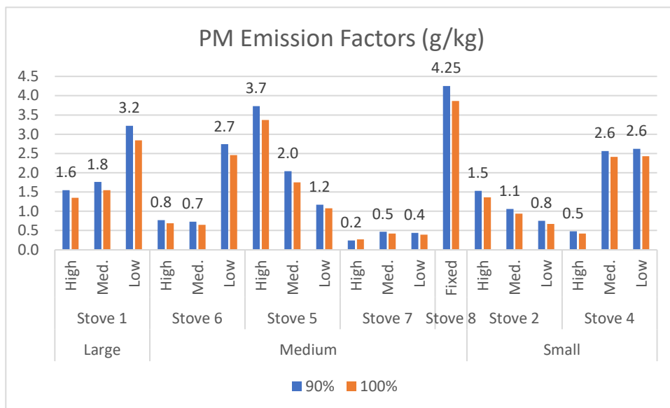
Figure 75. PM Emission Factors at 90% and 100% Combustion
