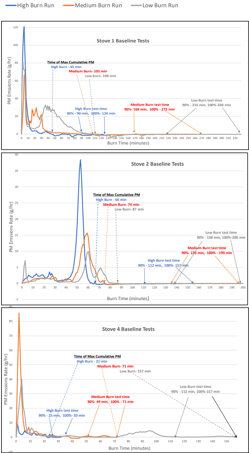
Figure 74. M28 Run Emission Profiles
