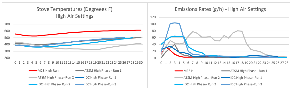
Figure 46. Stove 6—Comparison of Temperature Profiles and Emission Rates in Burns at High-Air Setting
