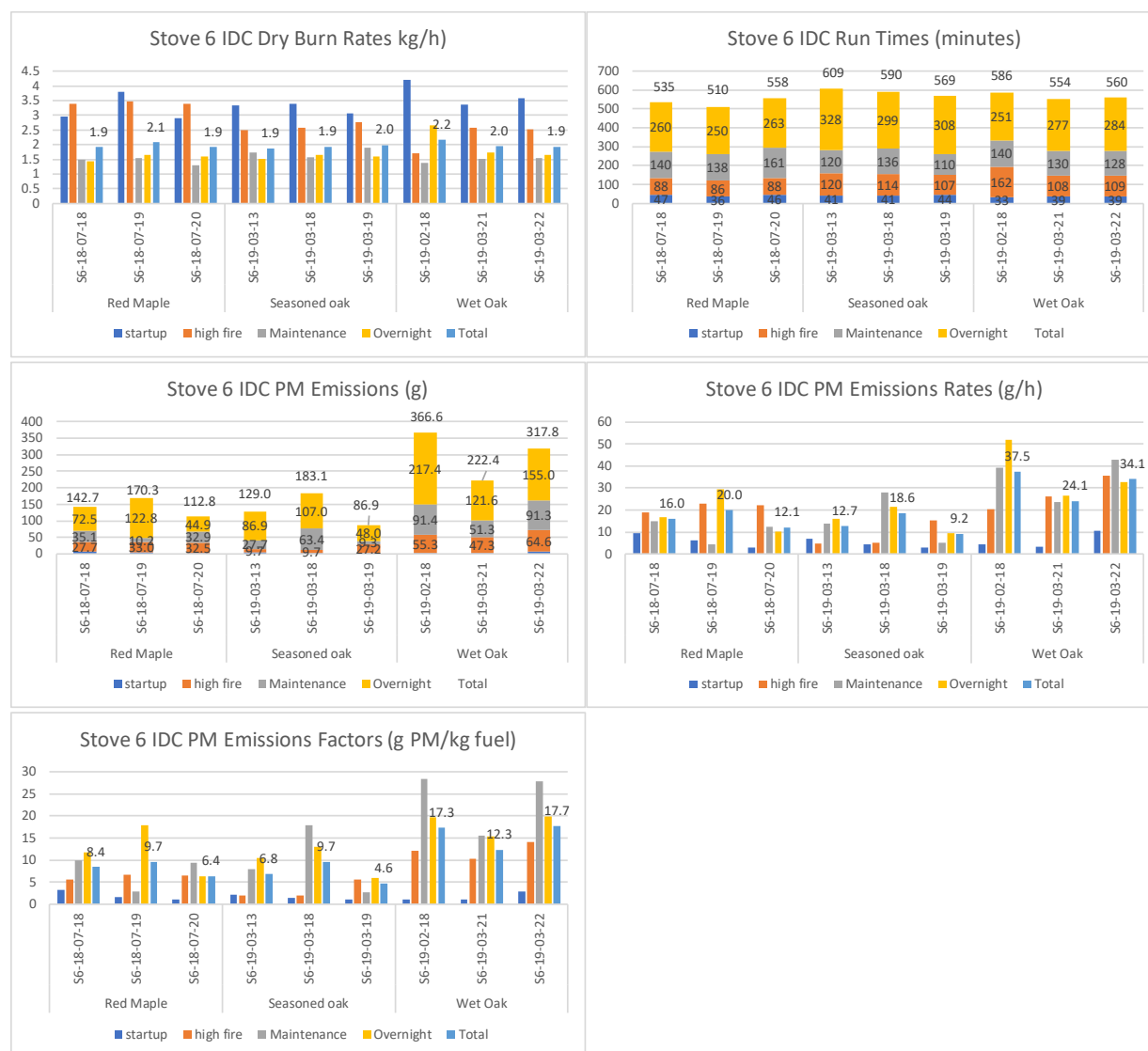
Figure 43. Stove 6—Comparison of Metrics for IDC Replicate Runs
