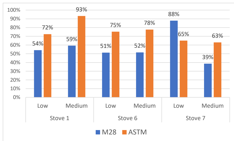
Figure 101. Percent Difference Between PM Emissions Rates (ER) at 100% and 90% Load Combustion in ASTM 3053-17 and M28 Medium- and Low-Air Runs
