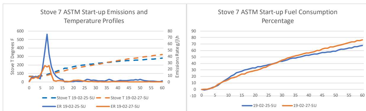
Figure 49. Stove 7 ASTM 3053-17 Start-Up Emissions, Stove Temperatures, and Fuel Combustion
