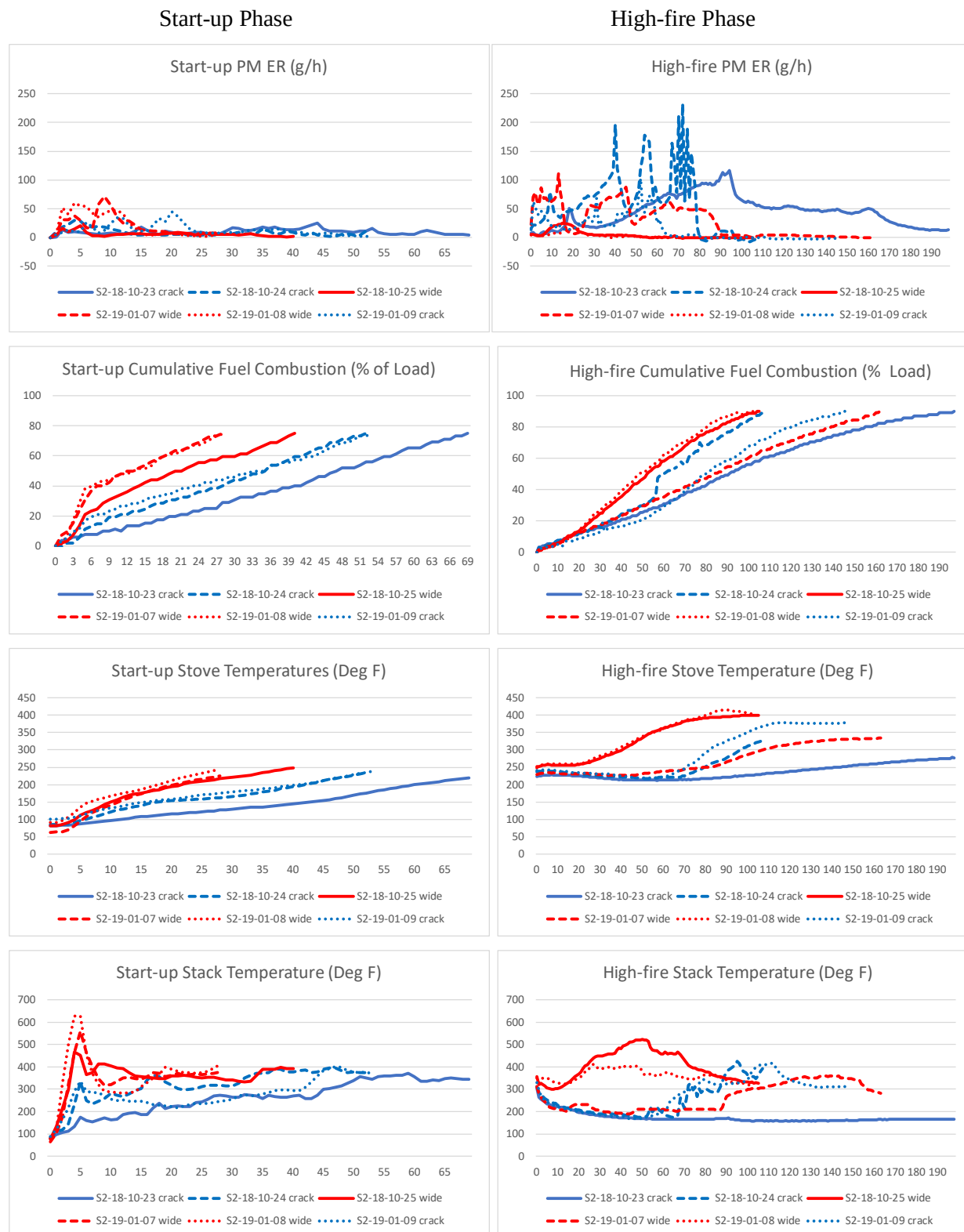
Figure 82. PM Emissions Profiles, Cumulative Fuel Consumption, and Temperature Profiles—Start-Up and High-Fires Phase of Stove 2 IDC Runs
