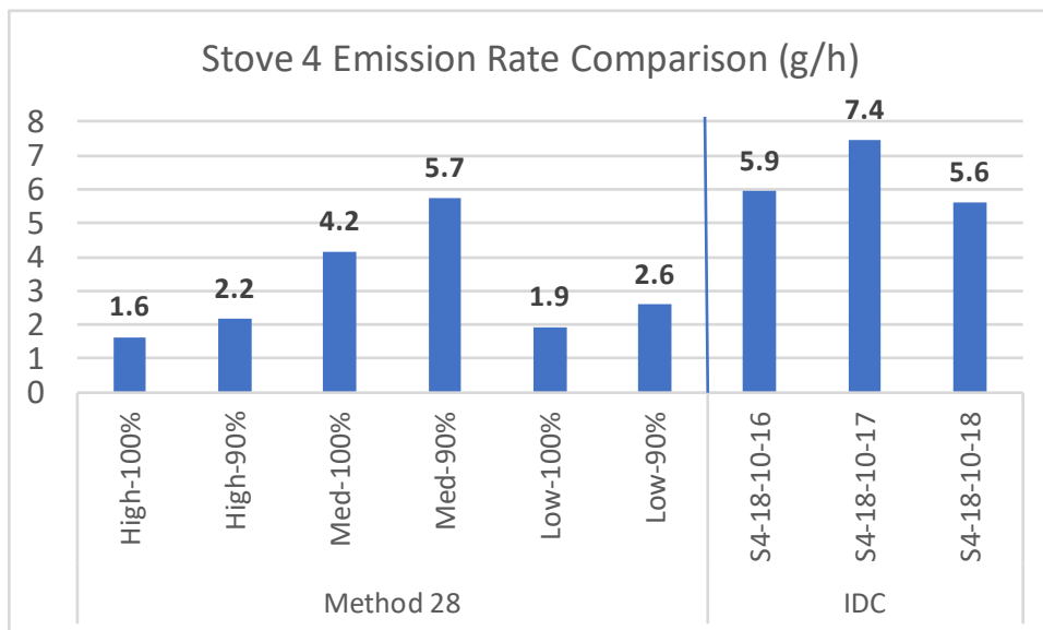
Figure 24. Stove 4—Comparison of Method 28 and IDC Emission Rate Measurements
