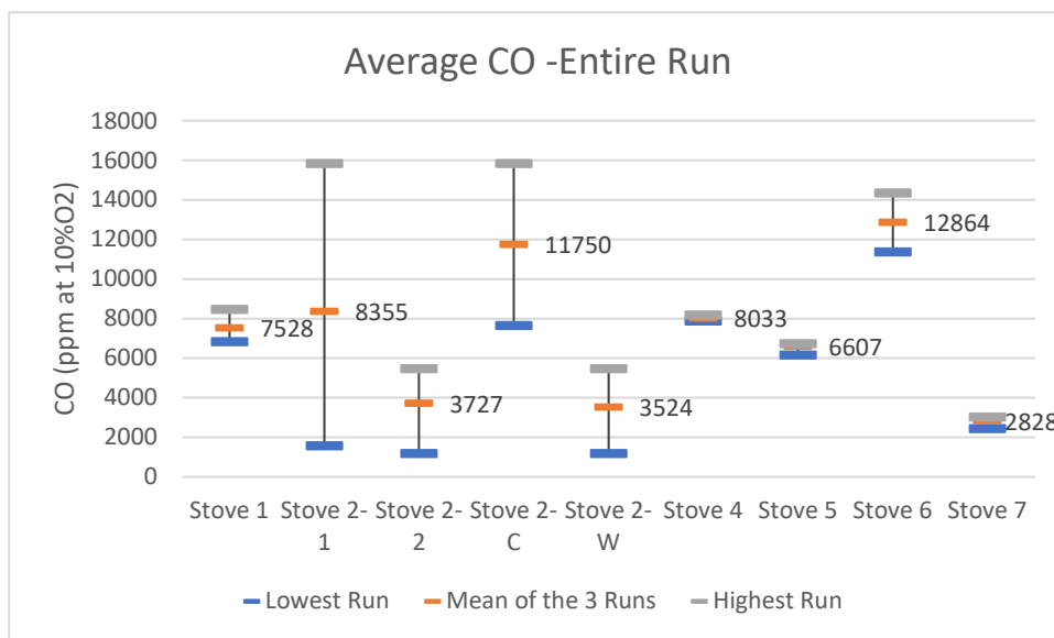
Figure 102. Average CO Concentration (in ppm at 10% O 2 )—Entire IDC Runs
