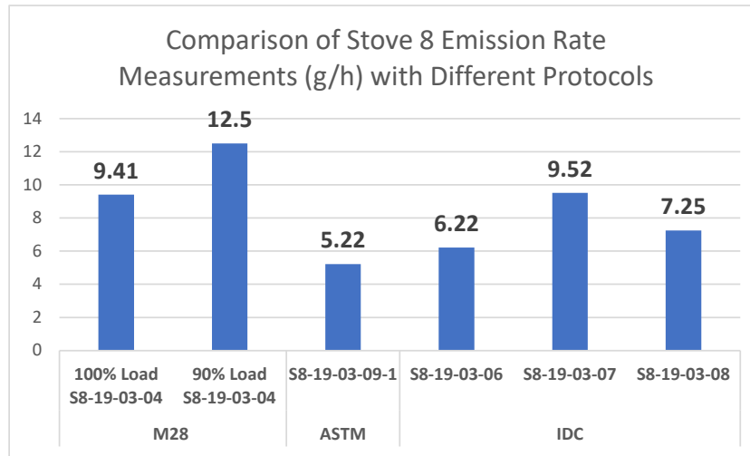
Figure 66. Stove 8—Comparison of Method 28, ASTM 3053-17, and IDC Final Protocol Emissions Rate Measurements (g/h)
