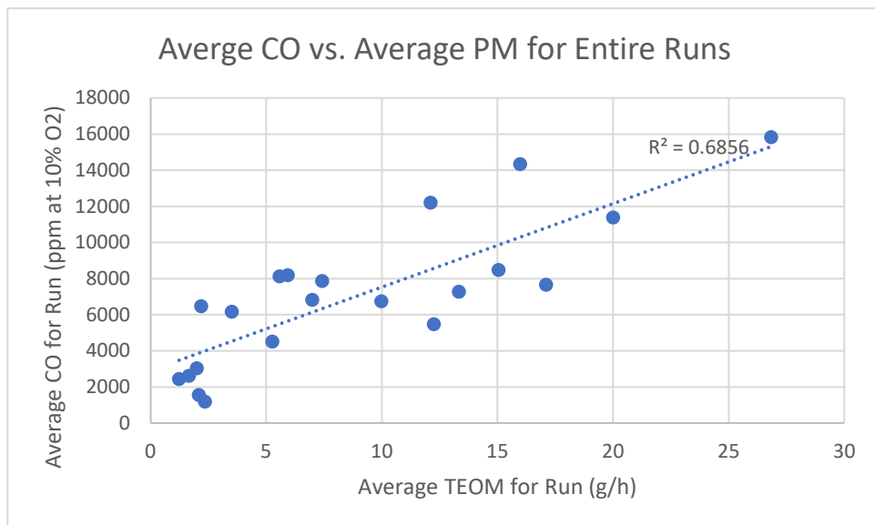
Figure 105. Correlation Average CO and PM Measurements for Entire Runs
