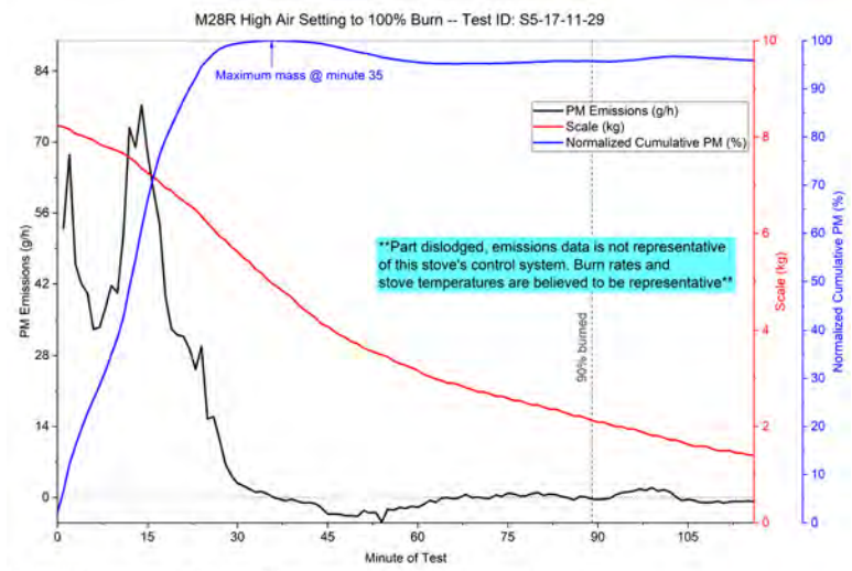
Figure 25. Stove 5—M28 Baseline Test Results
