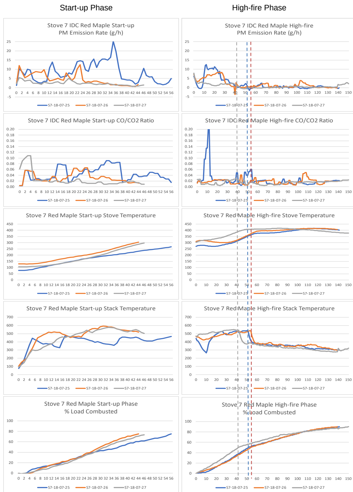
Figure 125. Stove 7—IDC Start-Up and High-Fire Phase Red Maple Profiles
