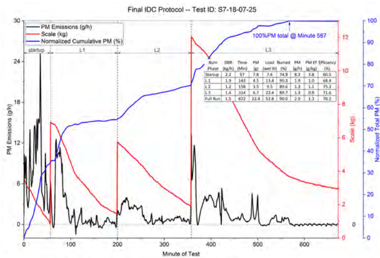
Figure 51. Stove 7—IDC Final Protocol Replicate Runs with Red Maple Cordwood
