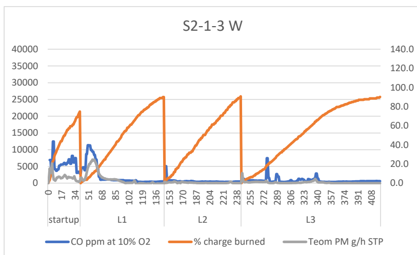
Stove 2: Runs with Door Initially Wide Open
