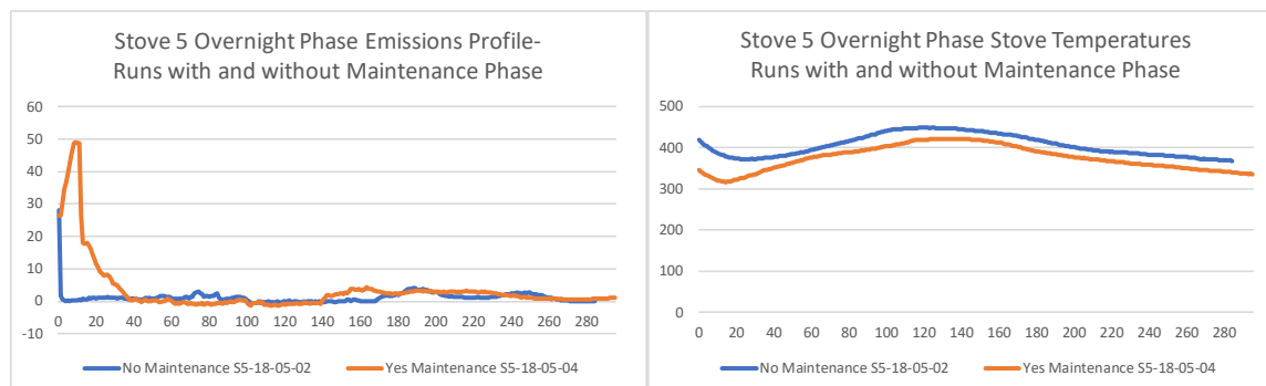
Figure 90. Emissions and Temperature in the Overnight Phase of Stove 5 Runs with and without Maintenance Phases
