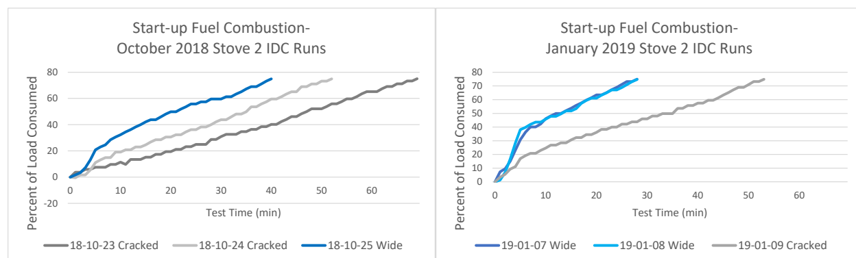
Figure 15. Stove 2—Cumulative Burn Rates—Start-Up Phase of IDC Runs
