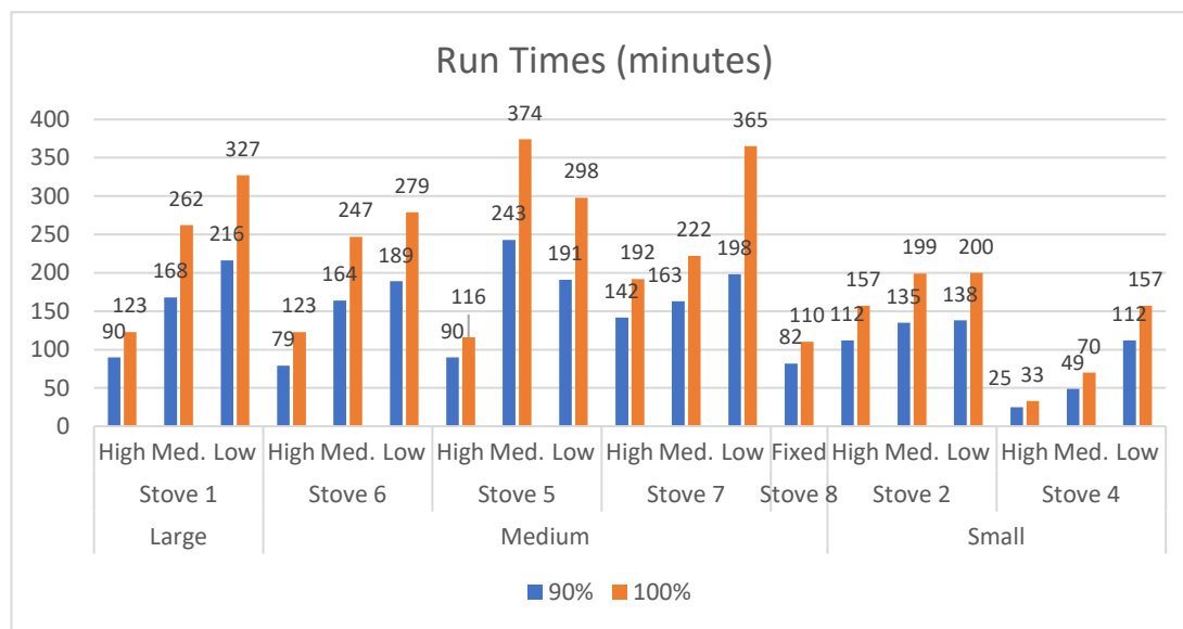
Figure 67. Method 28 Run Times at 90% and 100% Fuel Consumption
