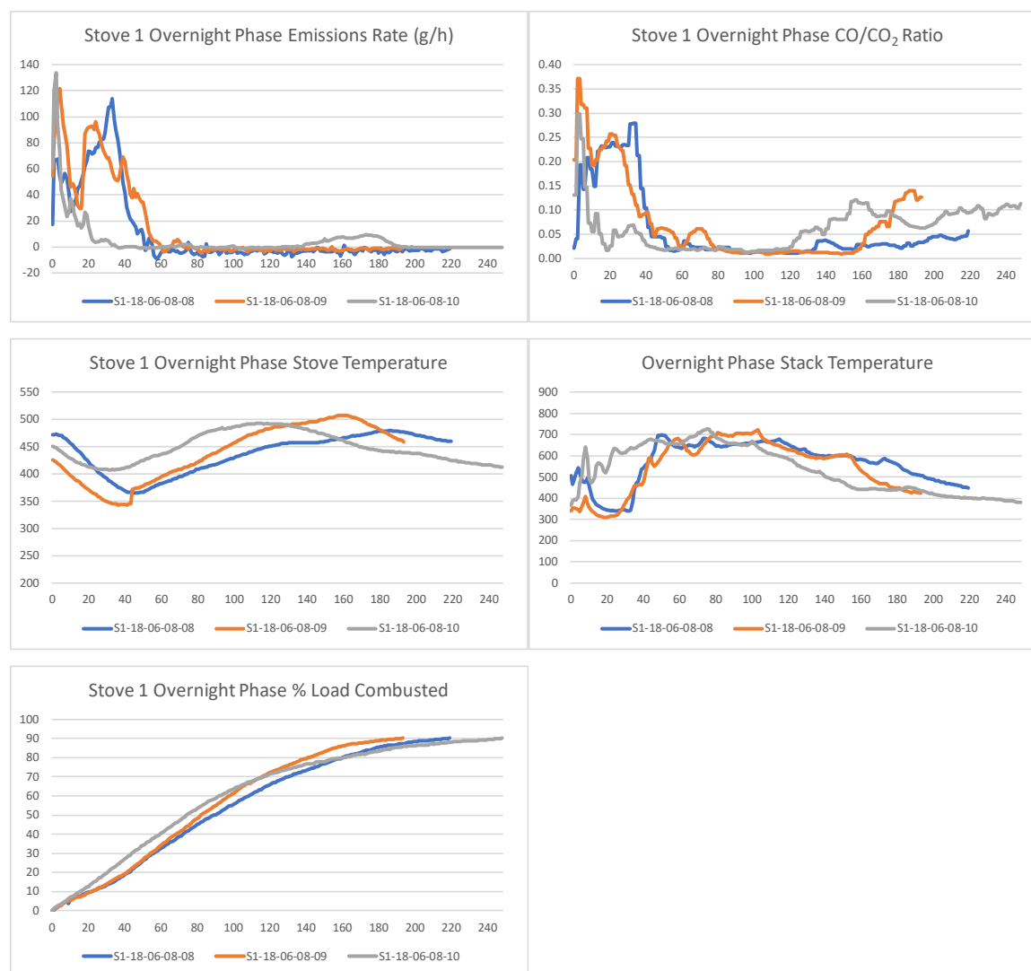
Figure 112. Stove 1 Overnight Phase Profiles
