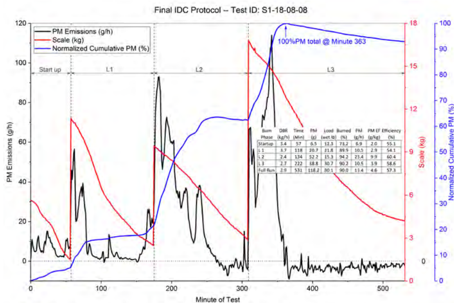
Figure 8. Stove 1—IDC Final Protocol Replicate Runs
