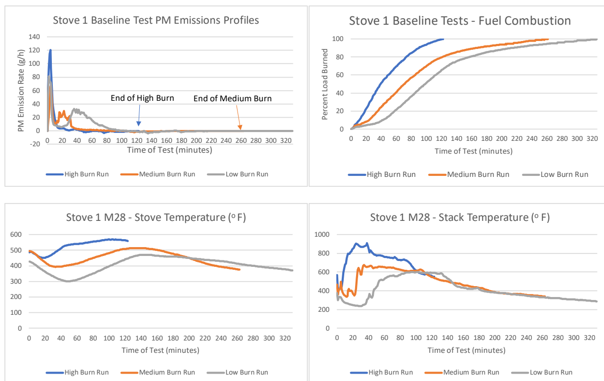
Figure 2. Stove 1—M28 Runs—PM Emission, Cumulative Fuel Consumption, and Stove Temperature Profiles
