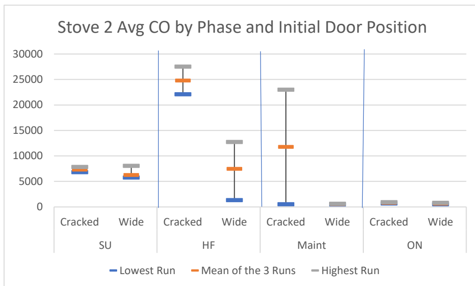
Figure 103. Average Stove 2 CO Concentration (in ppm at 10% O 2 )—by Phase and Initial Door Position
