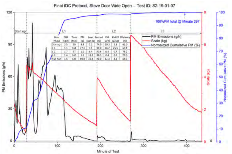
Figure 14. Stove 2—IDC Final Protocol Runs—January 2019
