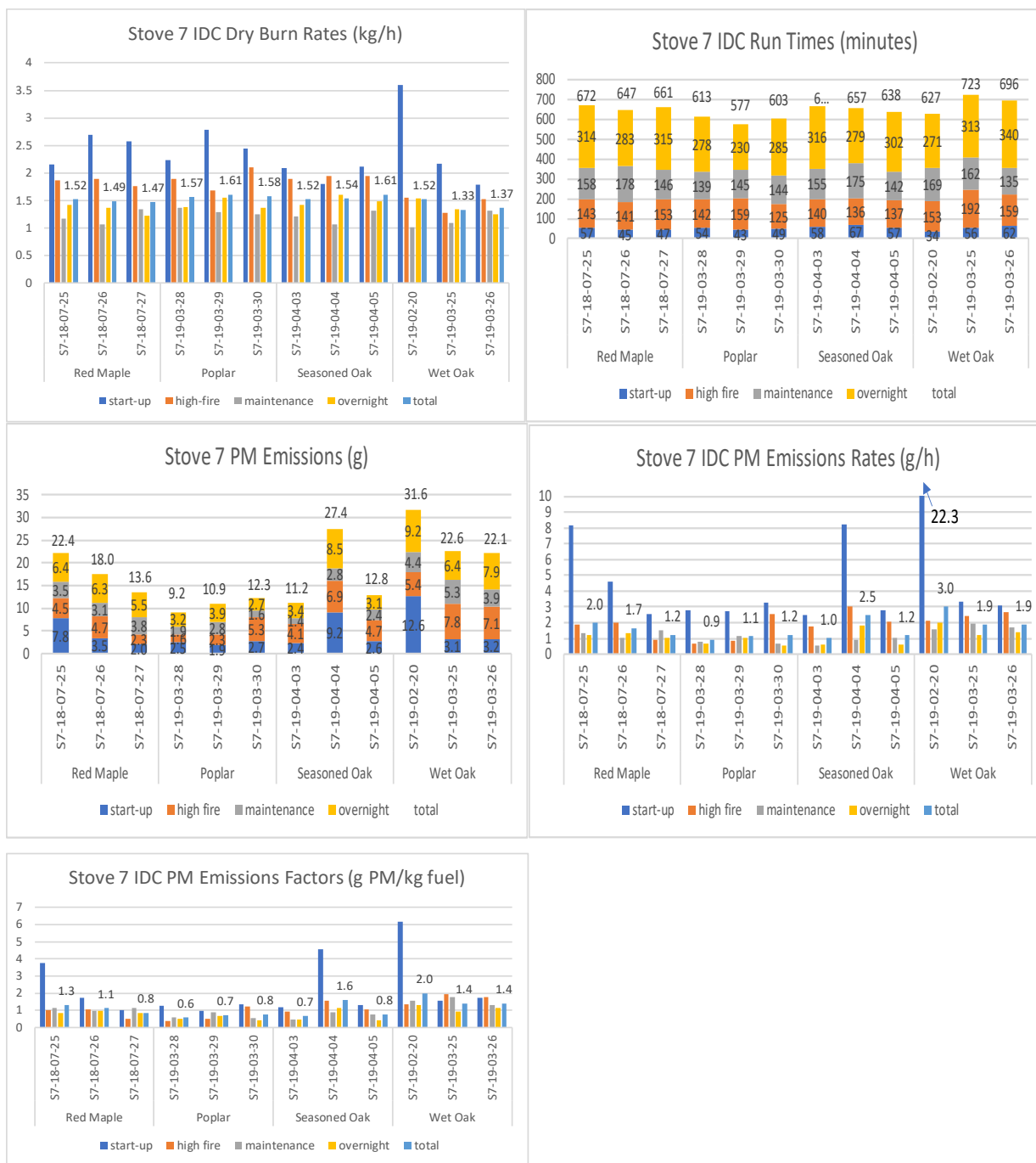
Figure 56. Stove 7—Comparison of Metrics for IDC Replicate Runs
