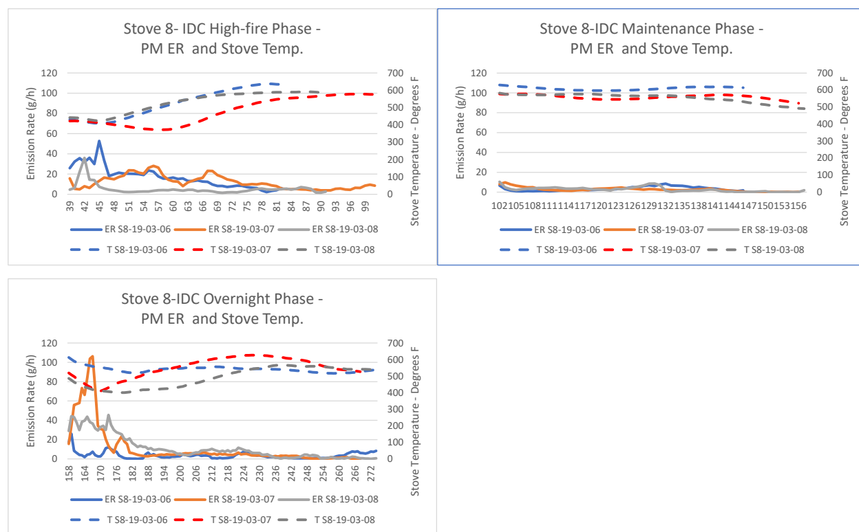
Figure 64. Stove 8—IDC Run Profiles—PM Emissions Rate (g/h) and Stove Temperature (°F)
