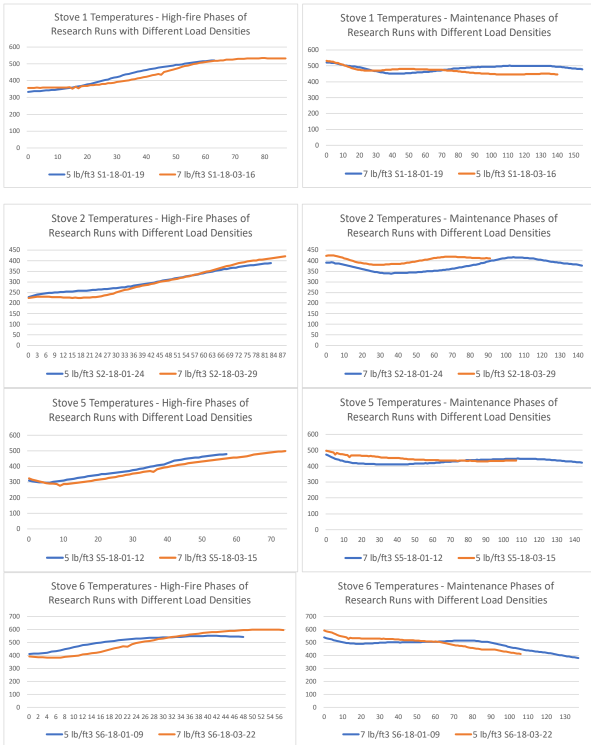
Figure 84. Comparison of High-Fire and Maintenance Phase Temperature Stove Profiles for Paired Runs with Different Load Densities
