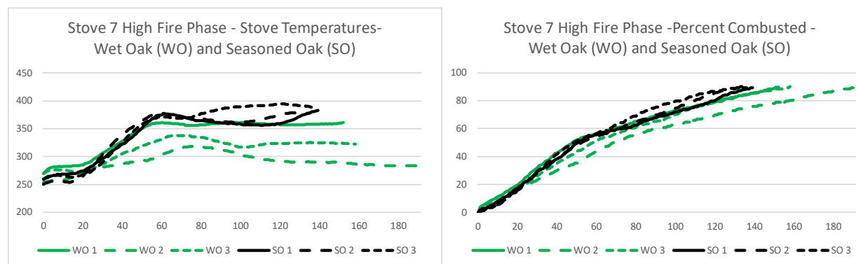
Figure 97. Stove 7 IDC High-Fire Phase—Seasoned and Wet Oak—Stove Temperatures and Fuel Consumption
