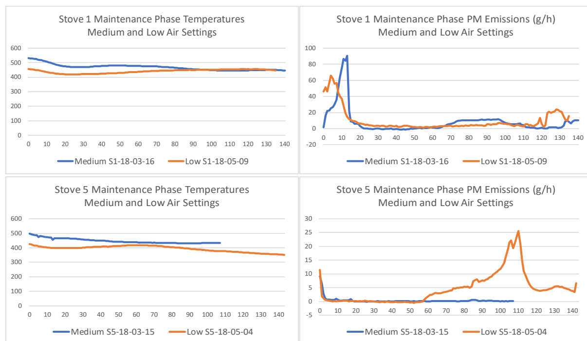
Figure 89. Temperature and Emissions Profiles for Medium- and Low-Maintenance Phases
