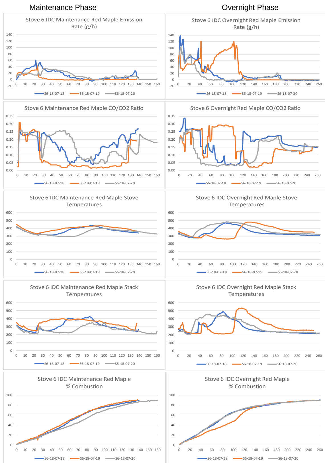
Figure 123. Stove 6—IDC Maintenance and Overnight Phase Red Maple Profiles
