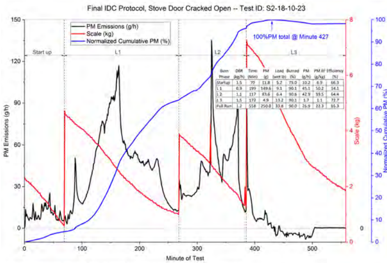
Figure 80. Stove 2—IDC Final Protocol Runs—October 2018
