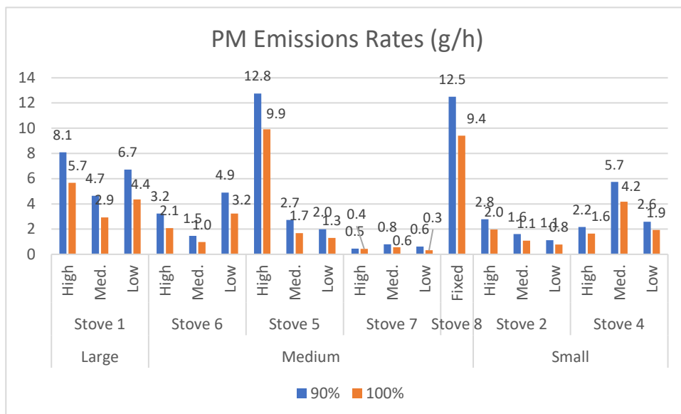
Figure 76. PM Emission Rates for 90% and 100% Combustion in M28 and ASTM 3053-17 Runs
