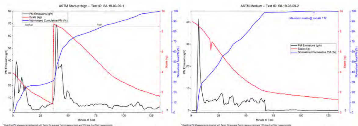
Figure 61. Stove 8—ASTM 3053-17 Runs
