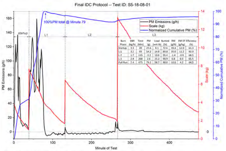
Figure 27. Stove 5 – IDC Final Protocol Runs
