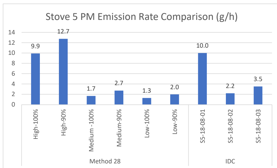
Figure 31. Stove 5—Comparison of Method 28 and IDC Emission Rate Measurements (g/h)
