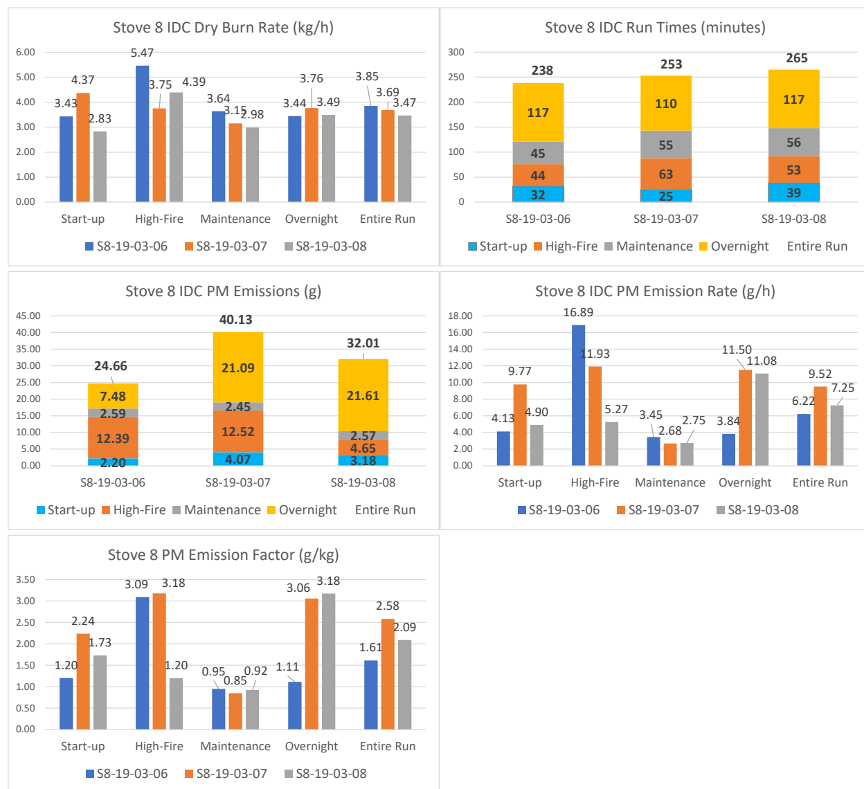
Figure 65. Stove 8—Comparison of Metrics for IDC Replicate Runs
