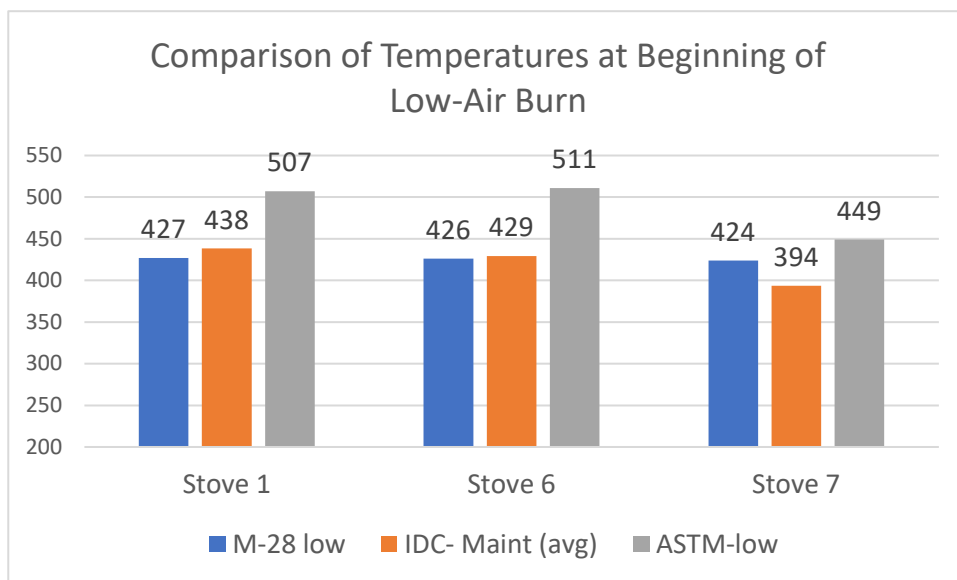
Figure 100. Temperatures (°F) at Beginning of M28, ASTM 3053-17, and IDC Low-Air Phases
