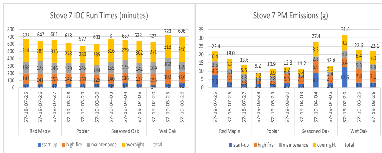
Figure 98. Stove 7 IDC Runs—Run Times and PM Emissions by Phase and Fuel Type
