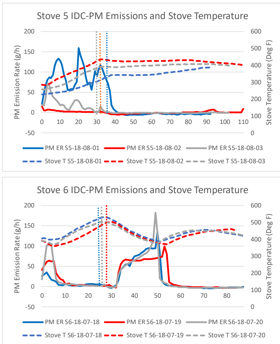
Figure 88. Stoves 5 and 6 High-Fire Phase PM Emissions and Stove Temperature Profiles
