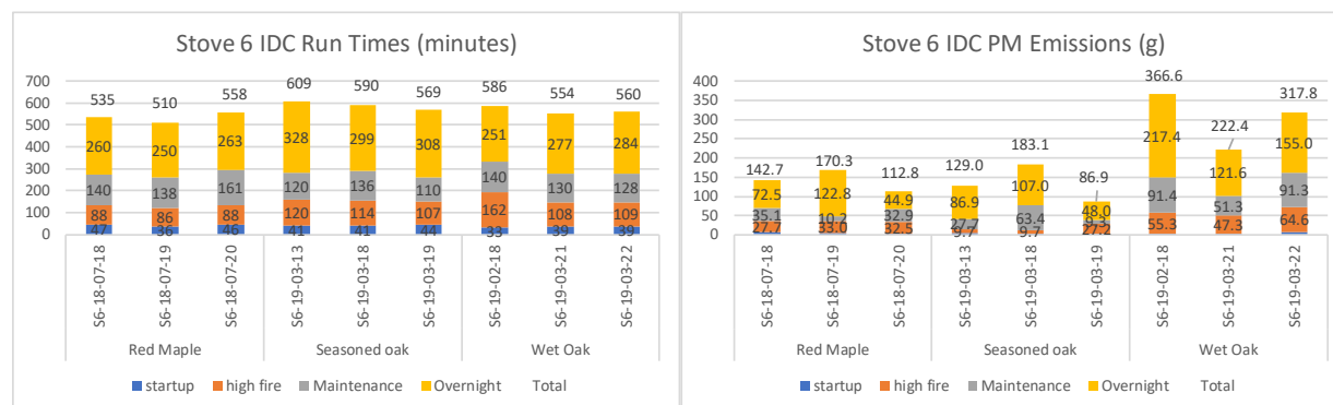
Figure 95. Stove 6 IDC Runs—Run Times and PM Emissions by Phase
