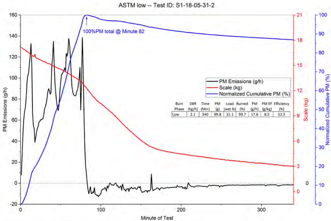
Figure 4. Stove 1—ASTM 3053-17 Low and Medium Loads
