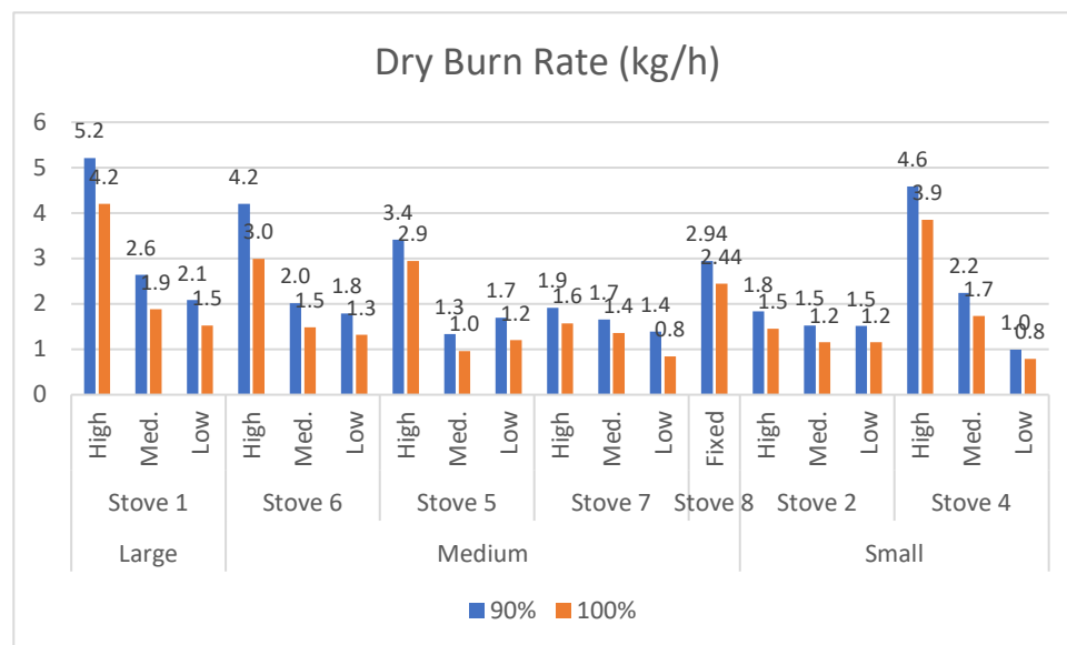
Figure 69. M28 Run Fuel Combustion Rates (kg fuel consumed/hour) at 90% and 100% Fuel Consumption
