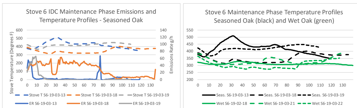
Figure 94. Variability in Stove 6 Seasoned Oak Maintenance Phase Emissions and Temperatures
