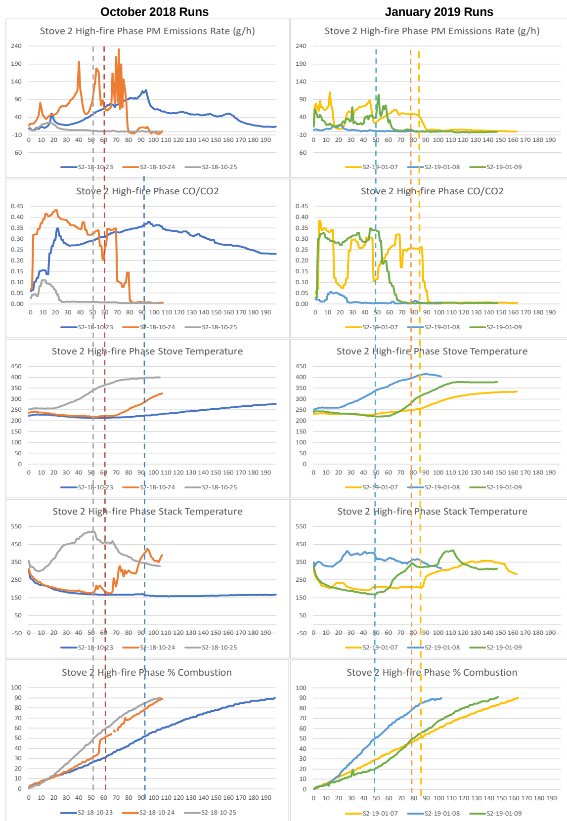
Figure 114. Stove 2 IDC Replicates—High-Fire Phase Profiles
