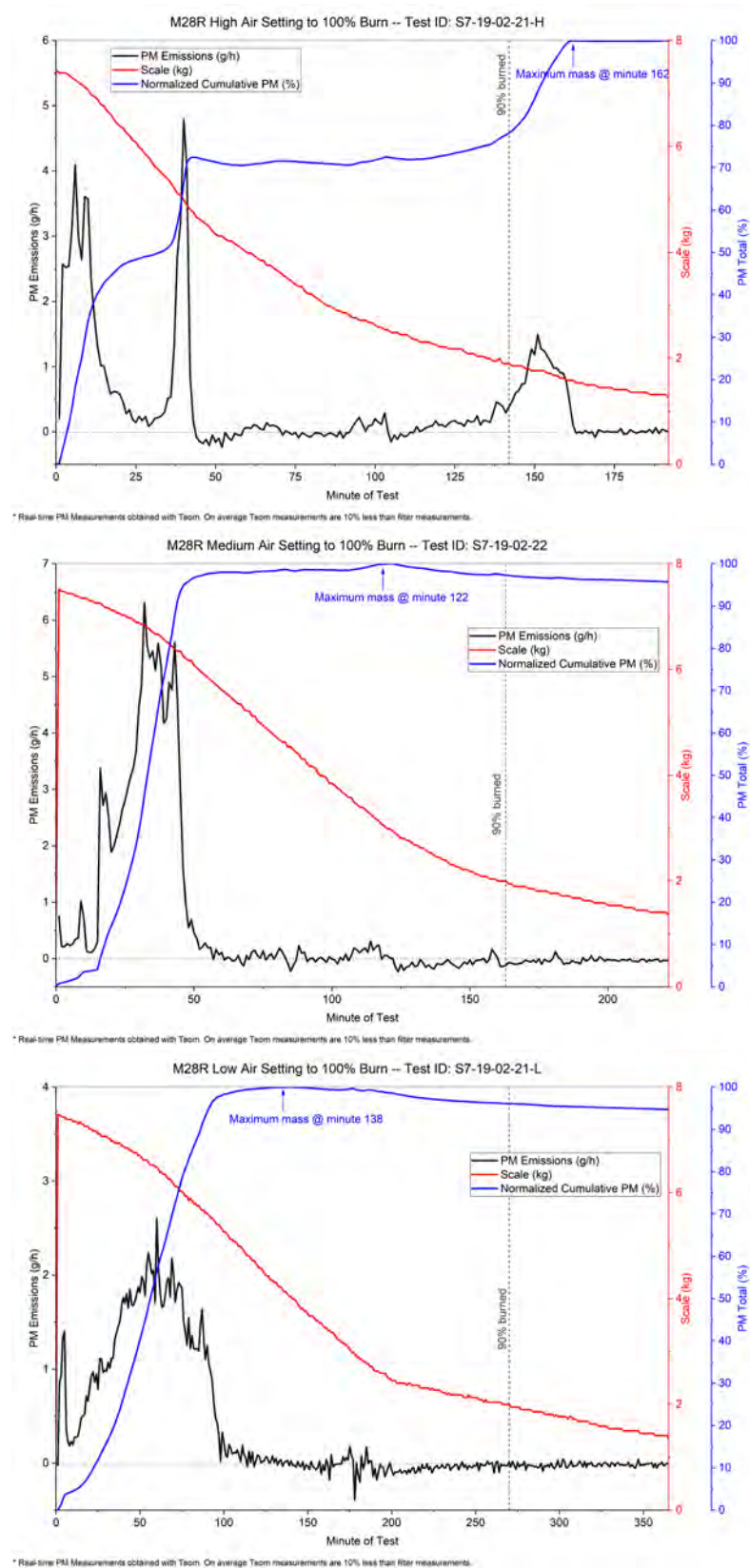
Figure 47. Stove 7—M28 Baseline Test Results
