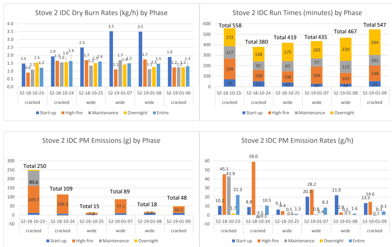
Figure 16. Stove 2—Comparison of Metrics for IDC Runs
