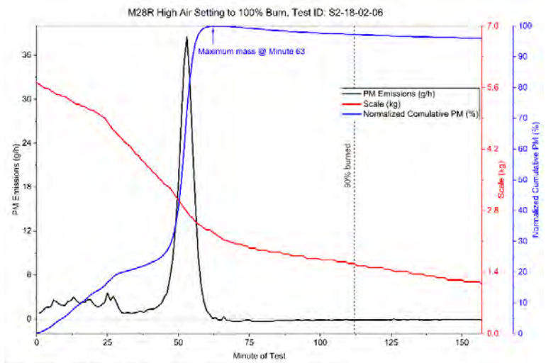
Figure 11. Stove 2—M28 Baseline Test Results
