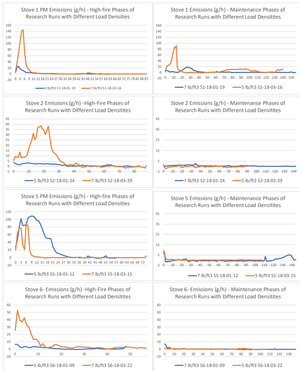
Figure 86. High-Fire and Maintenance Phase PM Emissions—5 lb/ft 3 and 7 lb/ft 3
