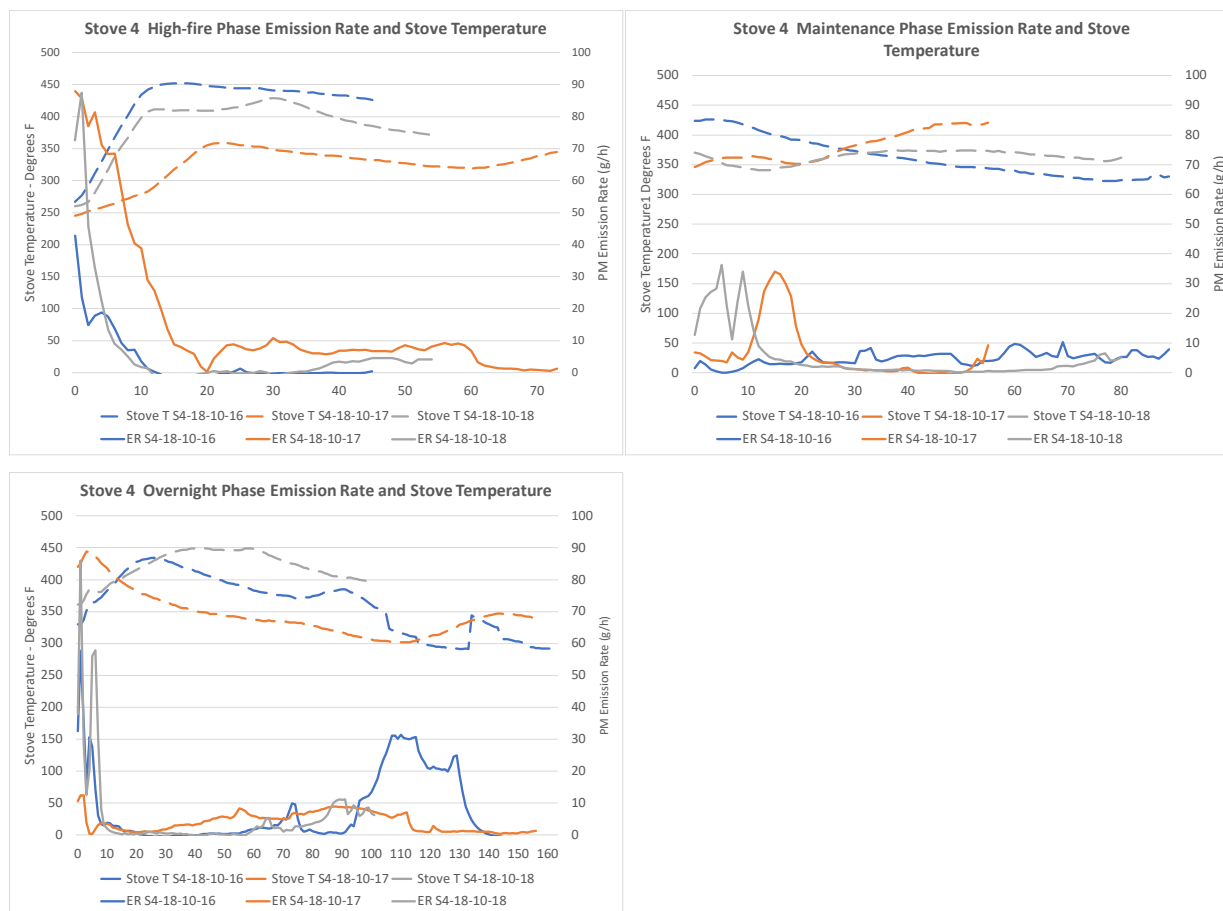
Figure 23. Stove 4—PM Emission Rates and Stove Temperatures
