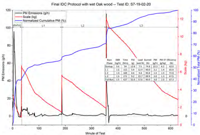
Figure 53. Stove 7—IDC Final Protocol Replicate Runs with Wet Oak Cordwood
