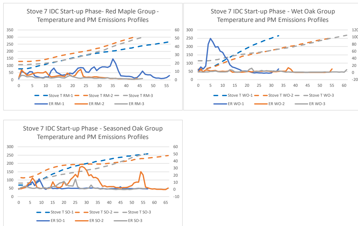
Figure 57. Stove 7—Start-Up Emission and Temperature Profiles
