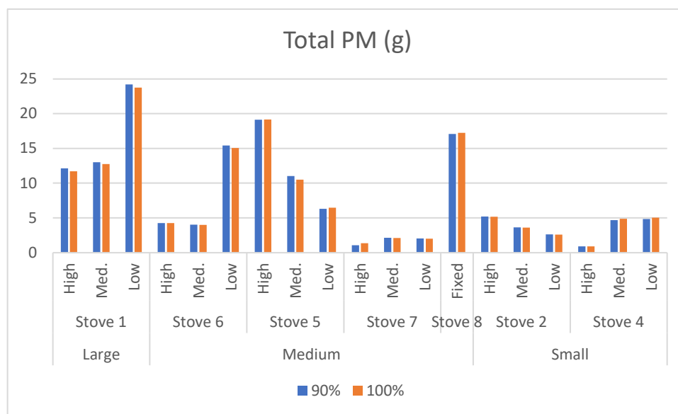
Figure 72. PM Emissions (g) in Method 28 Runs at 90% and 100% Combustion
