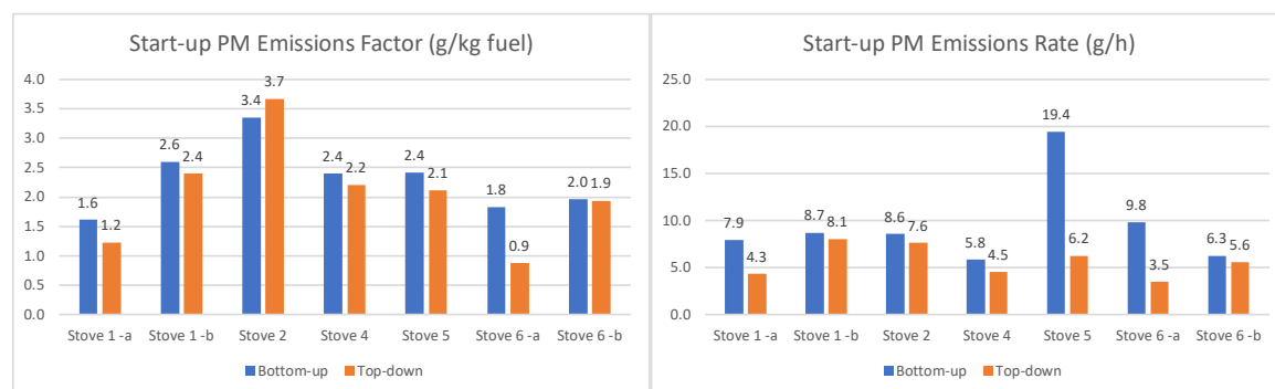
Figure 79. Comparison of Start-Up Bottom-Up and Top-Down PM Emission Parameters
