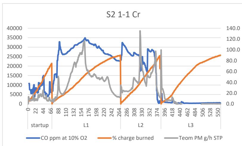
Stove 2: IDC Runs with Door Initially Cracked Open
