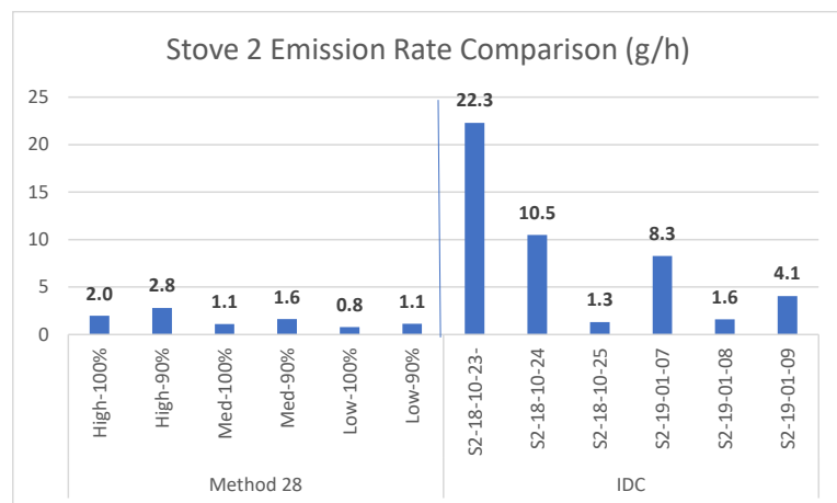
Figure 18. Stove 2—Comparison of Method 28 and IDC Emission Rate Measurements
