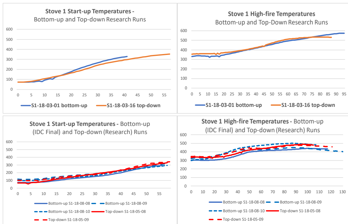
Figure 77. Comparison of Stove Temperature Profiles in Start-Up and High-Fire Phases of Bottom-Up and Top-Down Runs
