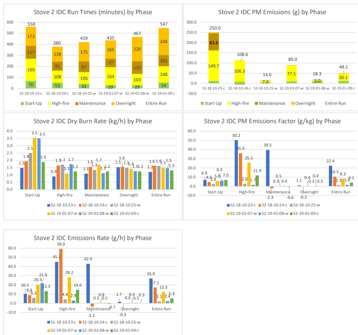
Figure 113. Stove 2—Comparison of Metrics for IDC Runs by Phase
