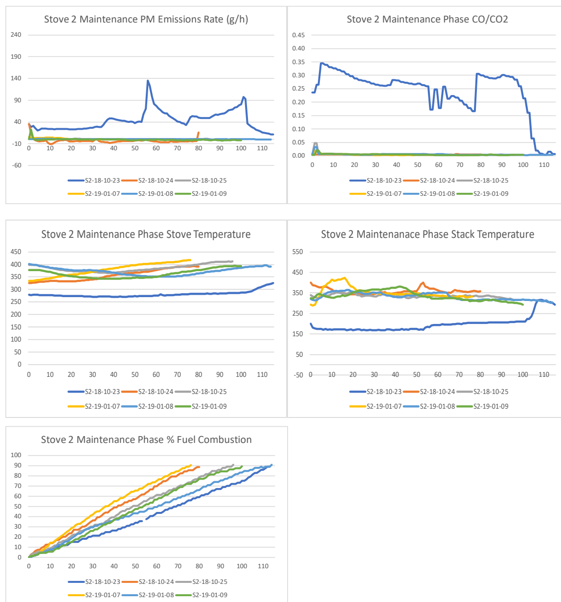
Figure 115. Stove 2 Maintenance Phase Profiles
