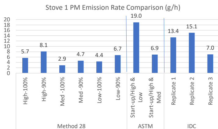
Figure 10. Stove 1—Comparison of M28, ASTM 3053-17, and IDC Emission Rate Measurements
