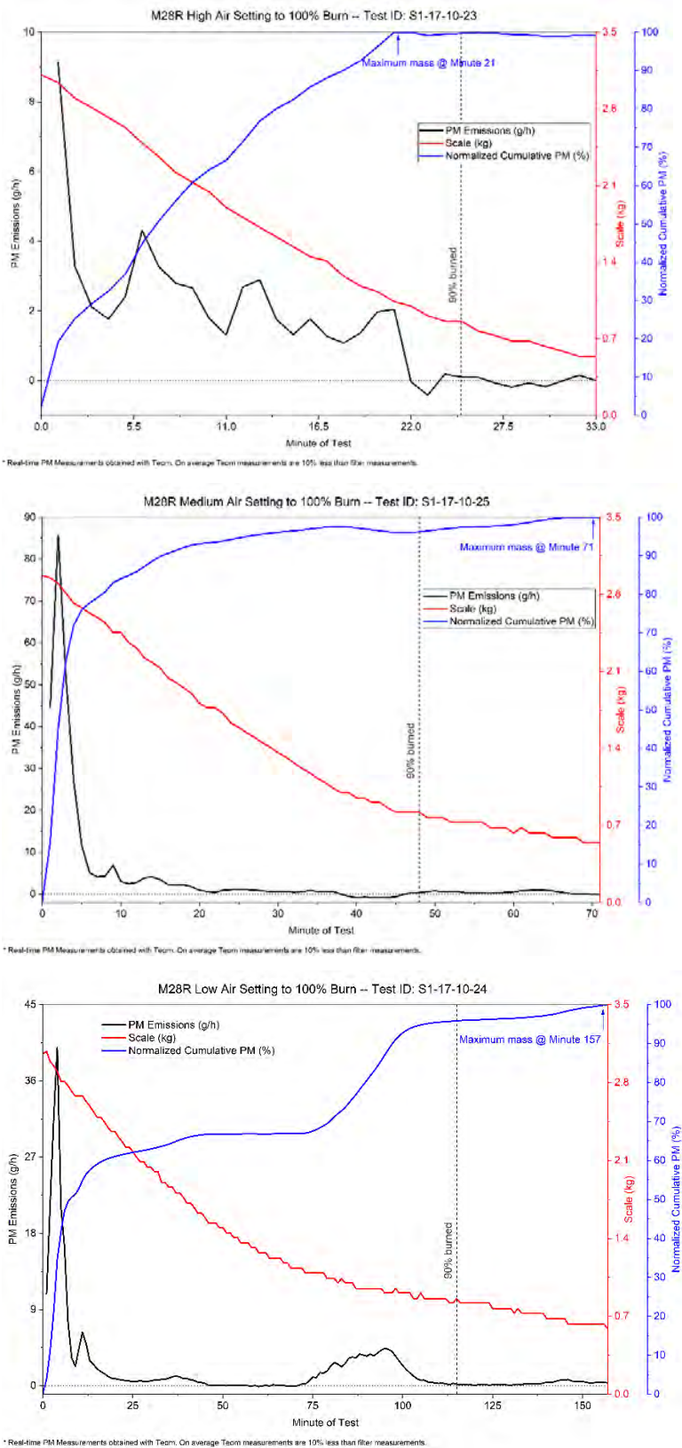
Figure 19. Stove 4—M28 Baseline Test Results
