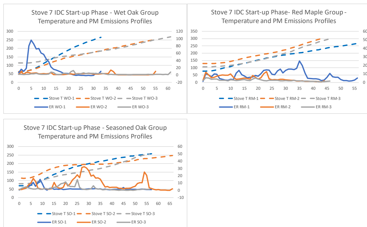
Figure 99. Start-Up Emissions and Temperature Profiles
