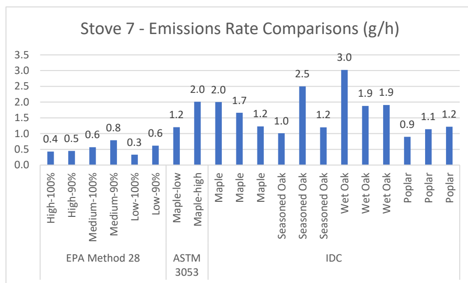
Figure 58. Stove 7—Comparison of Method 28, ASTM 3053-17, and IDC Final Protocol Emissions Rate Measurements (g/h)
