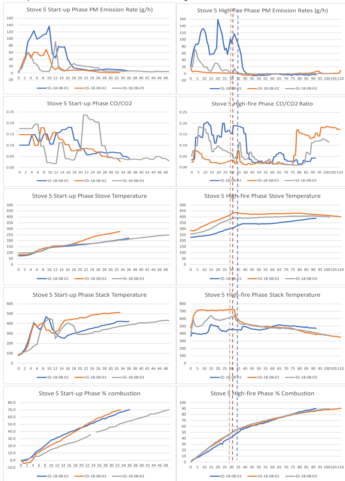
Figure 120. Stove 5 IDC Start-Up and High-Fire Phase Profiles
