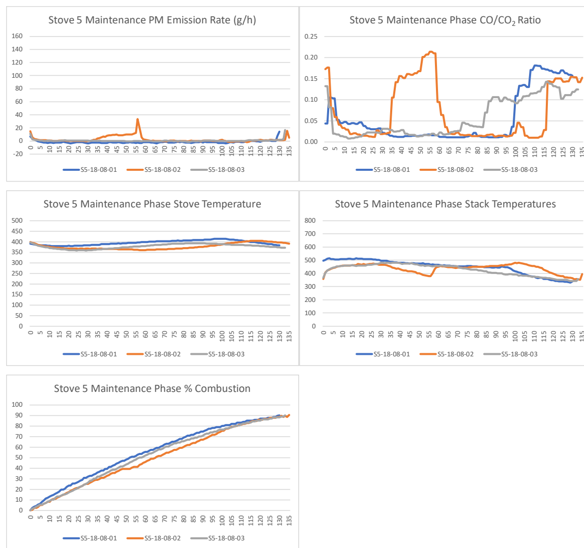
Figure 121. Stove 5 IDC Maintenance Phase Profiles
