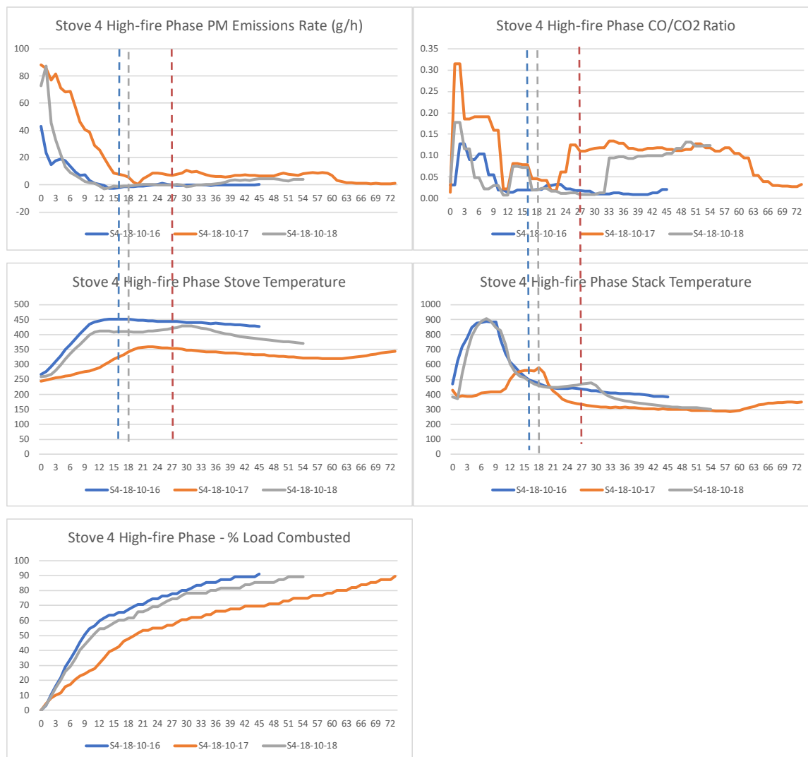
Figure 117. Stove 4 High-Fire Phase Profiles
