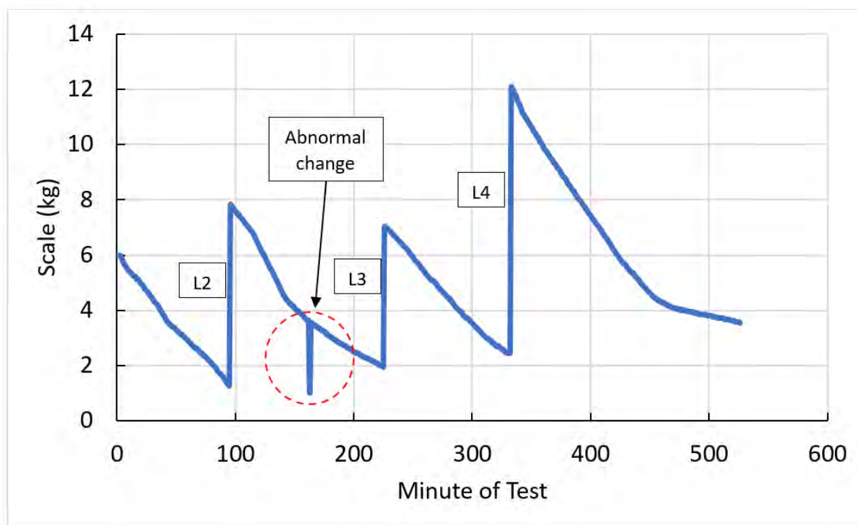
Figure A-9. Normal and Abnormal Changes in Scale Recorded Data
