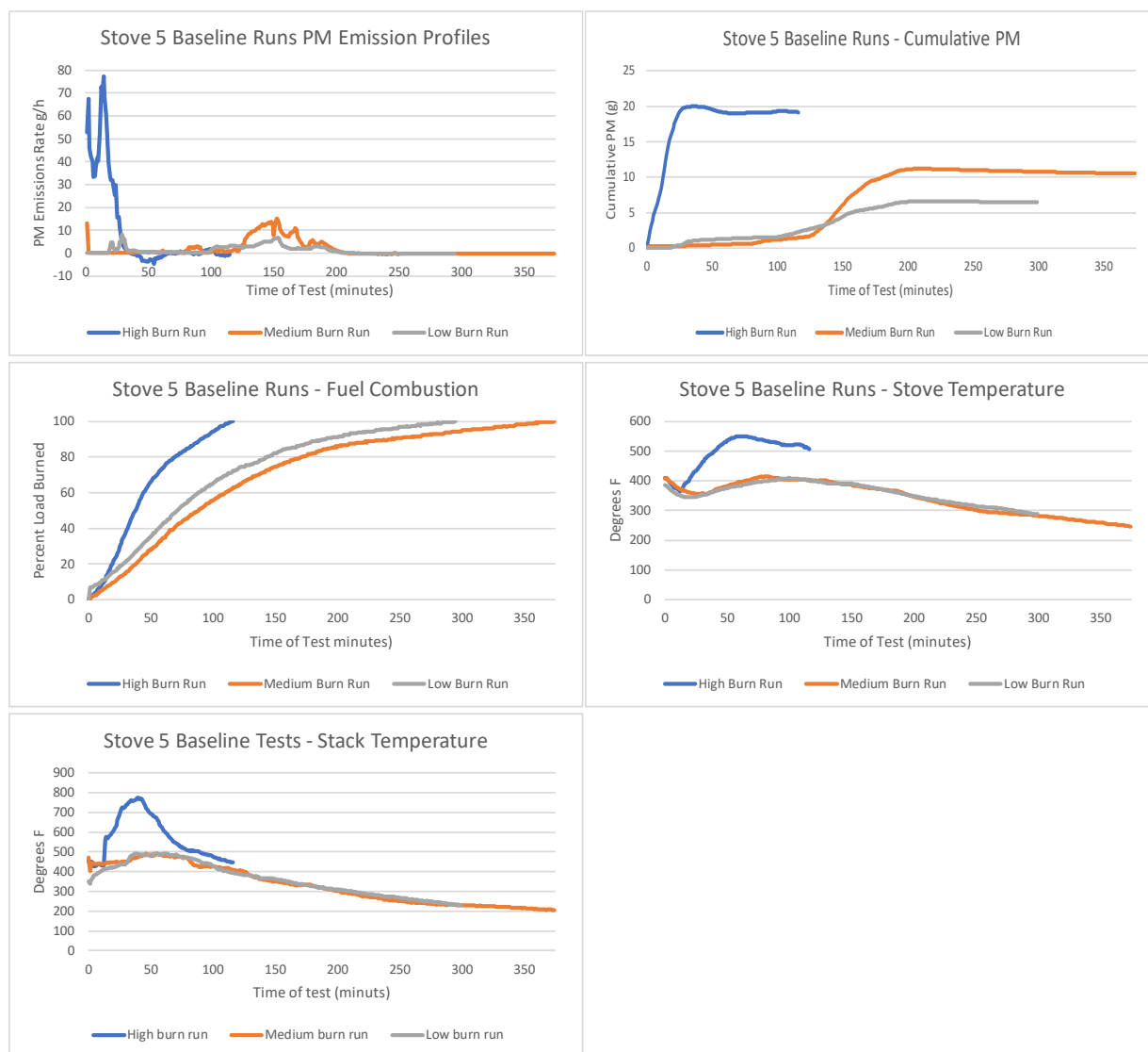
Figure 26. Stove 5—M28 Baseline Runs—PM Emission Profiles, Cumulative PM Emissions, Cumulative Fuel Consumption, and Stack Temperatures
