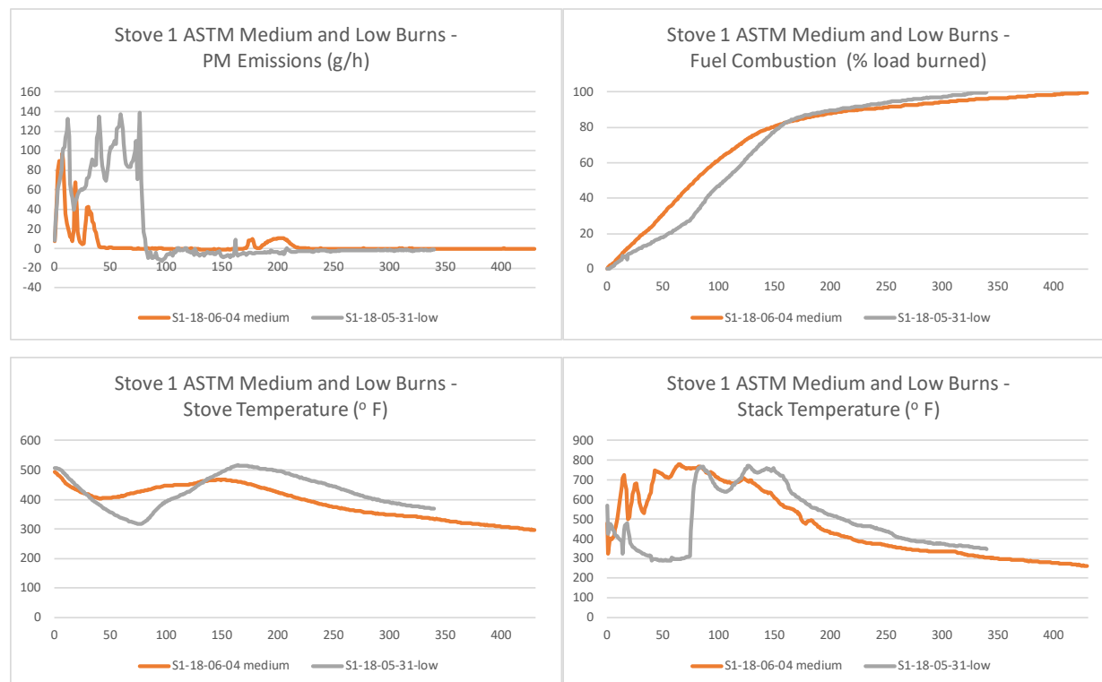
Figure 6. Stove 1—ASTM 3053-17 Medium and Low Phases—PM Emission, Cumulative Fuel Consumption and Stove Temperature Profiles
