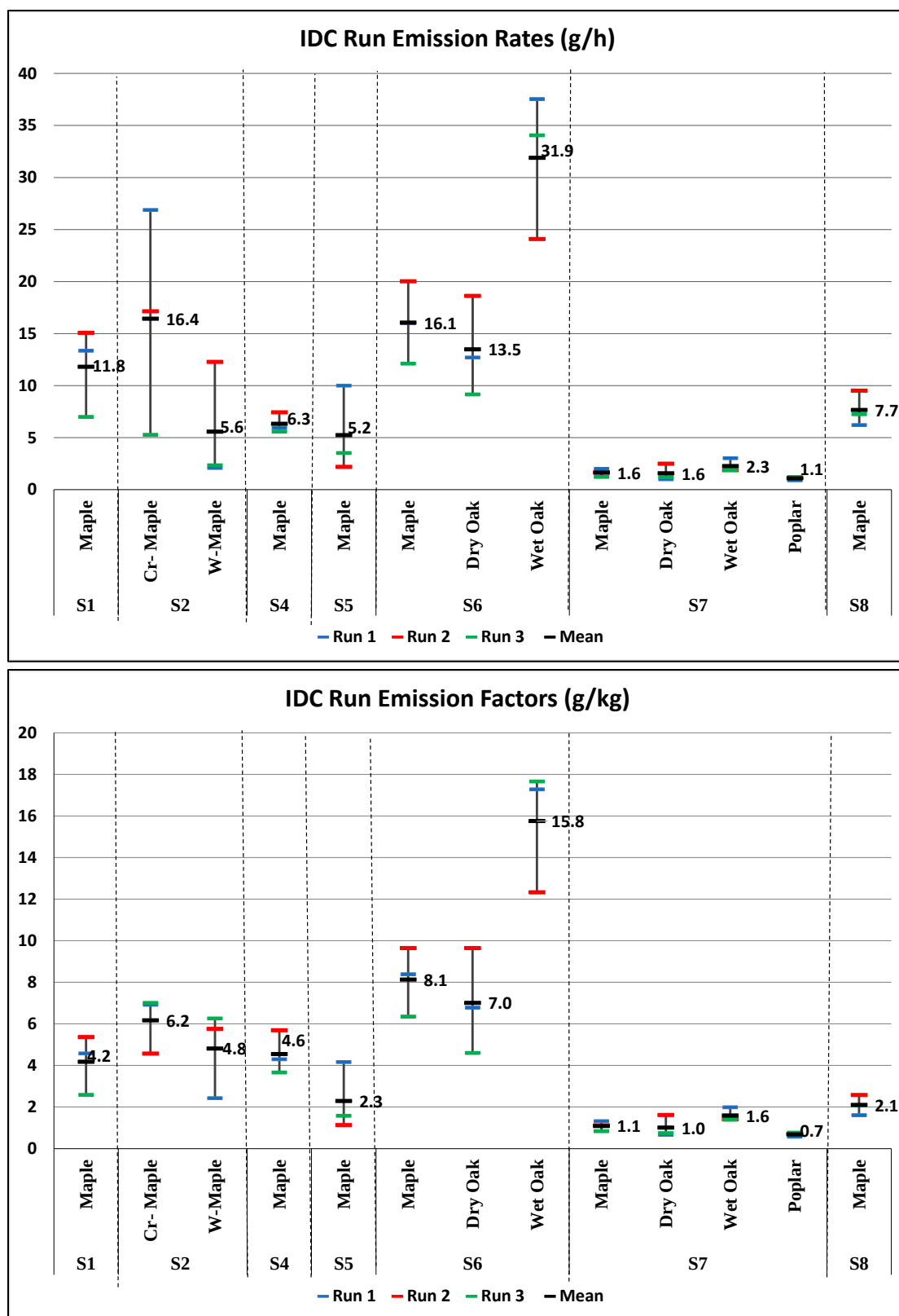
Figure 128. IDC Run Emission Rates (g/h) and Emission Factors (g/kg) by Stove and Fuel
