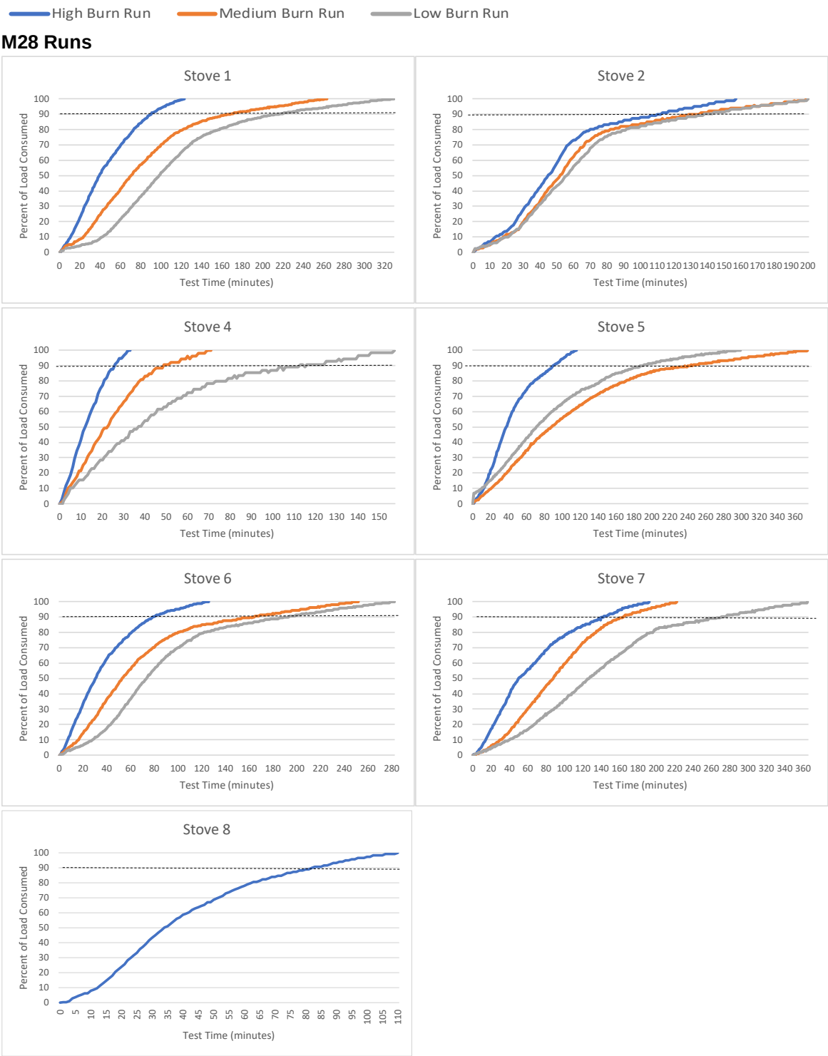
Figure 71. Burn Profiles (Percent of Fuel Consumed)
