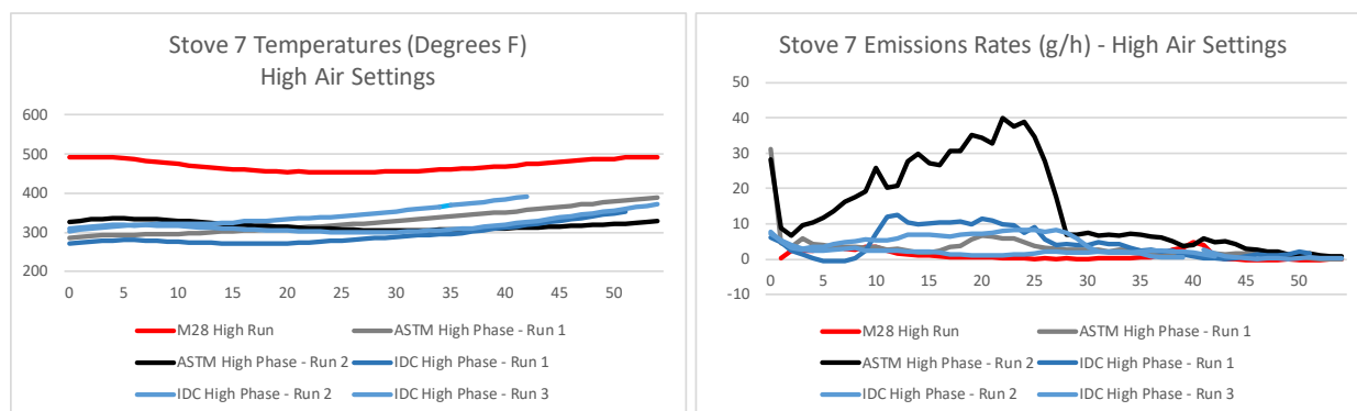
Figure 59. Stove 7—Comparison of Temperature Profiles and Emission Rates in Burns at High-Air Setting
