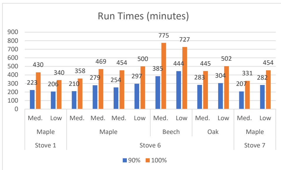
Figure 68. ASTM 3053-17 Low- and Medium-Burn Run Times at 90% and 100% Fuel Consumption
