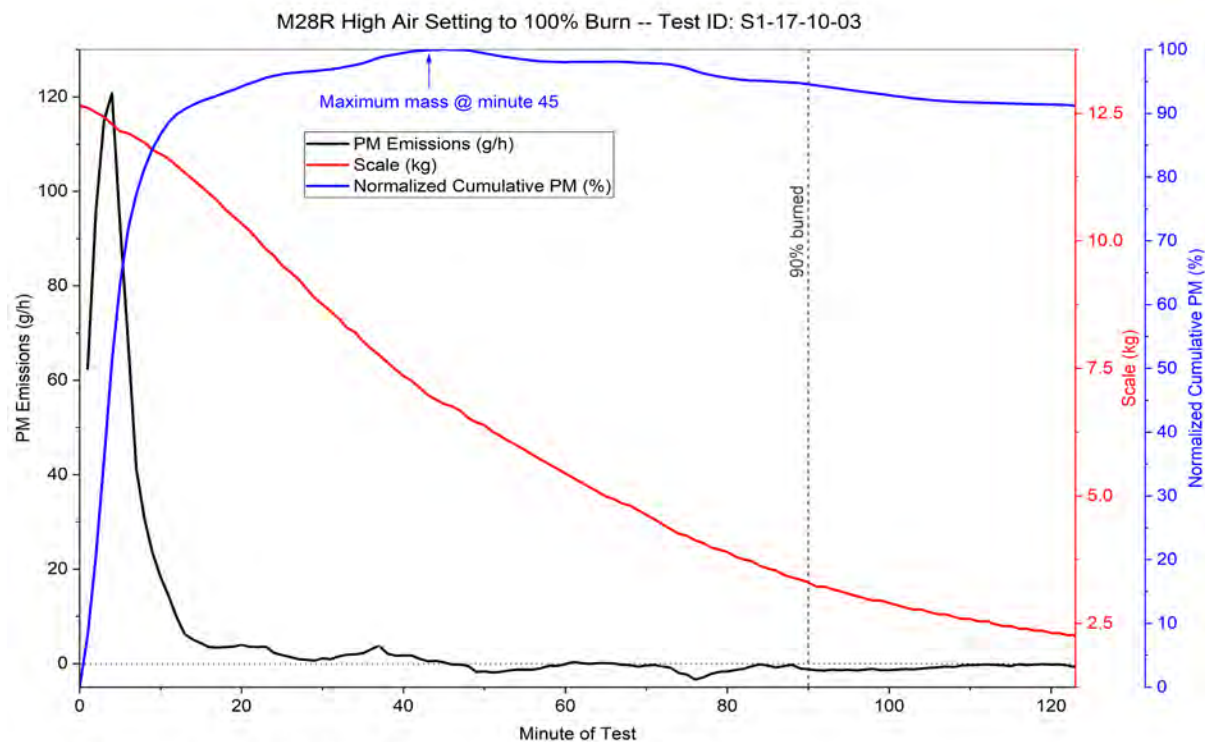
Figure 1. Stove 1—M28 Baseline Test Results
