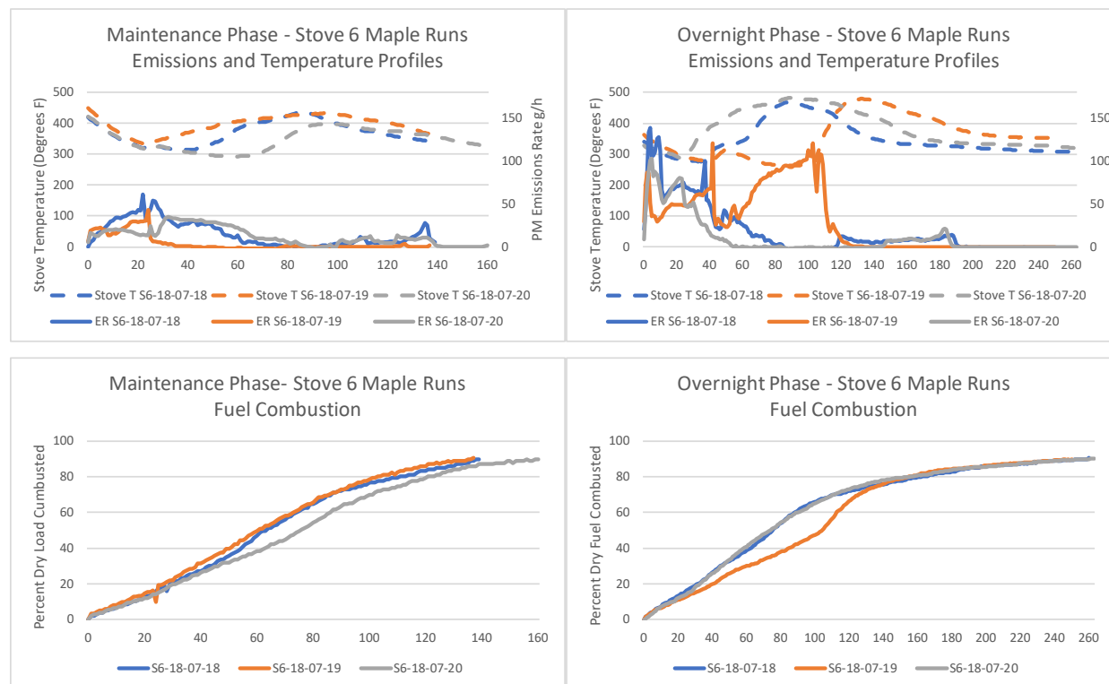
Figure 96. Comparison of Emissions and Temperature Profiles and Fuel Combustion Curves for the Maintenance and Overnight Phases of the Stove 6 Red Maple IDC Runs
