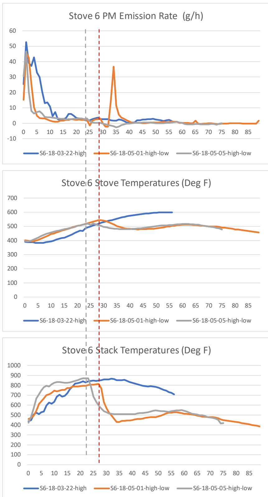
Figure 87. Stove 6 High-Fire Phase—PM Emissions and Stove and Stack Temperature Profiles for Runs with High and High-Low Air Settings
