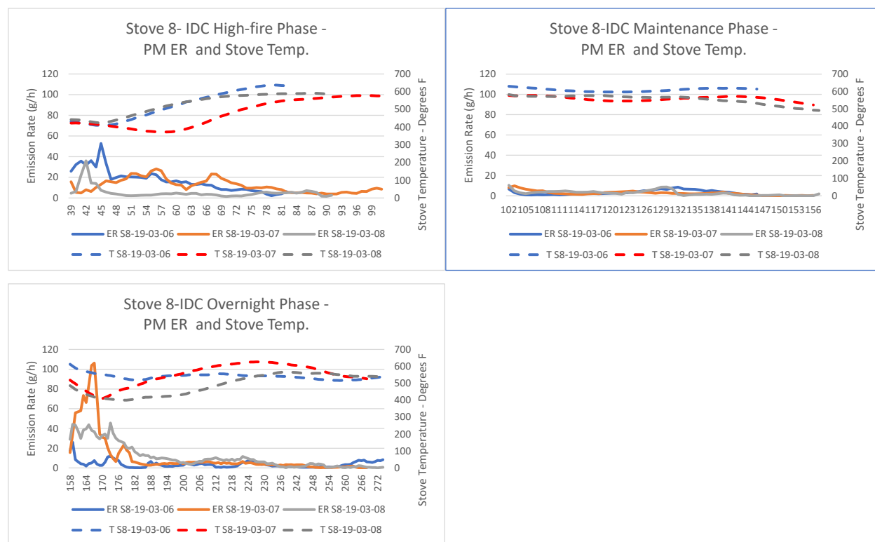
Figure 127. Stove 8—IDC Run Profiles—PM Emissions Rate (g/h) and Stove Temperature (°F)
