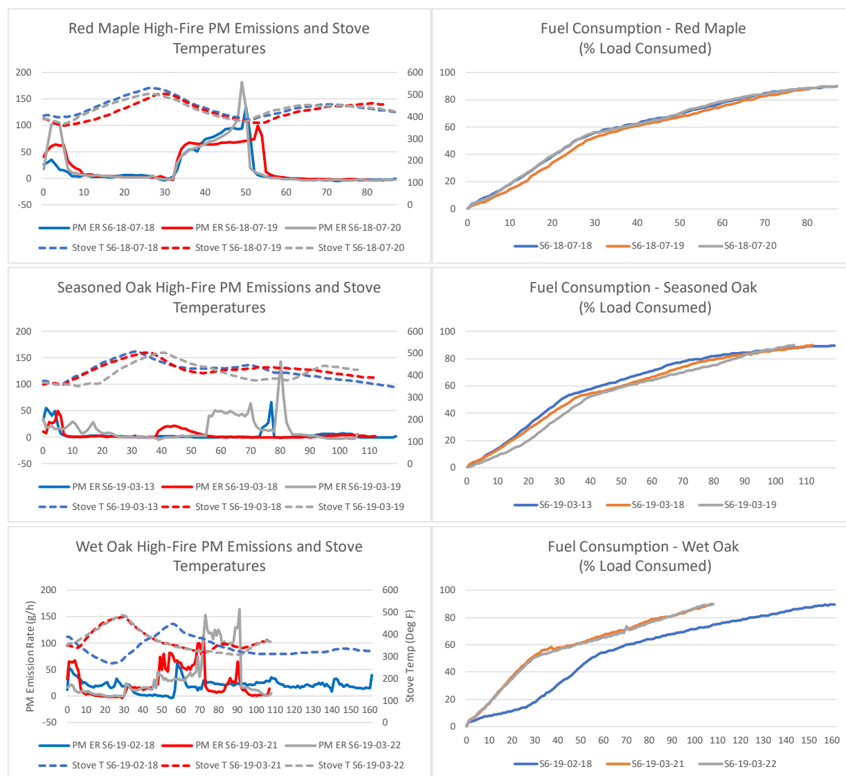
Figure 92. Stove 6 IDC High-Fire Phase Emissions, Stove Temperatures, and Fuel Consumption
