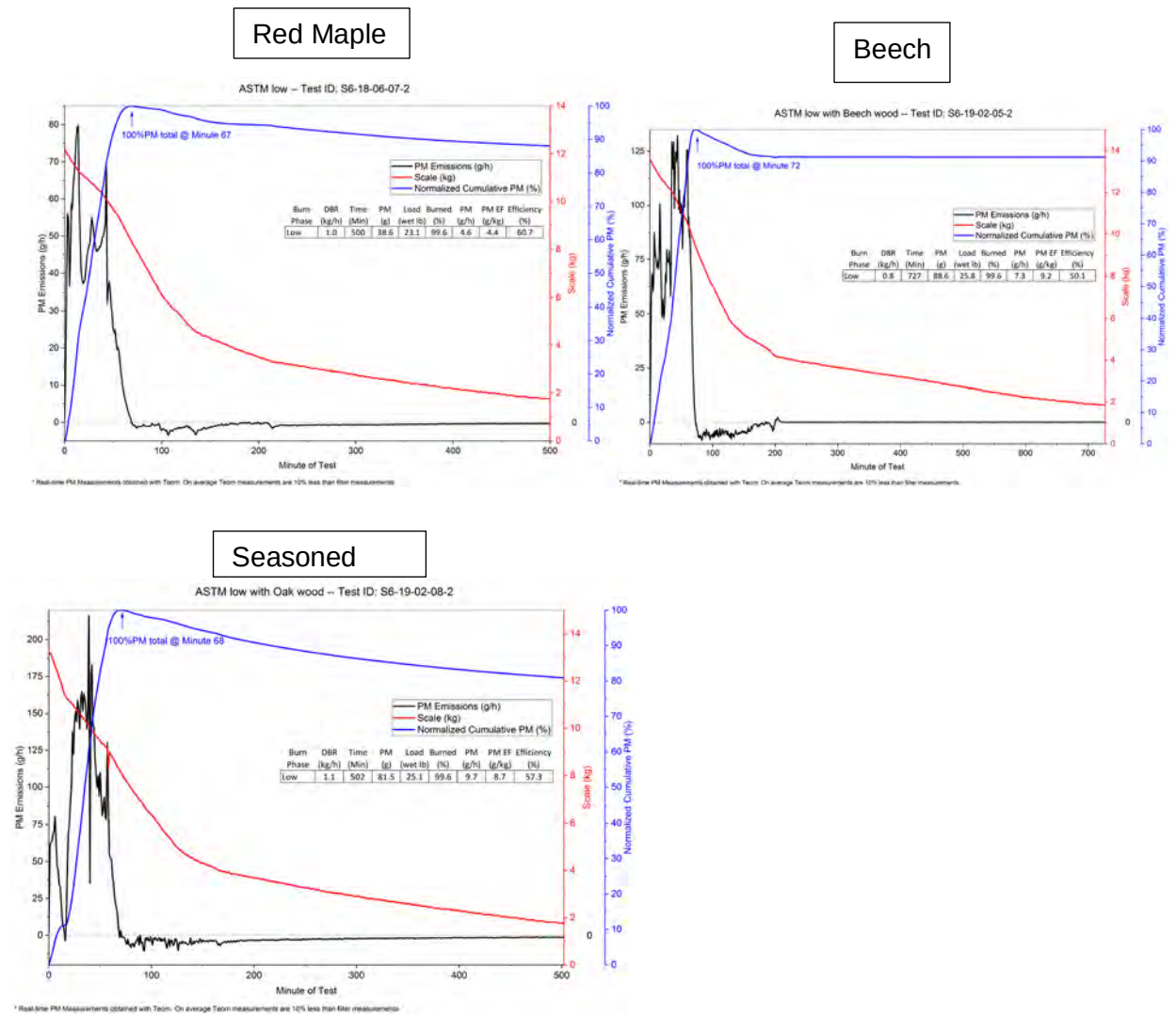
Figure 36. Stove 6—ASTM 3053-17 Runs—Low Fire Phases
