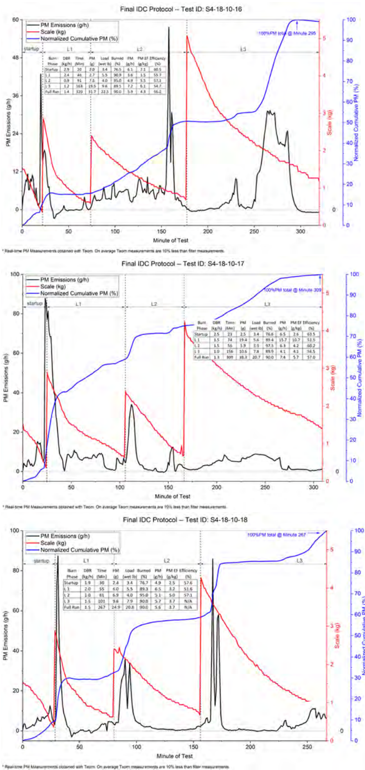
Figure 21. Stove 4—IDC Final Protocol Runs
