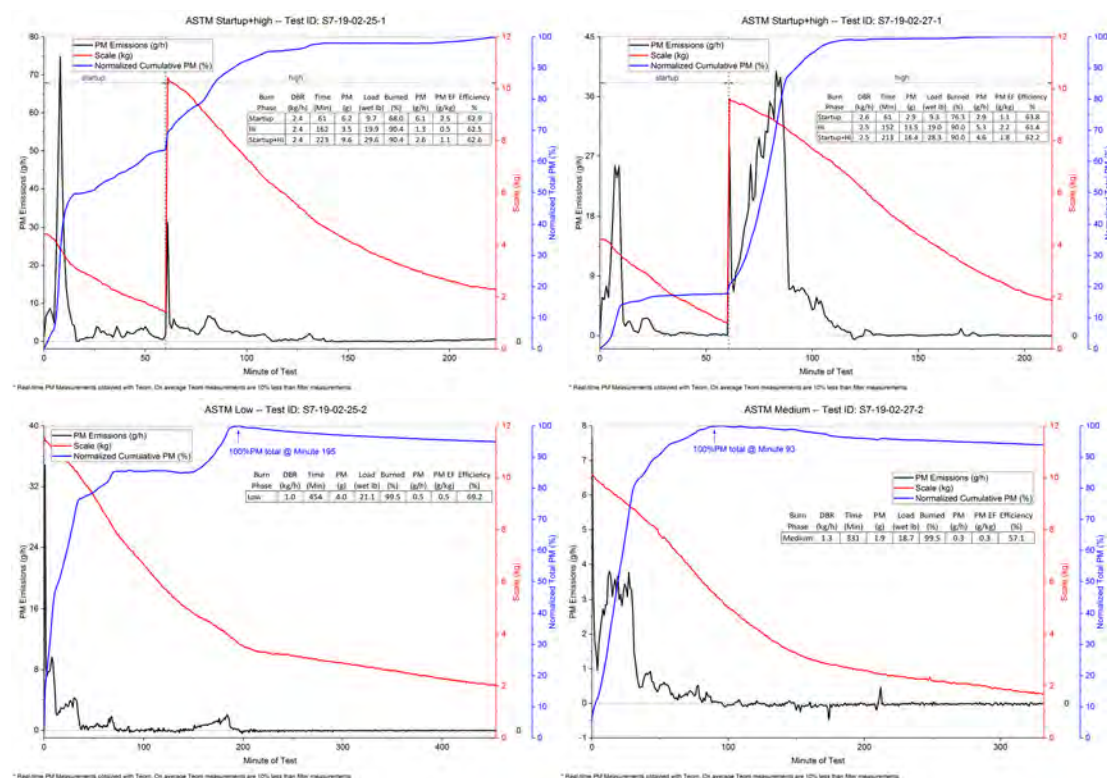
Figure 48. Stove 7—ASTM 3053-17 Runs
