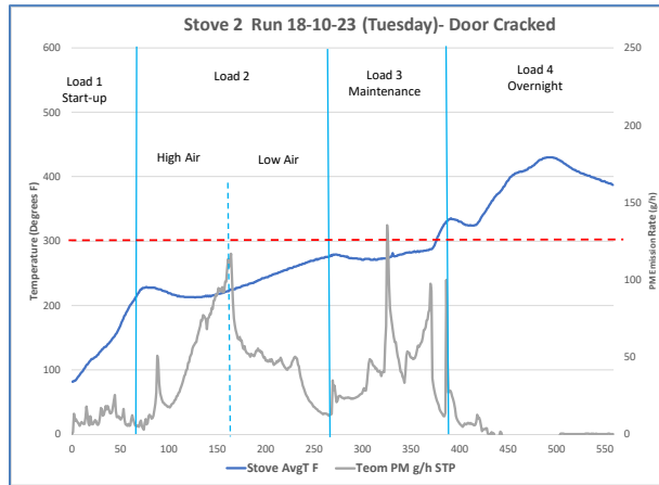
Stove 2—October 2018 IDC Runs
