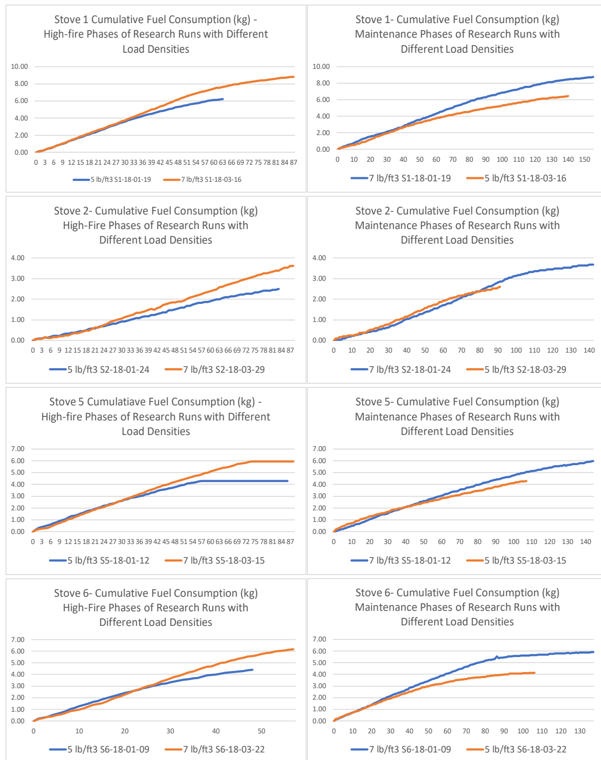
Figure 85. High-Fire and Maintenance Phase Cumulative Fuel Consumption in Runs with Different Load Densities
