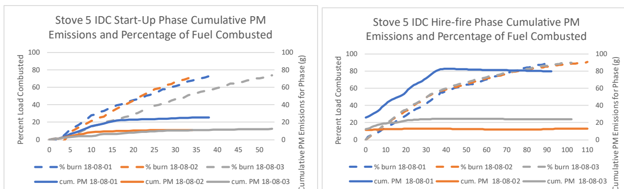
Figure 30. Stove 5—IDC Runs—Cumulative PM Emissions and Percentage of Load Combusted in Start-Up and High-Fire Phases
