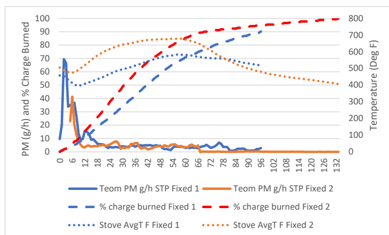
Figure 62. Stove 8—ASTM 3053-17 Emissions, Stove Temperatures, and Fuel Combustion
