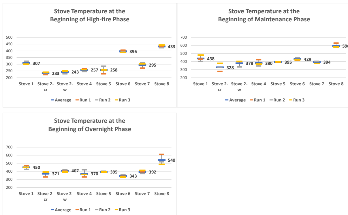
Figure 108. Stove Temperatures (°F)—Hgh-Fire, Maintenance, and Overnight Phases
