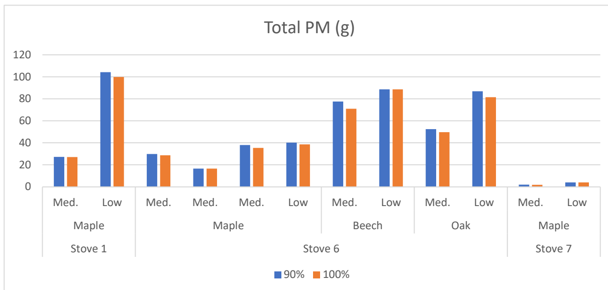
Figure 73. PM Emissions (g) in ASTM 3053-17 Low and Medium Runs at 90% and 100% Combustion
