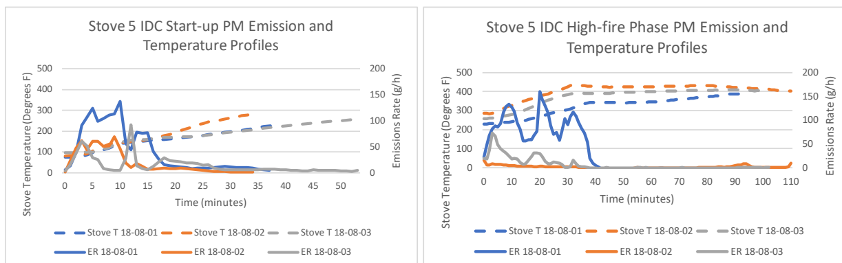
Figure 29. Stove 5—IDC Runs—PM Emission and Stove Temperature Profiles for Start-Up and High-Fire Phases
