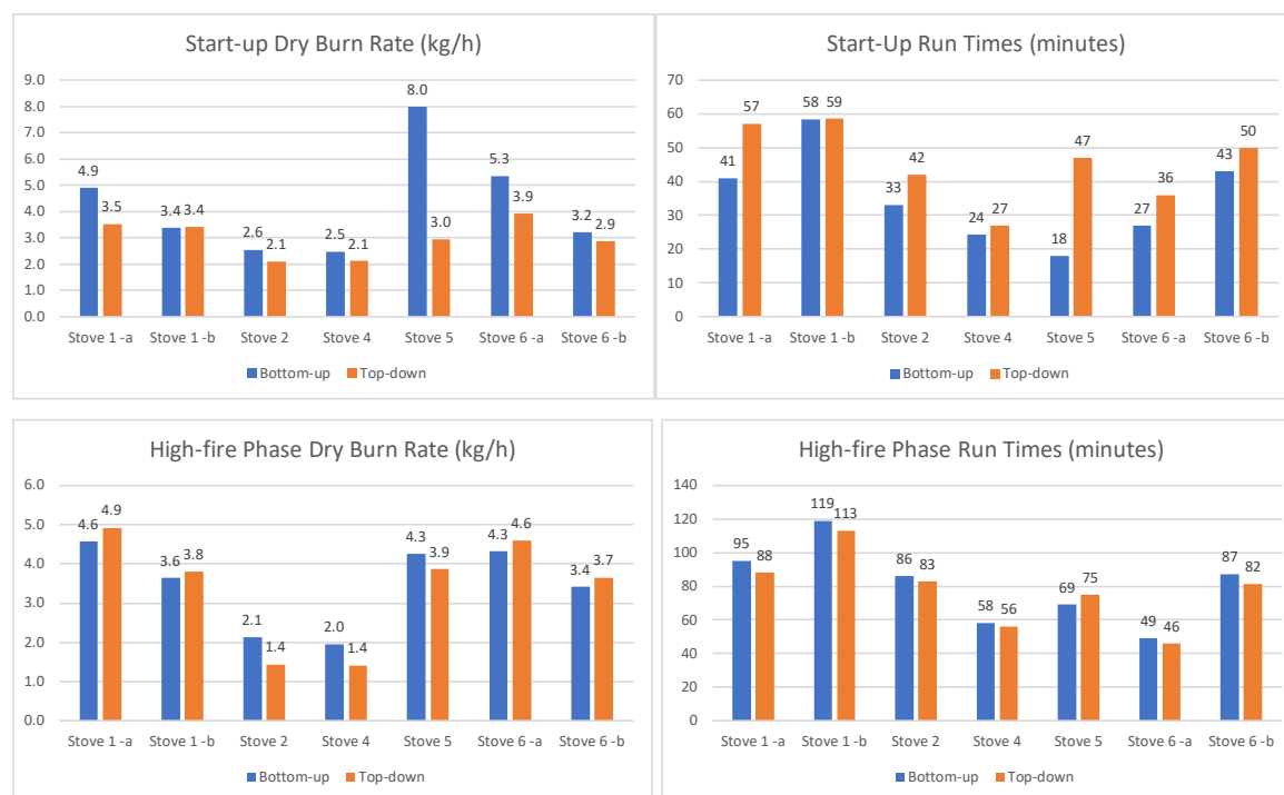
Figure 78. Comparison of Start-Up and High-Fire Bottom-Up and Top-Down Burn Parameters 6
