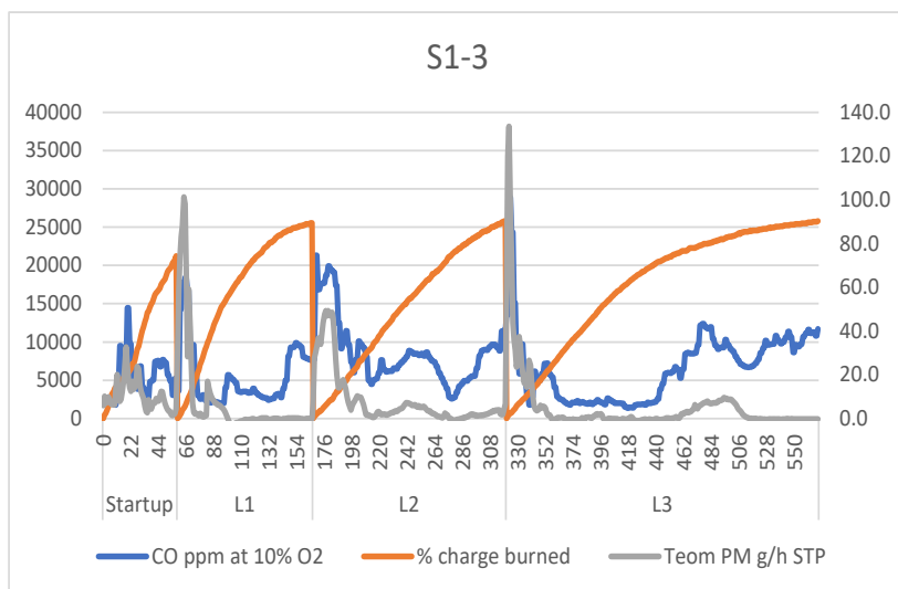
Stove 2: IDC Runs with Door Initially Cracked Open
