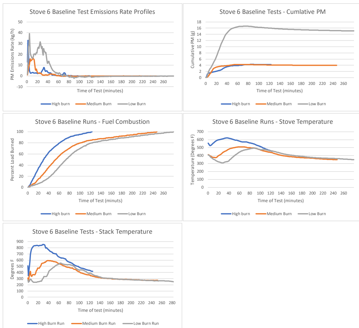
Figure 33. Stove 6—Baseline Runs—PM Emission Profiles, Cumulative PM Emissions, Cumulative Fuel Consumption, and Stove and Stack Temperatures
