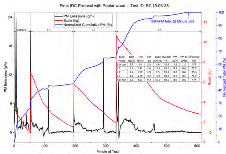
Figure 54. Stove 7—IDC Final Protocol Replicate Runs with Poplar Cordwood
