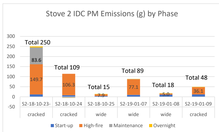
Figure 83. PM Emissions in Stove 2 IDC Runs
