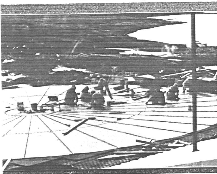
LAYING THE TANK BOTTOM
