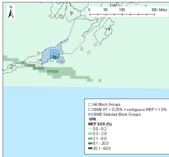
Figure 8-. Simeonof detail showing WEP SO x emissions outside of the VPA boundary that was developed following the methodology
