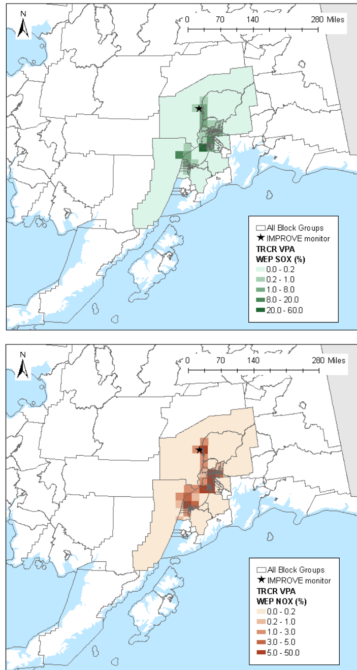
Figure 5-. SO x and NO x WEP within the VPA for Trapper Creek Site in Denali National Park and Preserve (TRCR1)
