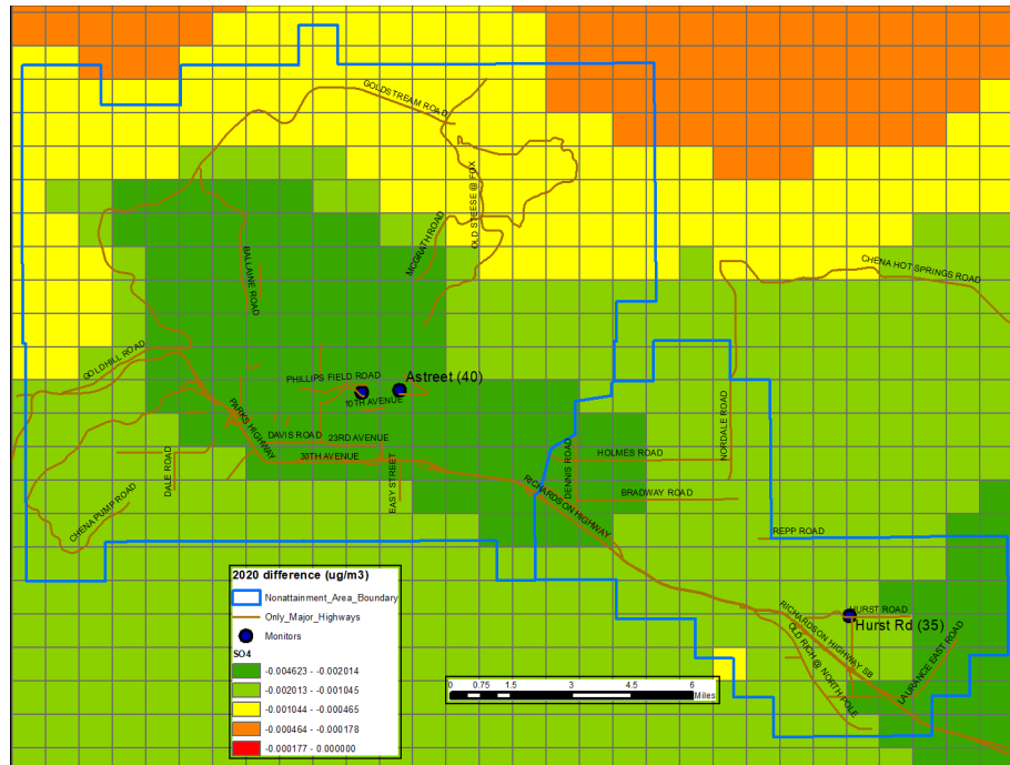
Figure 3.3.7 SO 2 point source zero out run – 2020 base case difference plot for SO 4 in µg/m 3
