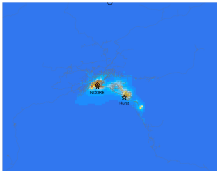
Episode average ATOTIJ ep2_Nov2_to_Nov22_org_emc
