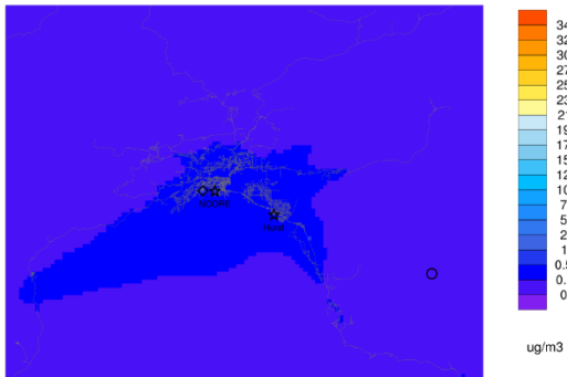
Episode average ANH4IJ ep2_Nov2_to_Nov22_org_emc
