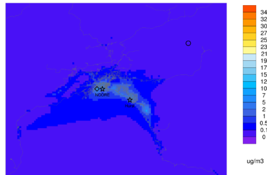
Episode average AECIJ ep2_Nov2_to_Nov22_BM
