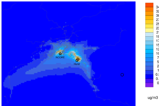
Episode average AOMIJ ep1_Jan23_to_Feb11_org_emc
