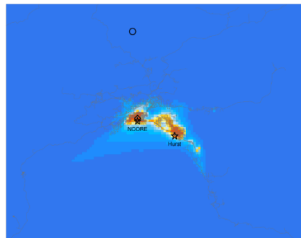
Episode average ATOTIJ ep1_Jan23_to_Feb11_BM
