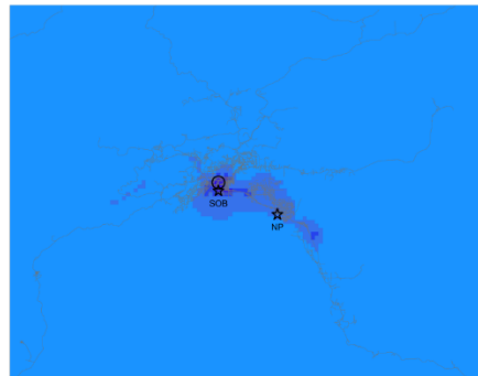
Episode average O3 episode2_Nov2_to_Nov22_particle
