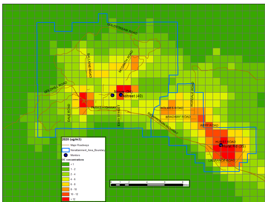
Figure 3.2.6 Organic Carbon (OC) concentration plot in \mu\text{g}/\text{m}^3 at the surface for the Fairbanks NAA for the base year 2020
