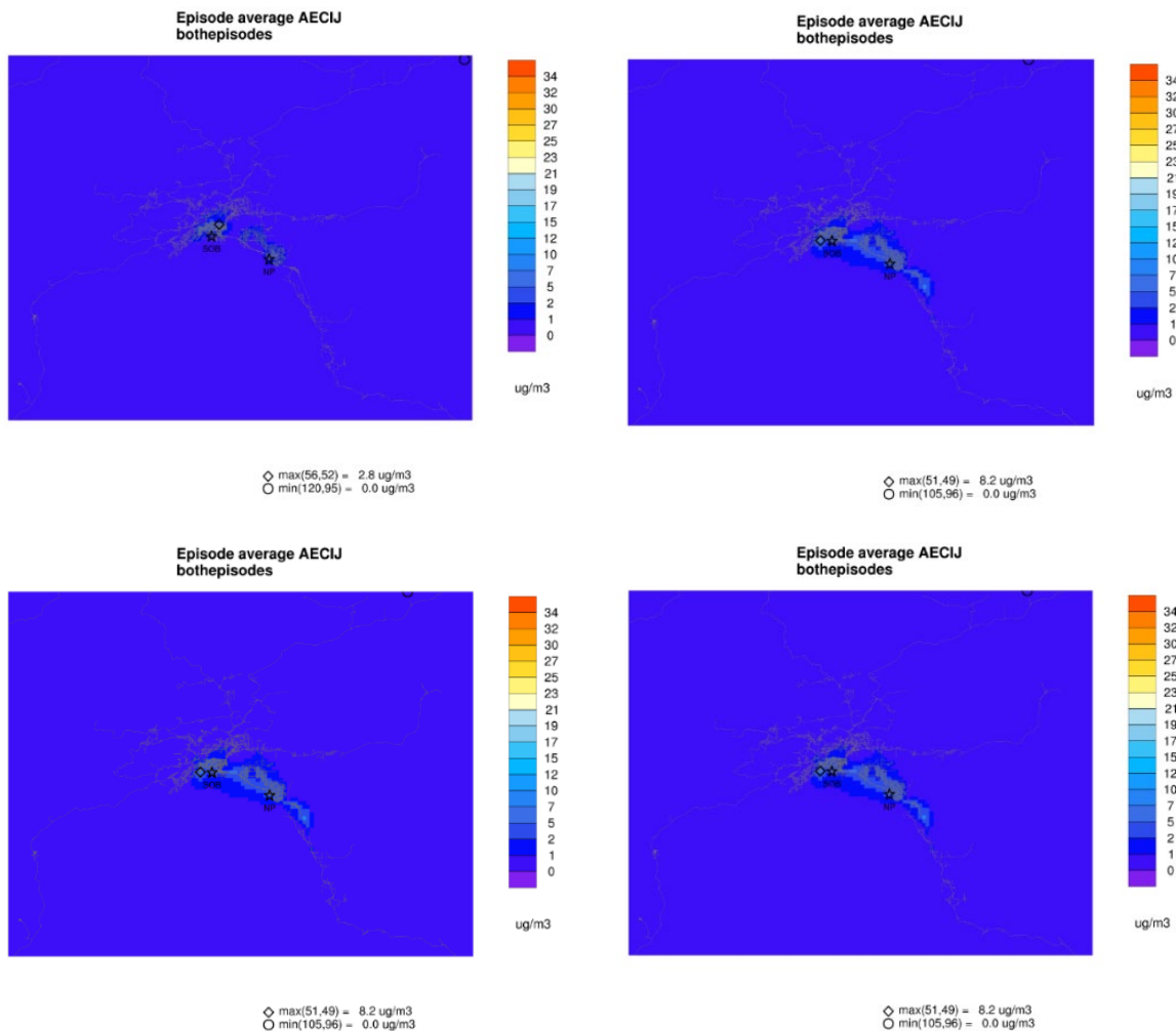
Figure 1.5.1 Elemental Carbon(AECIJ) in \mu\text{g}/\text{m}^3 both episode average concentration in the domain area at 1.33 km grid cell for 2019 base year emissions inventory using CMAQ version 4.7.1 (top left), CMAQ version 5.3.2 ORG_EMC (top right), BM (bottom left) and particle (bottom right)
