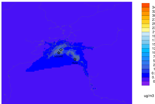
Episode average AECIJ ep2_Nov2_to_Nov22v471
