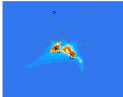
Episode average ATOTIJ ep1_Jan23_to_Feb11_particle
