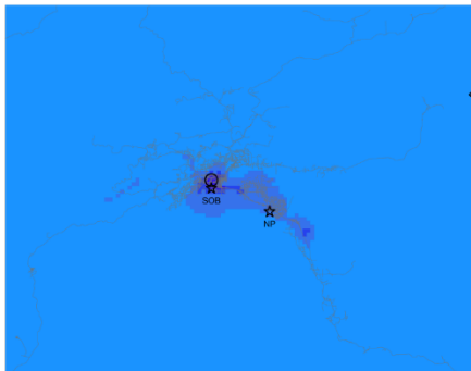
Episode average O3 episode2_Nov2_to_Nov22_org_emc
