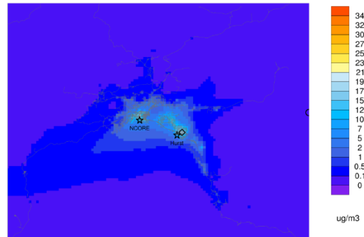
Episode average APOMIJ ep2_Nov2_to_Nov22_particle
