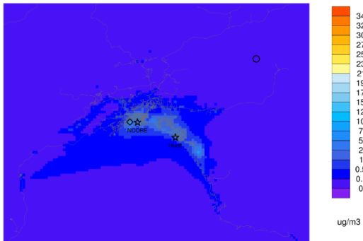
Episode average AECIJ ep2_Nov2_to_Nov22_org_emc
