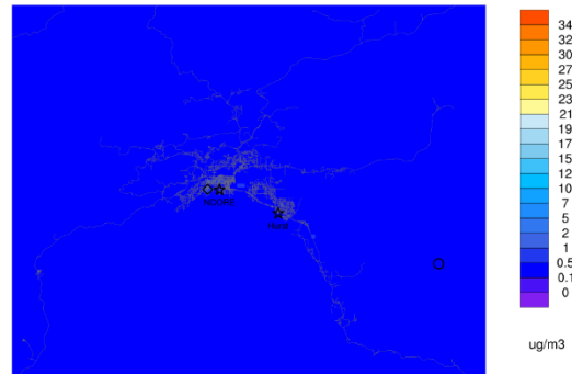
Episode average ANH4IJ ep1_Jan23_to_Feb11_particle
