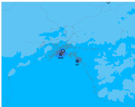
Episode average O3 episode2_Nov2_to_Nov22_v471
