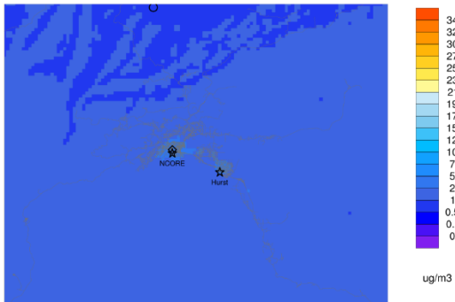
Episode average ASO4IJ ep1_Jan23_to_Feb11_org_emc
