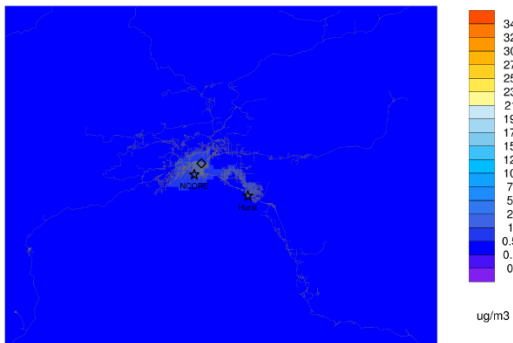
Episode average ANH4IJ ep2_Nov2_to_Nov22v471
