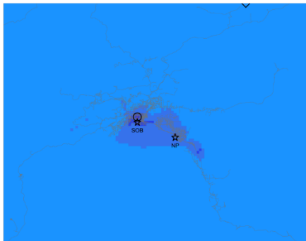
Episode average O3 episode1_Jan23_to_Feb11_org_emc
