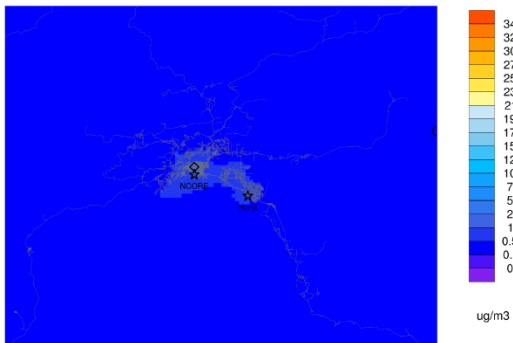
Episode average ANH4IJ ep1_Jan23_to_Feb11v471
