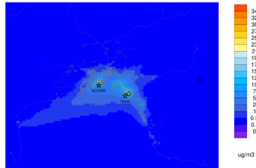
Episode average AOMIJ ep2_Nov2_to_Nov22_particle
