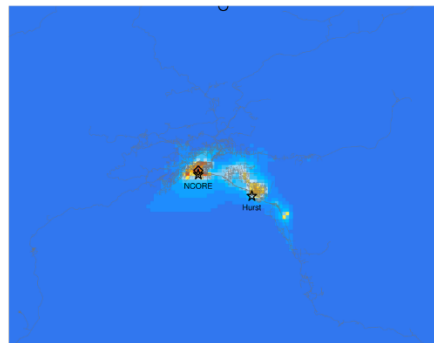
Episode average ATOTIJ ep2_BM
