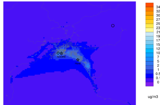
Episode average AECIJ ep2_Nov2_to_Nov22_particle
