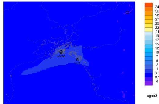
Episode average ANO3IJ ep1_Jan23_to_Feb11_particle
