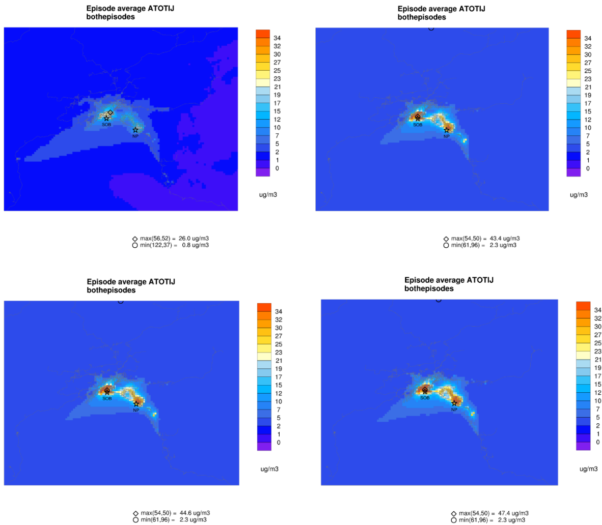
Figure 1.5.8 PM 2.5 (ATOTIJ) in \mu\text{g}/\text{m}^3 both episode average concentration in the domain area at 1.33 km grid cell for 2019 base year emissions inventory using CMAQ version 4.7.1 (top left), CMAQ version 5.3.2 ORG_EMC (top right), BM (bottom left) and particle (bottom right)
