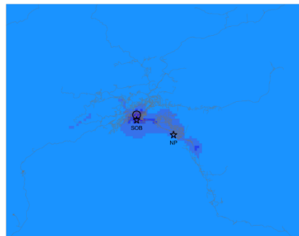
Episode average O3 episode2_Nov2_to_Nov22_BM
