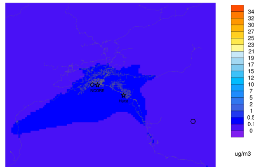
Episode average ANH4IJ ep2_Nov2_to_Nov22_BM
