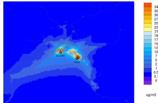
Episode average AOMIJ ep1_Jan23_to_Feb11_particle
