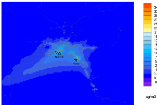
Episode average AOMIJ ep1_Jan23_to_Feb11v471
