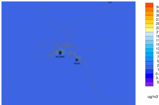
Episode average ASO4IJ episode2_Nov2_to_Nov22_org_emc
