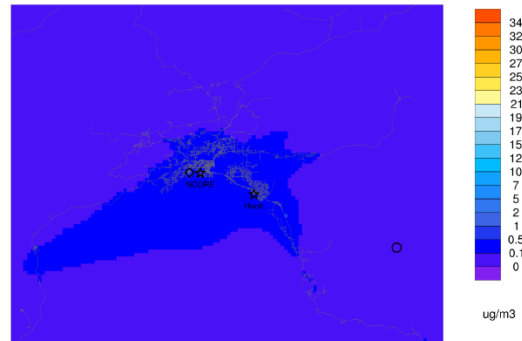
Episode average ANH4IJ ep2_Nov2_to_Nov22_particle
