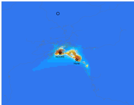
Episode average ATOTIJ ep1_Jan23_to_Feb11_org_emc
