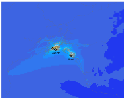
Episode average ATOTIJ ep1_Jan23_to_Feb11v471
