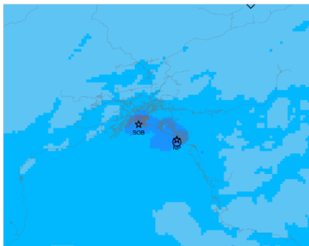
Episode average O3 episode1_Jan23_to_Feb11_v471
