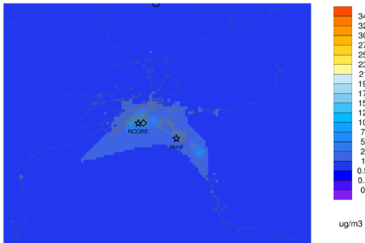
Episode average PM25_OTHUJ ep1_Jan23_to_Feb11_BM
