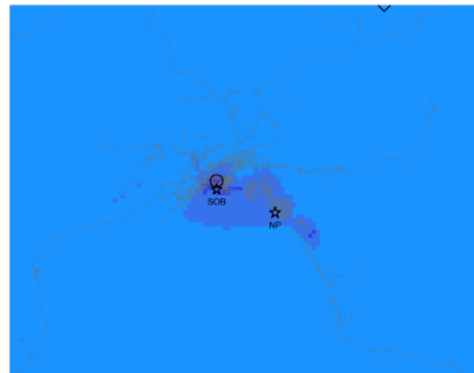
Episode average O3 episode1_Jan23_to_Feb11_particle
