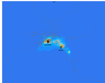
Episode average ATOTIJ ep2_Nov2_to_Nov22_particle
