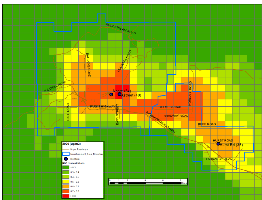
Figure 3.2.7 Nitrate ( \text{NO}_3 ) concentration plot in \mu\text{g}/\text{m}^3 at the surface for the Fairbanks NAA for the base year 2020
