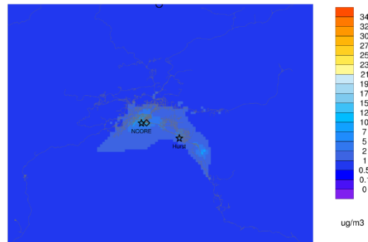
Episode average PM25_OTHUJ ep2_Nov2_to_Nov22_BM
