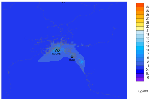
Episode average PM25_OTHUJ ep2_Nov2_to_Nov22_particle
