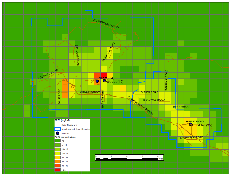
Figure 3.2.5 PM2.5 concentration plot in \mu\text{g}/\text{m}^3 at the surface for the Fairbanks NAA for the base year 2020
