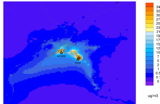
Episode average APOMIJ ep1_Jan23_to_Feb11_particle
