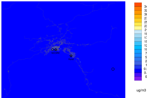
Episode average ANH4IJ ep1_Jan23_to_Feb11_org_emc
