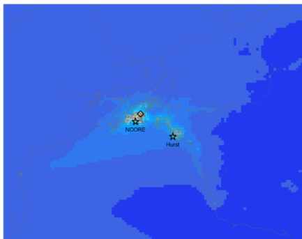
Episode average ATOTIJ ep2_Nov2_to_Nov22v471
