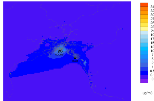
Episode average PM25_OTH ep2_Nov2_to_Nov22v471
