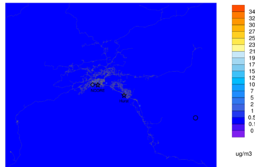
Episode average ANH4IJ ep1_Jan23_to_Feb11_BM
