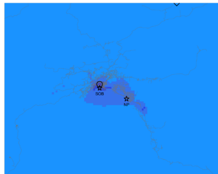
Episode average O3 episode1_Jan23_to_Feb11_BM
