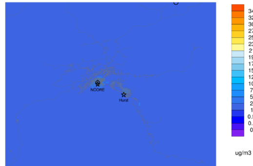
Episode average ASO4IJ ep2_Nov2_to_Nov22_particle
