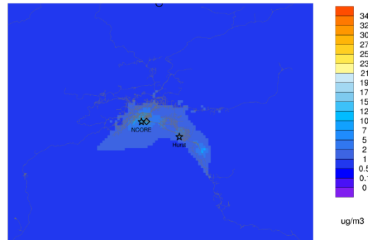
Episode average PM25_OTHUJ ep2_Nov2_to_Nov22_org_emc
