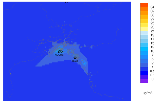
Episode average PM25_OTHJ ep1_Jan23_to_Feb11_particle
