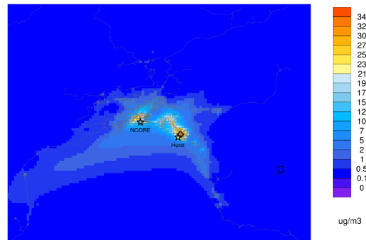
Episode average AOMIJ ep1_Jan23_to_Feb11_BM
