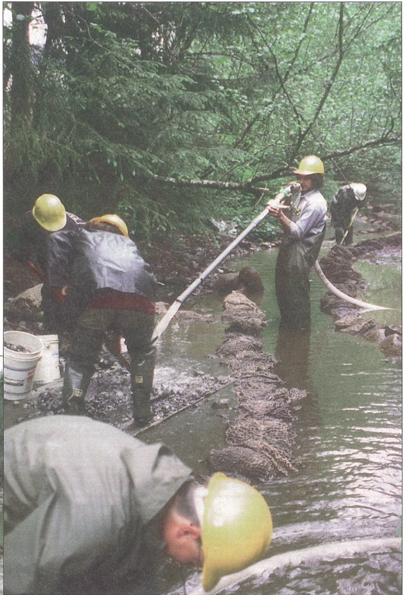
Figure 10.--An Americorps crew using dredging equipment to remove fine sediment from a salmon spawning area in Duck Creek. (Photo by NMFS).
