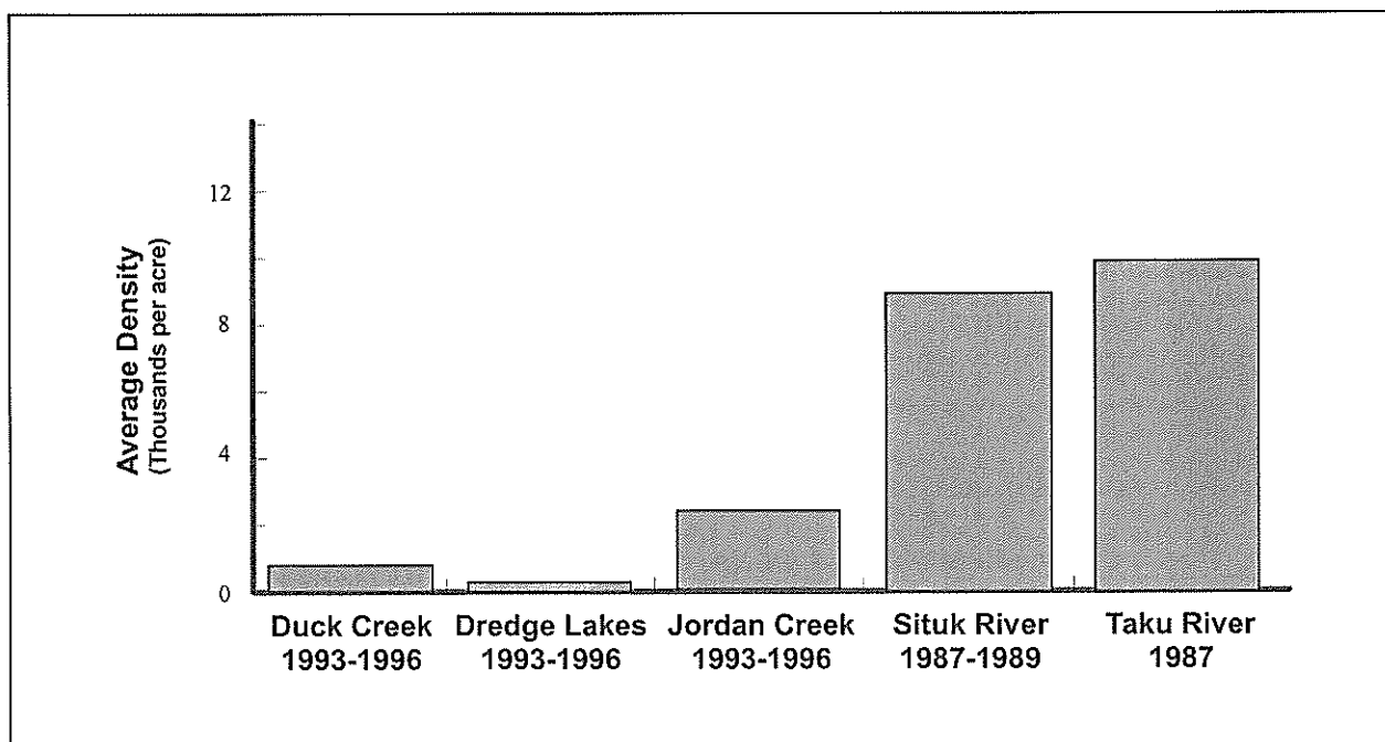
Figure 17.--Juvenile coho density during fall at five Southeast Alaska areas.
