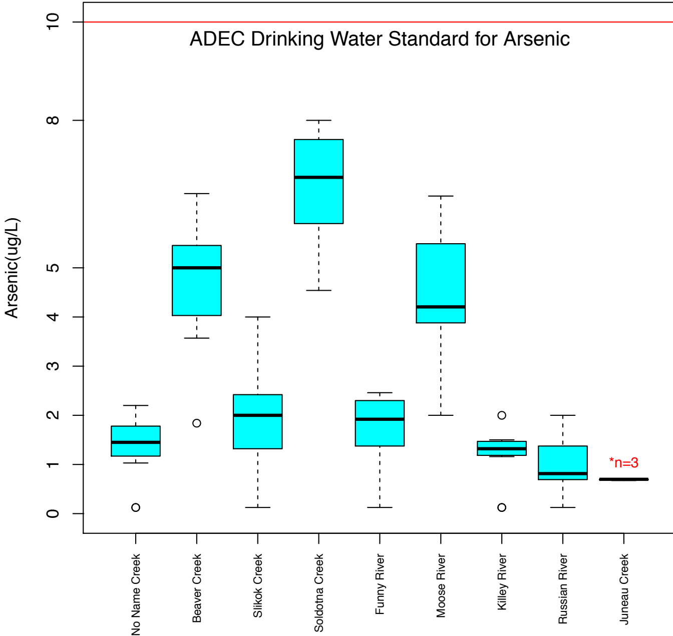
Figure 31: Arsenic sampled in Kenai River tributaries during spring 2001 to 2014 compared to ADEC drinking water standards. Since 25% of the samples are reported as below the MRL or MDL, these values have been estimated using values that are half of the MRL or MDL.
