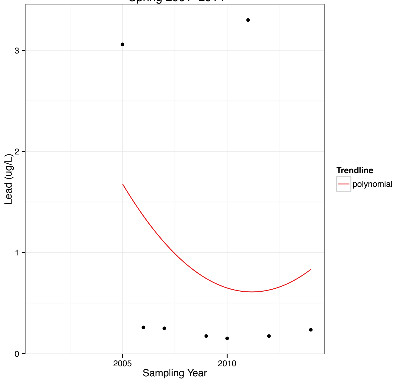
Figure 51: Trend analysis for lead sampled at Mile 6.5 from spring 2001 to 2014, Kenai River. Not detected values are not taken into account in the analysis and therefore are not shown in this graph.
