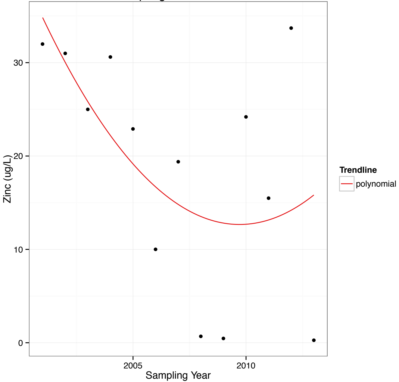
Figure 72: Trend analysis for zinc sampled at Mile 50 from spring 2001 to 2014. Not detected values are not taken into account in the analysis and therefore are not shown in this graph.
