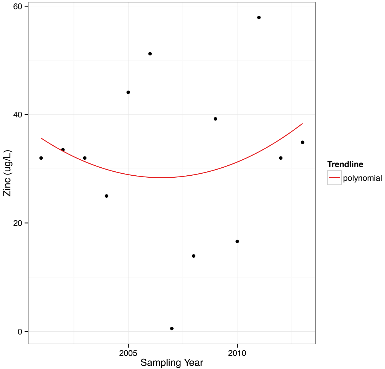
Figure 82: Trend analysis for zinc sampled at Mile 31 from summer 2000 to 2014. Not detected values are not taken into account in the analysis and therefore are not shown in this graph.
