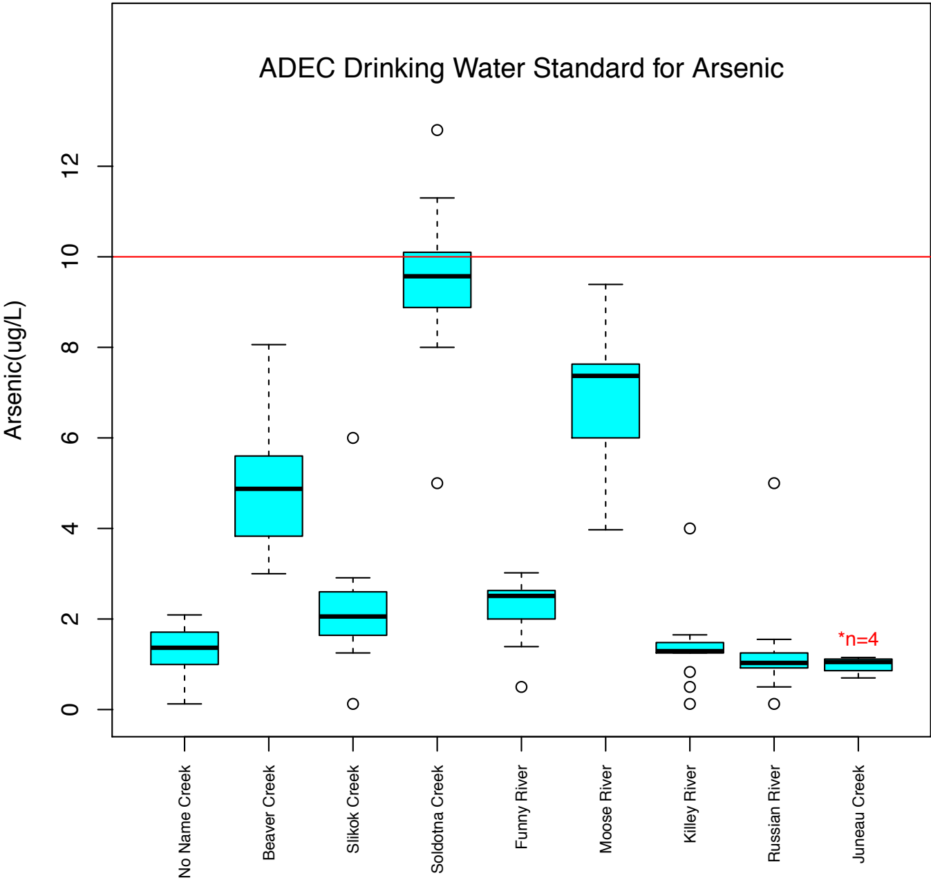
Figure 33: Arsenic sampled in Kenai River tributaries during summer 2000 to 2014 compared to ADEC drinking water standards. Since 20% of the samples are reported as below the MRL or MDL, these values have been estimated using values that are half of the MRL or MDL.
