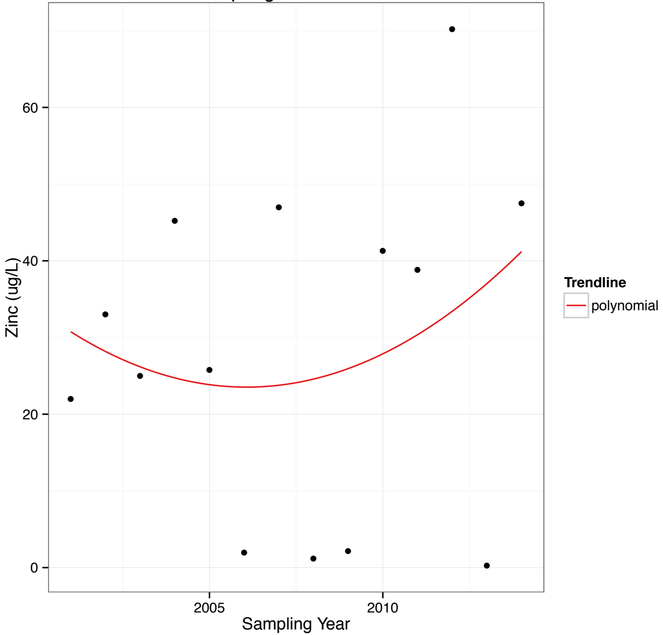
Figure 68: Trend analysis for zinc sampled at Mile 23 from spring 2001 to 2014. Not detected values are not taken into account in the analysis and therefore are not shown in this graph.
