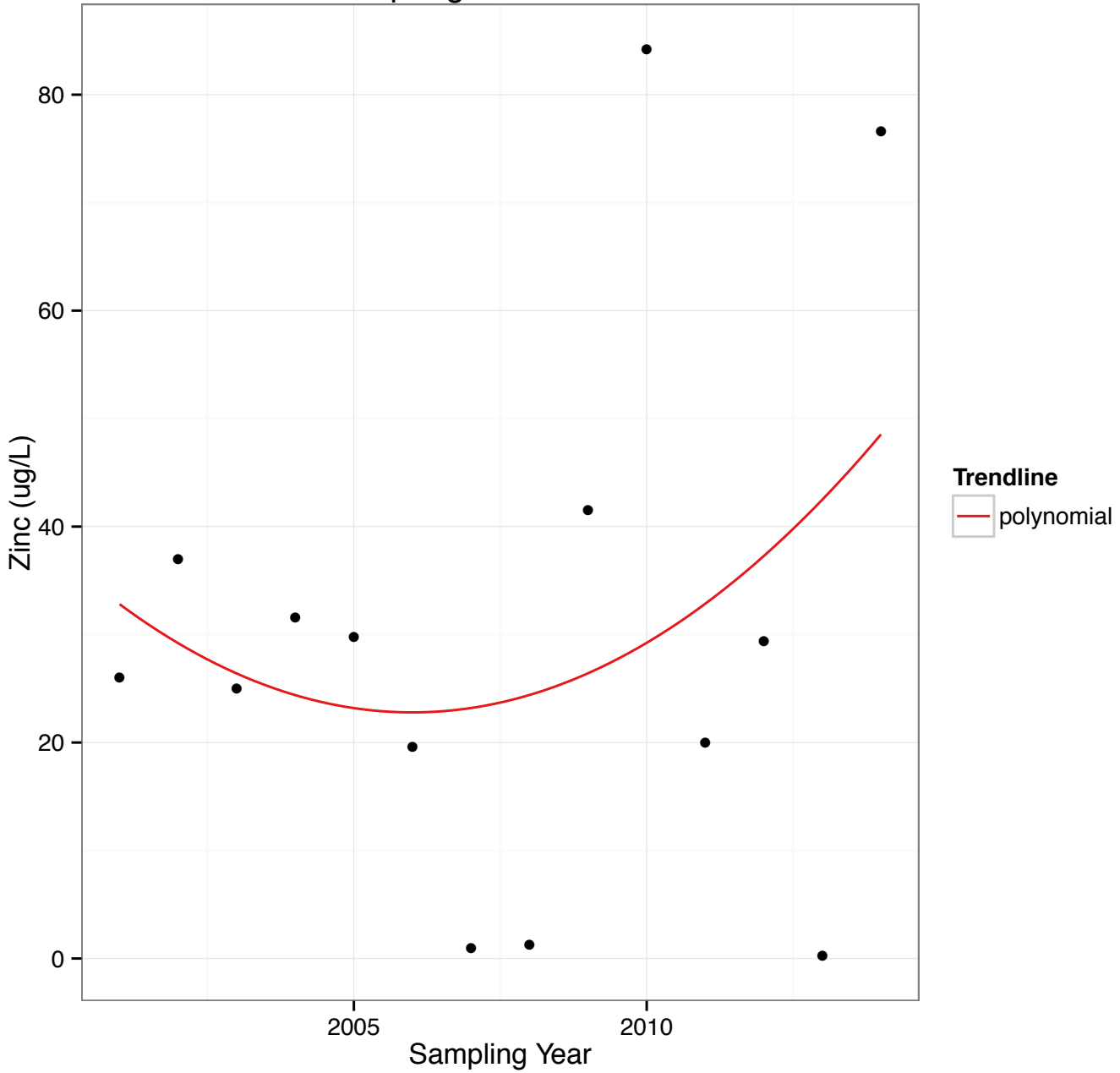
Figure 65: Trend analysis for zinc sampled at Mile 12.5 from spring 2001 to 2014. Not detected values are not taken into account in the analysis and therefore are not shown in this graph.
