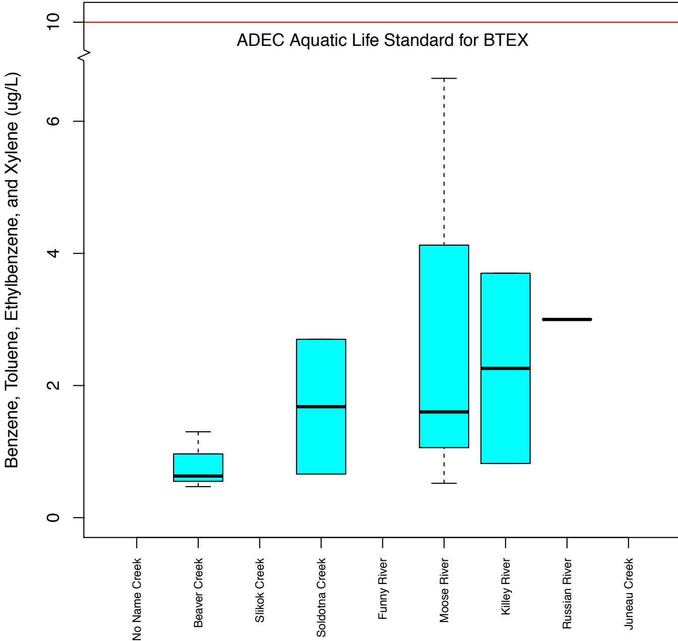
Figure 117: Total BTEX sampled in Kenai River tributaries during summer 2000 to 2012. Miles 1.5, 6.5, 40 and 43 were also sampled during the 2013 event and that data was used to produce this graph. This graph does not include instances of non-detect, in which all of the BTEX samples were reported as below the MRL or MDL.
