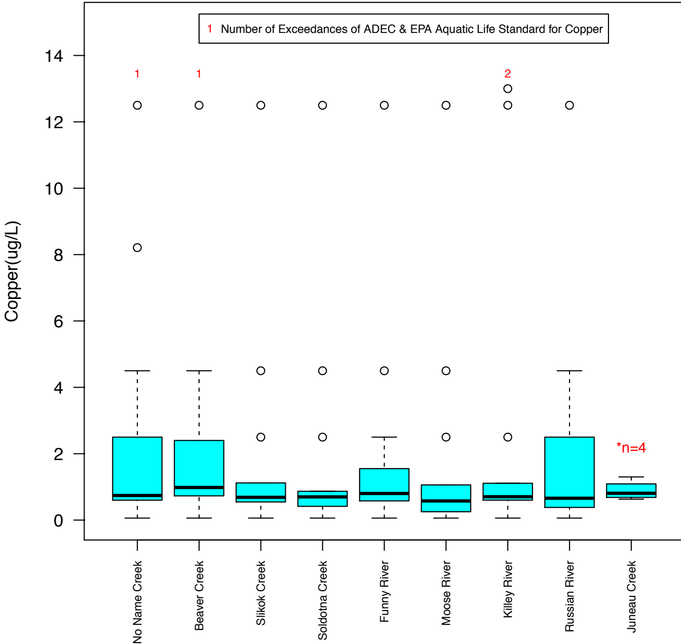
Figure 42: Copper sampled in Kenai River tributaries during spring 2001 to 2014 with hardness dependent standards and exceedances. Since 32% of the samples are reported as below the MRL or MDL, these values have been estimated using values that are half of the MRL or MDL.
