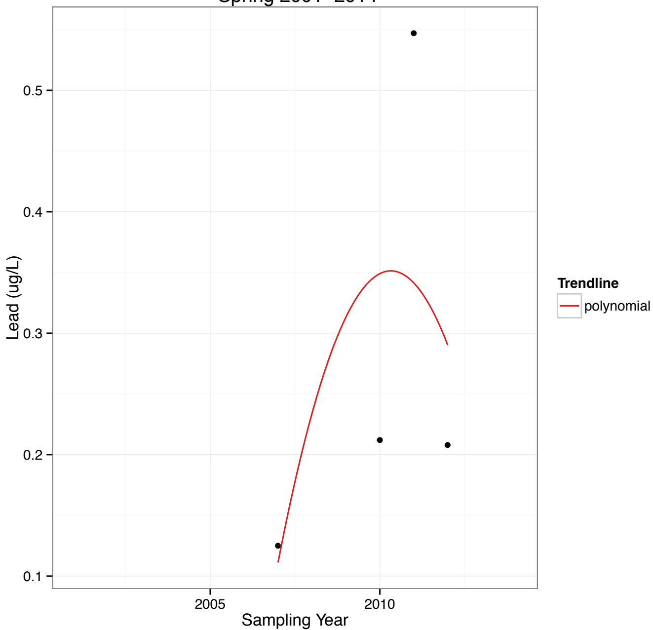
Figure 52: Trend analysis for lead sampled at Mile 10.1 from spring 2001 to 2014, Kenai River. Not detected values are not taken into account in the analysis and therefore are not shown in this graph.
