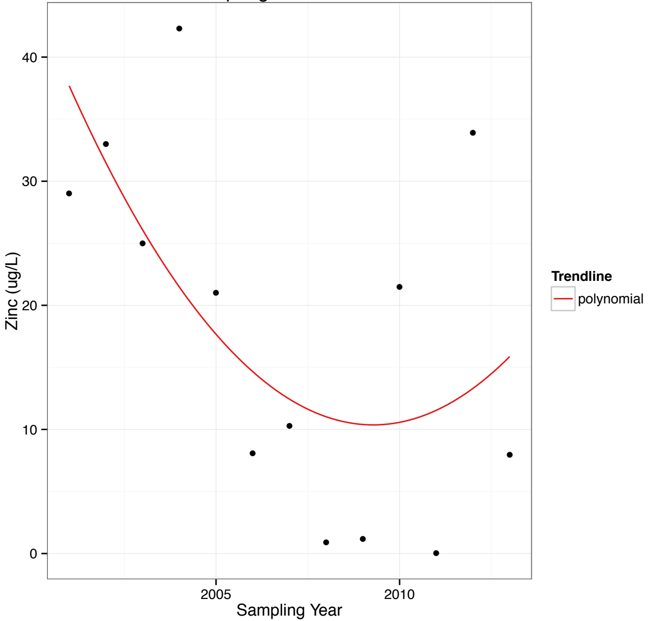
Figure 71: Trend analysis for zinc sampled at Mile 43 from spring 2001 to 2014. Not detected values are not taken into account in the analysis and therefore are not shown in this graph.
