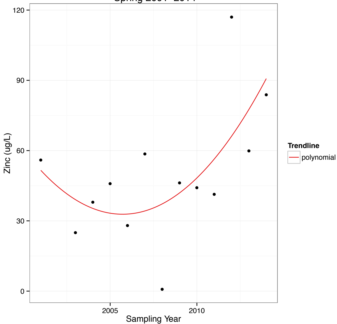
Figure 64: Trend analysis for zinc sampled at Mile 10.1 from spring 2001 to 2014. Not detected values are not taken into account in the analysis and therefore are not shown in this graph.
