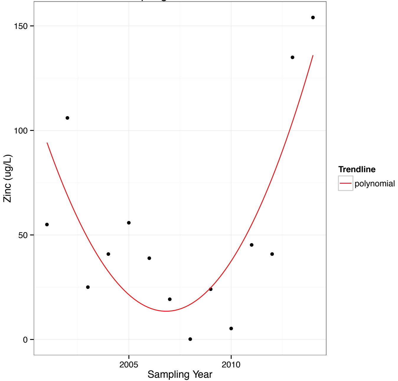
Figure 62: Trend analysis for zinc sampled at Mile 1.5 from spring 2001 to 2014. Not detected values are not taken into account in the analysis and therefore are not shown in this graph.
