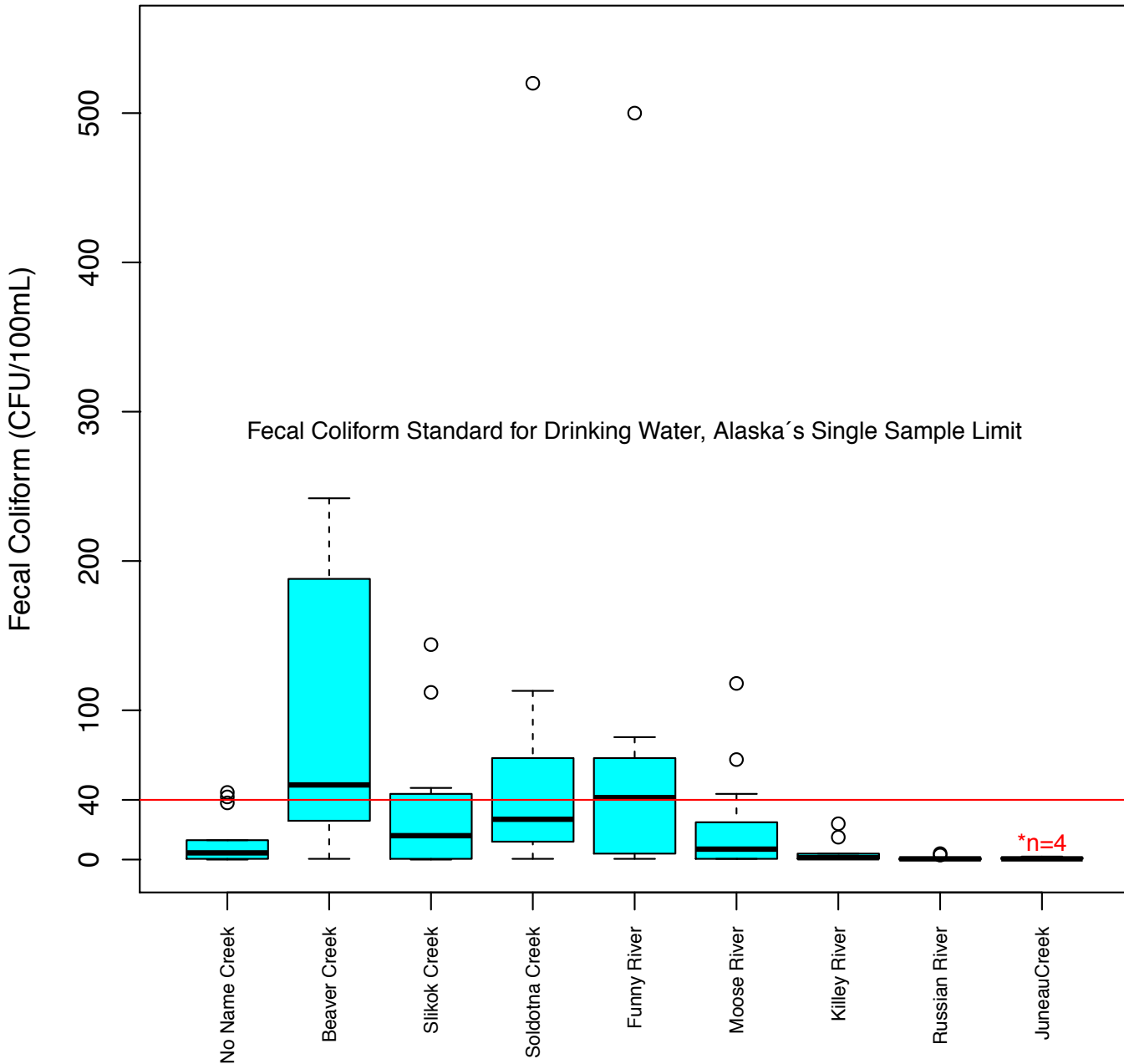
Figure 131: Fecal Coliform Bacteria sampled in Kenai River tributaries during summer 2000 to 2014 compared to ADEC standards. Since 26% of the samples are reported as below the MRL or MDL, these values have been estimated using values that are half of the MRL or MDL.
