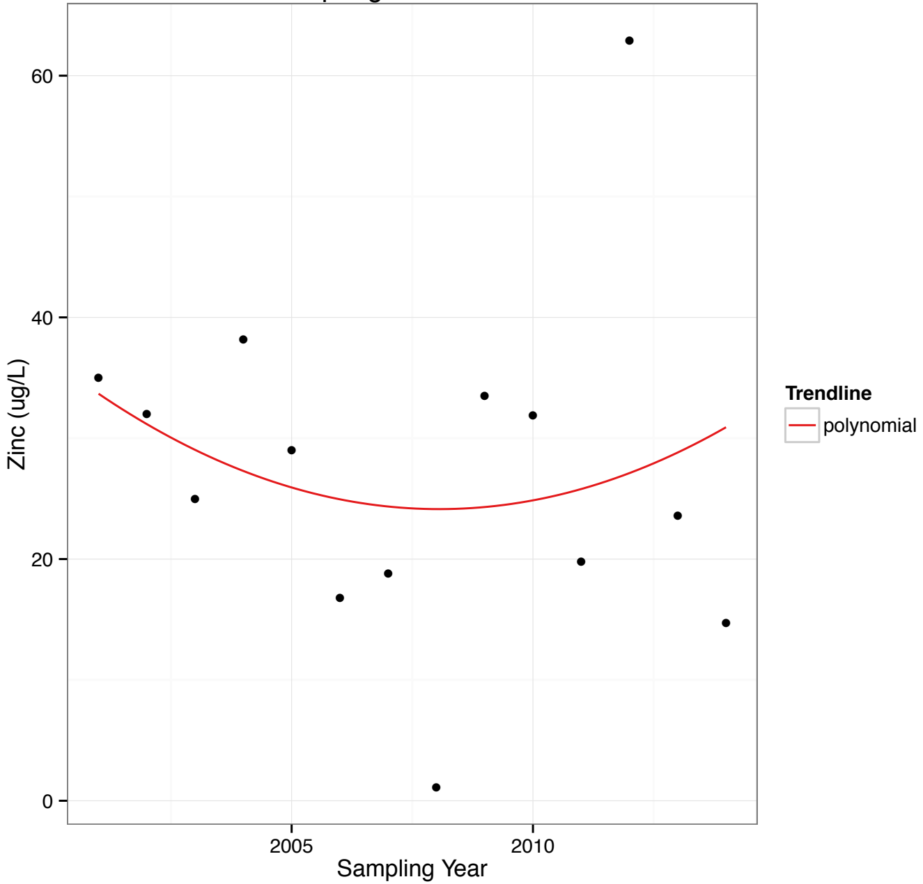
Figure 67: Trend analysis for zinc sampled at Mile 21 from spring 2001 to 2014. Not detected values are not taken into account in the analysis and therefore are not shown in this graph.
