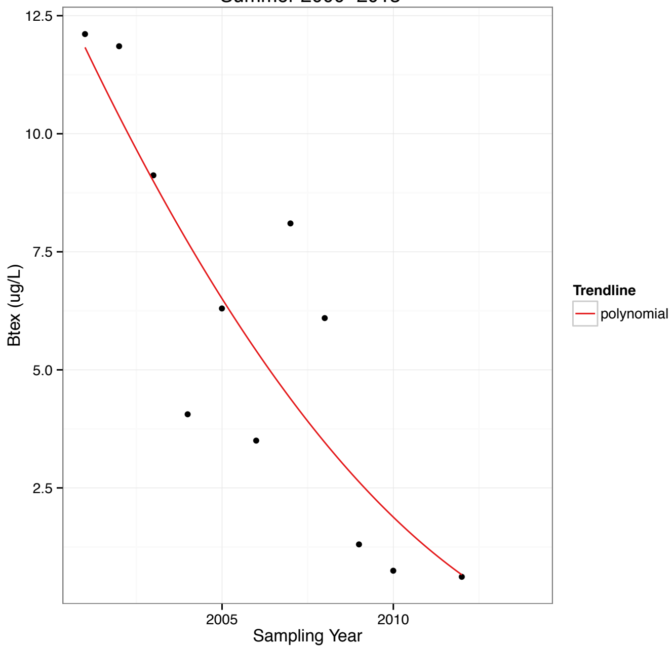
Figure 121: Trend analysis for BTEX sampled at Mile 6.5 from summer 2000 to 2013. Not detected values are not taken into account in the analysis and therefore are not shown in this graph.
