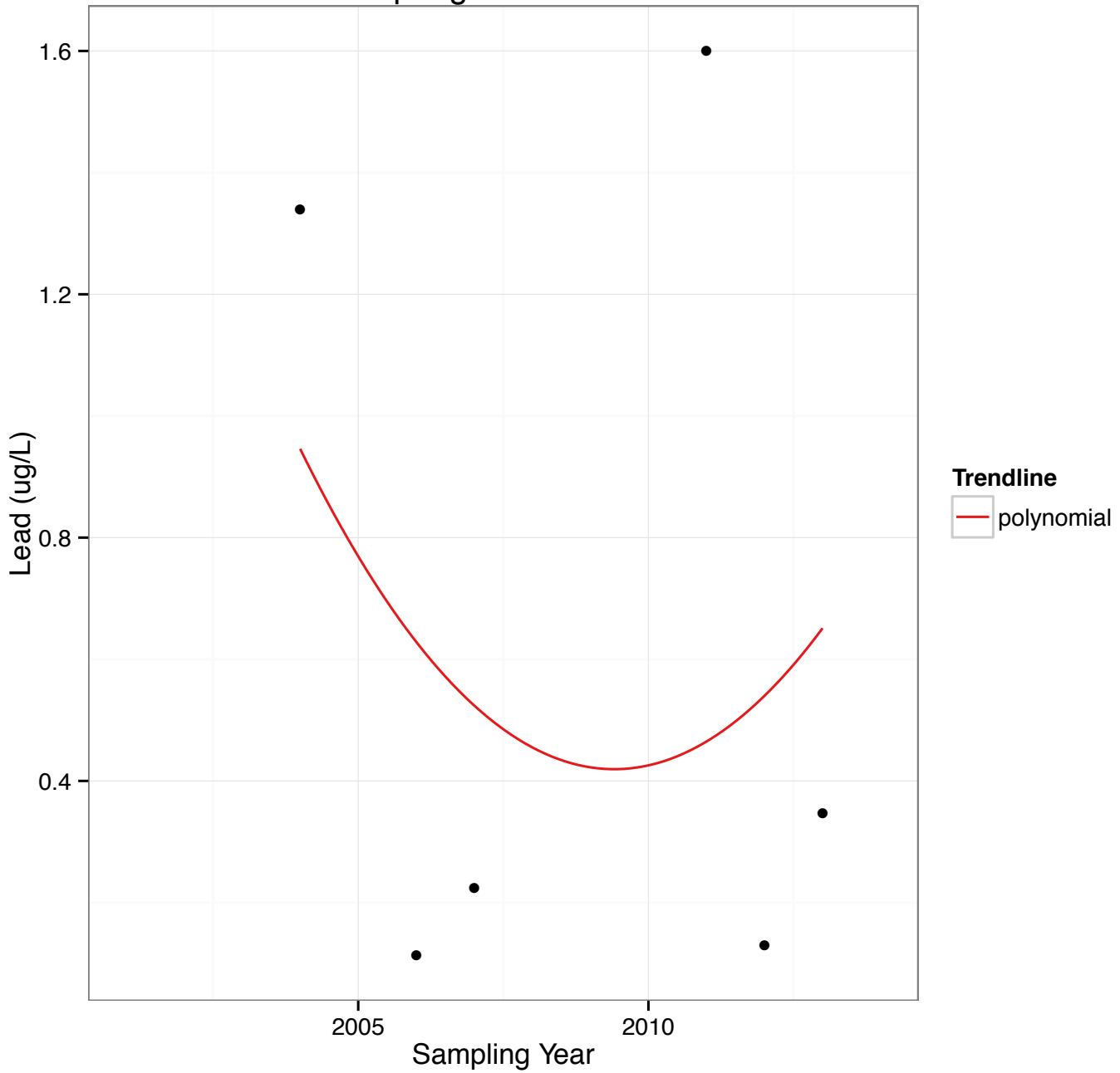
Figure 50: Trend analysis for lead sampled at Mile 1.5 from spring 2001 to 2014, Kenai River. Not detected values are not taken into account in the analysis and therefore are not shown in this graph.
