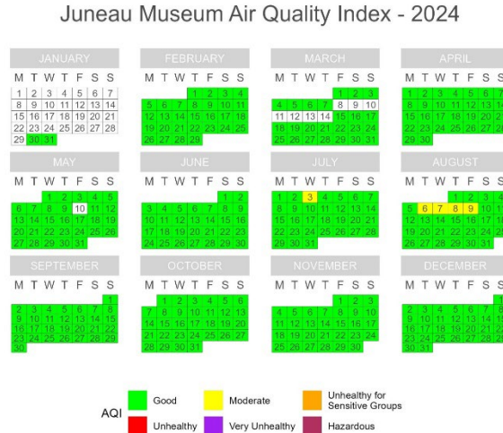
Figure 39. PM 2.5 Calendar Plots for Juneau at the State Museum (4/1/2024 – 9/30/2024).
