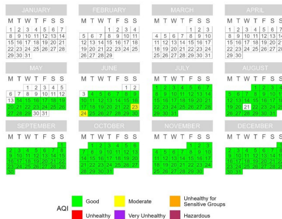
Figure 33. PM 2.5 Calendar Plots for Ninilchik (5/14/2024 – 9/30/2024).
