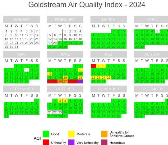
Figure 16. PM 2.5 Calendar Plots for Goldstream (4/1/2024 – 9/30/2024).
