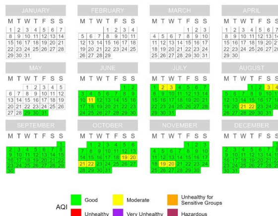
Figure 21. PM 2.5 Calendar Plots for Nome (5/28/2024 – 9/30/2024).
