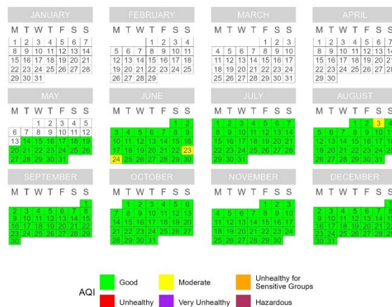
Figure 35. PM 2.5 Calendar Plots for Soldotna (5/14/2024 – 9/30/2024).
