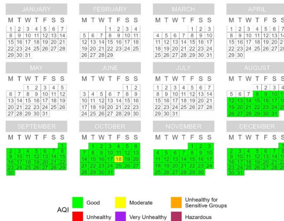
Figure 25. PM 2.5 Calendar Plots for Chickaloon/Sutton-Alpine (8/7/2024 – 9/30/2024).
