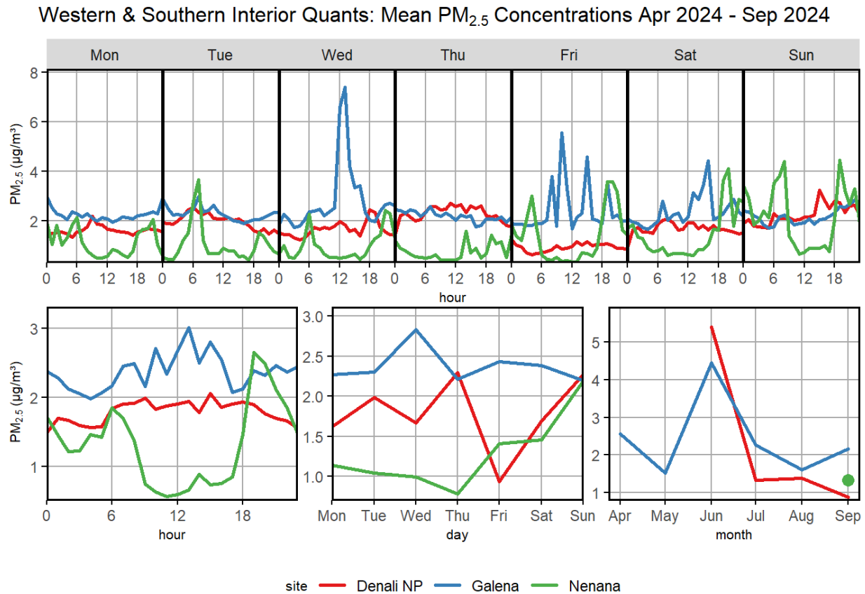
Figure 2. PM 2.5 Concentrations in Denali NP, Galena, and Nenana (4/1/2024 – 9/30/2024) after removal of days affected by wildland fire smoke.
