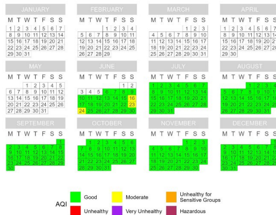
Figure 34. PM 2.5 Calendar Plots for Seward (6/5/2024 – 9/30/2024).
