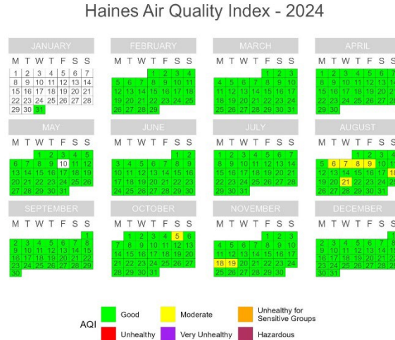
Figure 36. PM 2.5 Calendar Plots for Haines (4/1/2024 – 9/30/2024).
