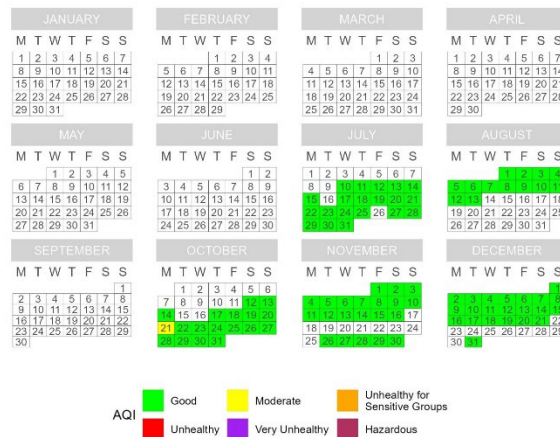
Figure 20. PM 2.5 Calendar Plots for Kotzebue (7/10/2024 – 9/30/2024).
