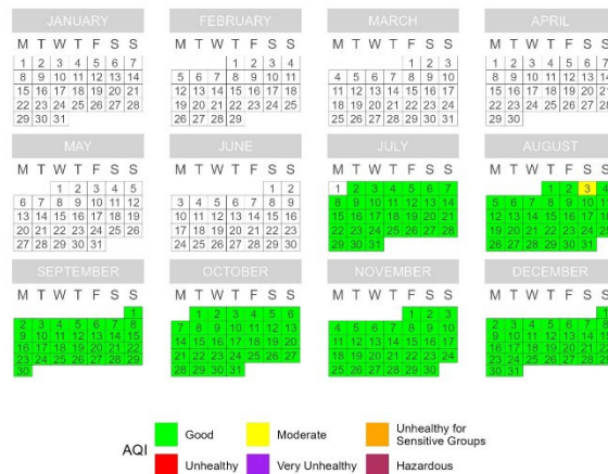
Figure 26. PM 2.5 Calendar Plots for Talkeetna (7/1/2024 – 9/30/2024).
