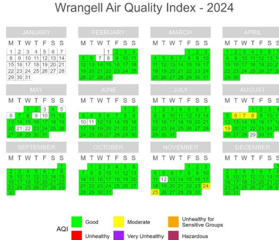
Figure 43. PM 2.5 Calendar Plots for Wrangell (4/1/2024 – 9/30/2024).
