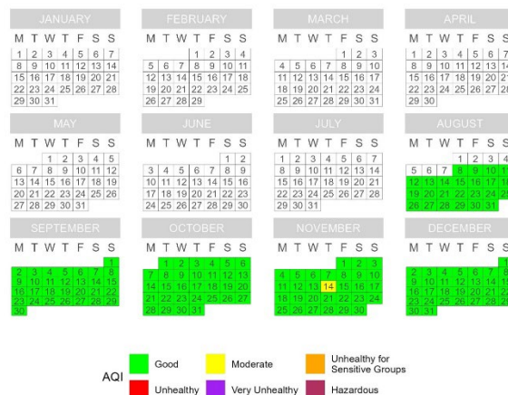
Figure 27. PM 2.5 Calendar Plots for Palmer (8/7/2024 – 9/30/2024).
