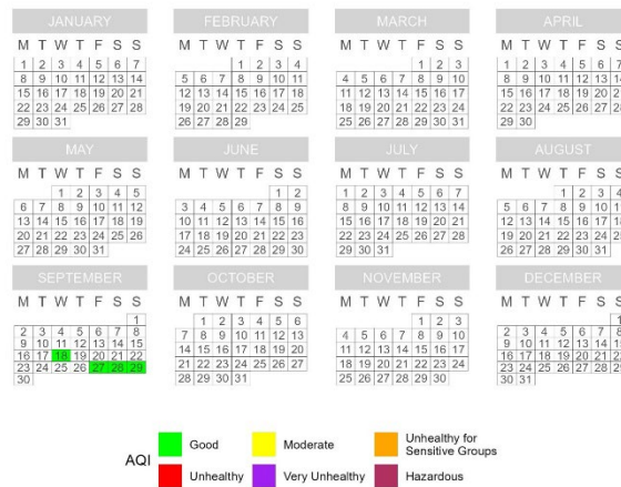
Figure 30. PM 2.5 Calendar Plots for Cordova (9/18/2024 – 9/30/2024).
