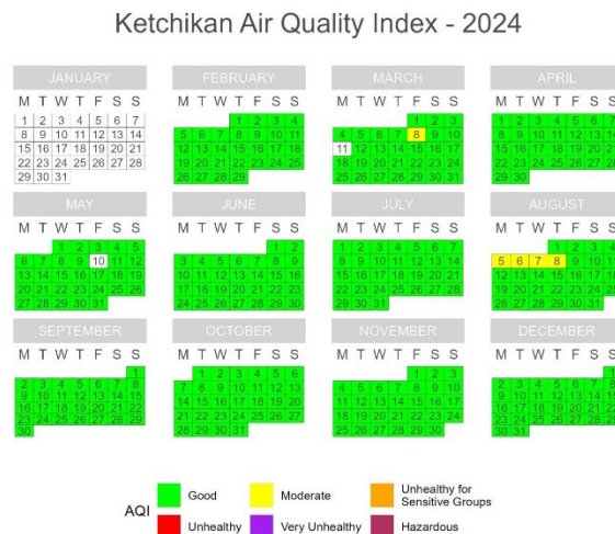
Figure 42. PM 2.5 Calendar Plots for Ketchikan (4/1/2024 – 9/30/2024).
