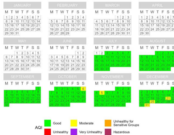
Figure 22. PM 2.5 Calendar Plots for Kodiak (7/2/2024 – 9/30/2024).
