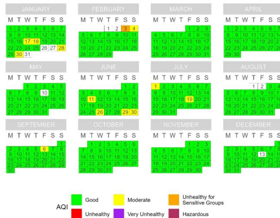
Figure 19. PM 2.5 Calendar Plots for Galena (4/1/2024 – 9/30/2024).
