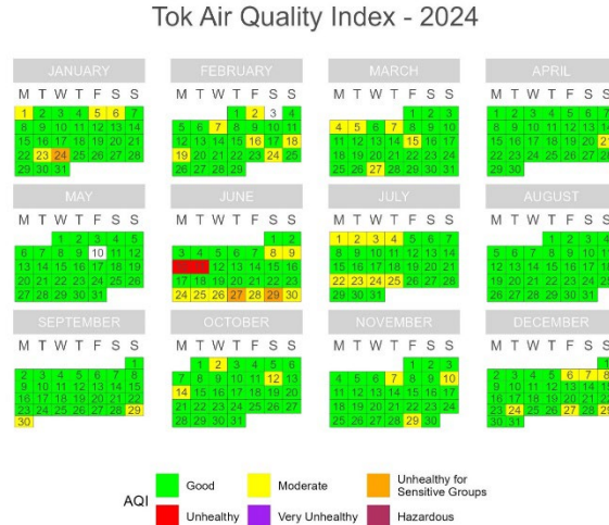
Figure 17. PM 2.5 Calendar Plots for Tok (4/1/2024 – 9/30/2024).
