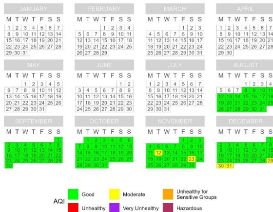
Figure 29. PM 2.5 Calendar Plots for Willow (8/7/2024 – 9/30/2024).
