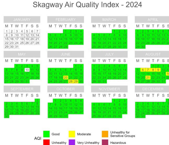
Figure 37. PM 2.5 Calendar Plots for Skagway (4/1/2024 – 9/30/2024).
