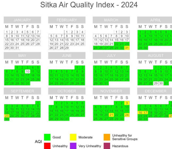
Figure 41. PM 2.5 Calendar Plots for Sitka (4/1/2024 – 9/30/2024).
