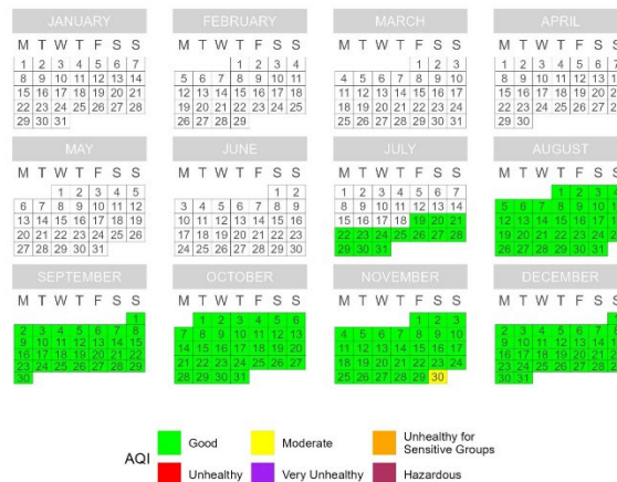
Figure 31. PM 2.5 Calendar Plots for Glennallen (7/18/2024 – 9/30/2024).
