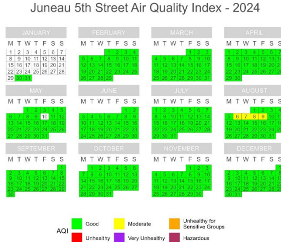
Figure 38. PM 2.5 Calendar Plots for Juneau at 5 th Street (4/1/2024 – 9/30/2024).
