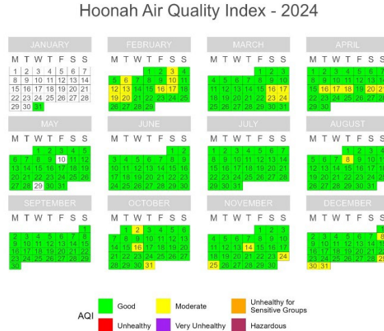
Figure 40. PM 2.5 Calendar Plots for Hoonah (4/1/2024 – 9/30/2024).
