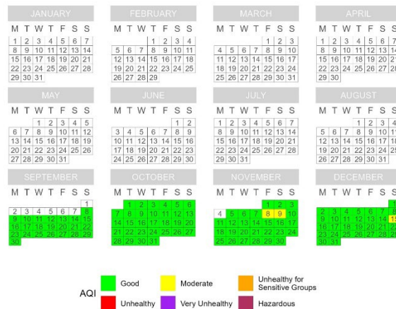
Figure 18. PM 2.5 Calendar Plots for Nenana (9/7/2024 – 9/30/2024).
