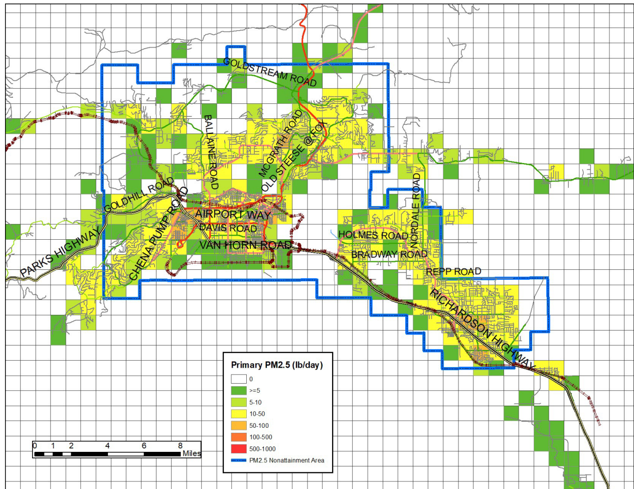
Figure 7.6-38. 2019 Baseline Gridded PM 2.5 Emissions, Space Heating Sources
