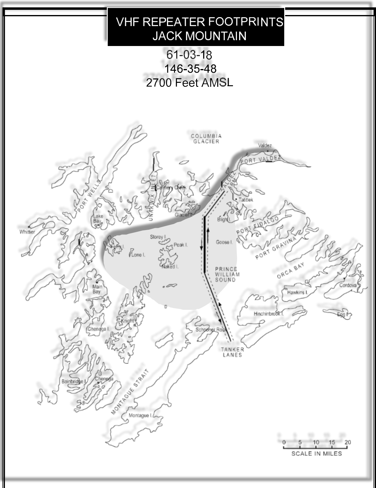
I figure FIGURE 5-3: VHF REPEATER FOOTPRINTS JACK MOUNTAIN
