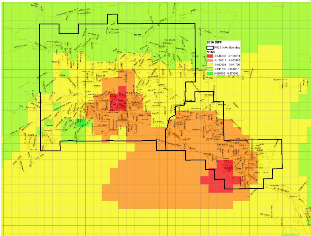
Figure 7.8-22. 2019 difference (2019-2013) of 24-hour averaged modeled NH 4 (ammonium) concentrations for the Nonattainment Area over All Episode Days (January 23 to February 10 and November 2 to 17, 2008)
