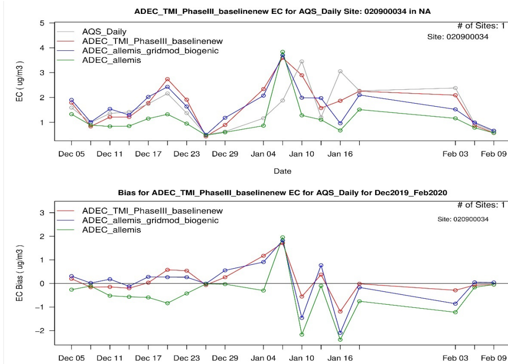
Figure 7.8.15-24 Timeseries Plot for NCore EC Using the Baseline 2020 Modeling Run and the Latest CMAQ Configuration (v533hetchem) 2020 Emissions and Meteorology
