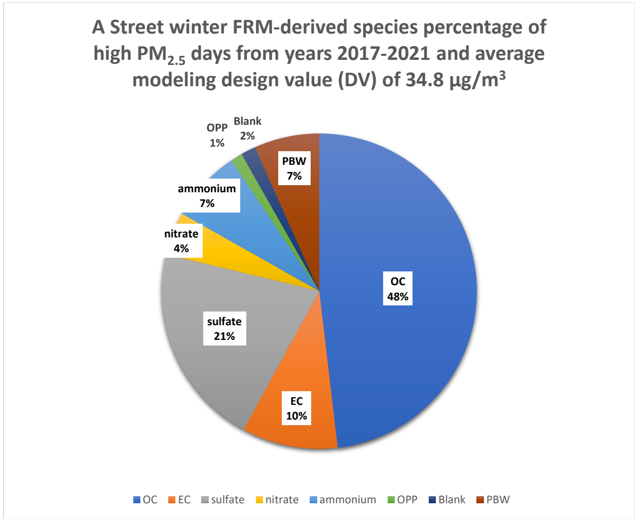
Figure 7.8.15-36 24-hr Average FRM-Derived PM 2.5 Speciation Concentrations Based on the Design Value (DV) of 34.8 µg/m 3 for A Street Monitor
