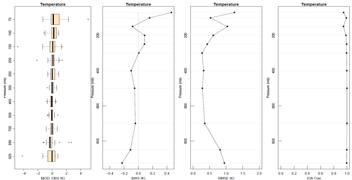
Figure X: Temperature profile statistics for the Dec-Feb modeling period at PAFA. Tiles include the distribution of Temperature difference (mod-obs), model bias, error (RMSE) and index of agreement
