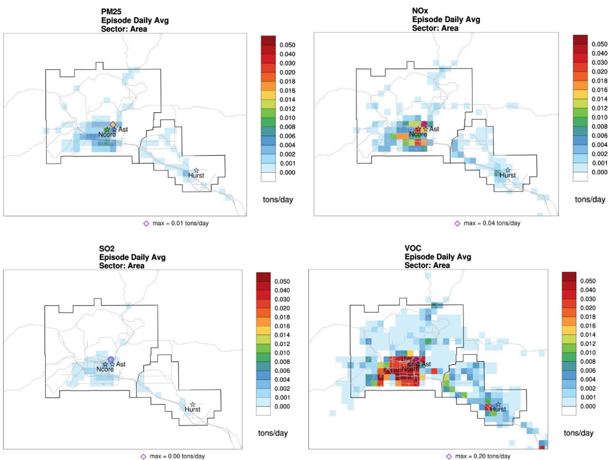
Figure 7.8.15-4 Area Source Base Year 2020 Gridded Emissions Spatial Plots for PM 2.5 (Upper Left), NO x (Upper Right), SO 2 (Lower Left), and VOC (Lower Right)
