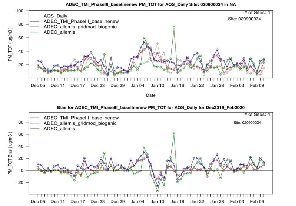
Figure 7.8.15-17 Timeseries Plot for NCore Total PM 2.5 (PM_TOT) Using the Baseline 2020 Modeling Run and the Latest CMAQ Configuration (v533het) 2020 Emissions and Meteorology
