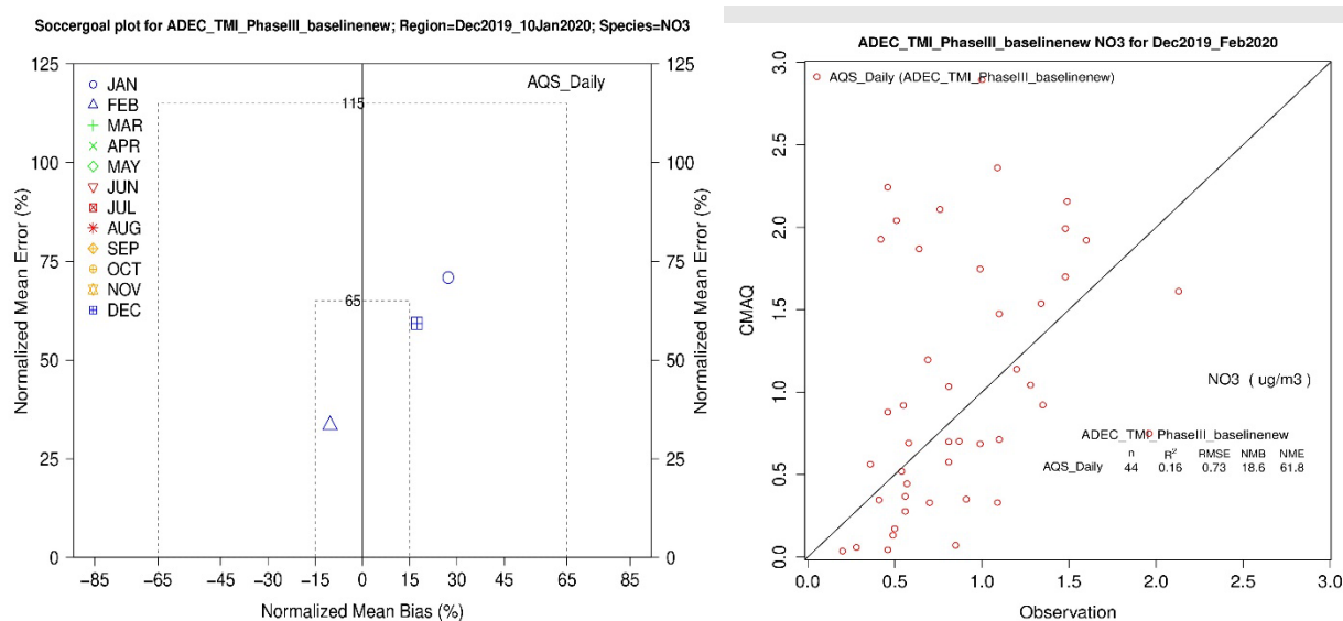
Figure 7.8.15-11 Domain wide Soccer Plot (Left) and Scatter Plot (Right) for NO 3 Using the Baseline 2020 Modeling Run and the Latest CMAQ Configuration (v533hetchem) 2020 Emissions and Meteorology
