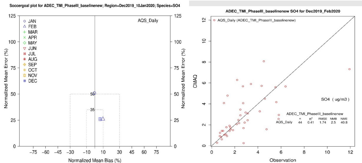
Figure 7.8.15-12 Domain wide Soccer Plot (Left) and Scatter Plot (Right) for SO 4 Using the Baseline 2020 Modeling Run and the Latest CMAQ Configuration (v533hetchem) 2020 Emissions and Meteorology
