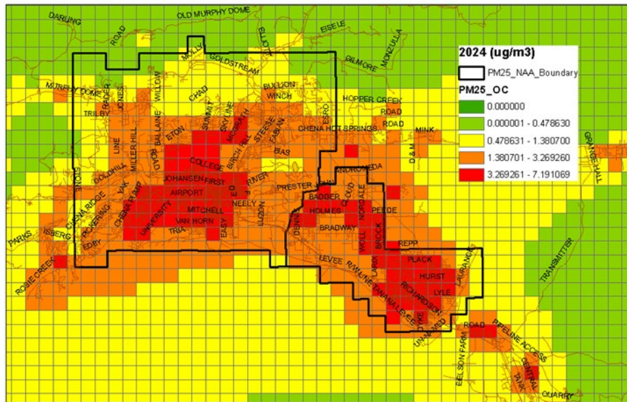
Figure 7.8.14.2-2 Non-attainment area grid cell plot for the modeling year 2024 24-hr average Organic Carbon ( \mu\text{g}/\text{m}^3 ) for all episode days
