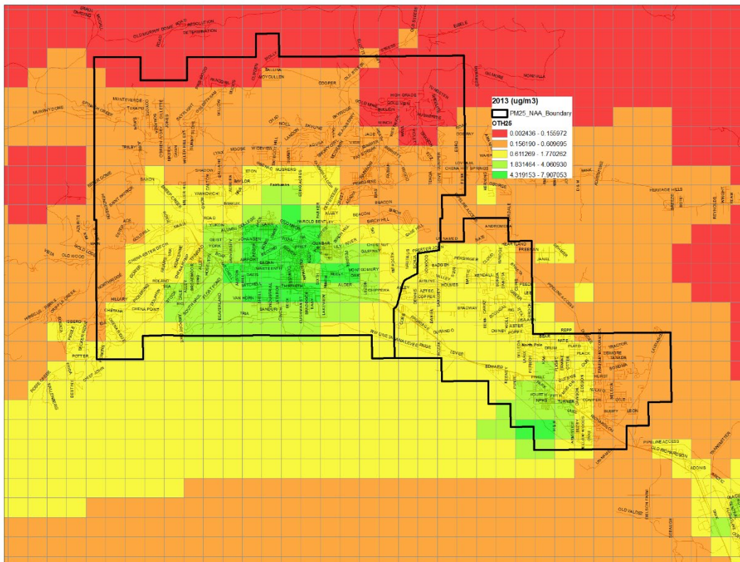
Figure 7.8-15. 2013 Base year 24-hour Averaged Model Other PM 2.5 Concentrations for the Nonattainment Area over All Episode Days (January 23 to February 10 and November 2 to 17, 2008)
