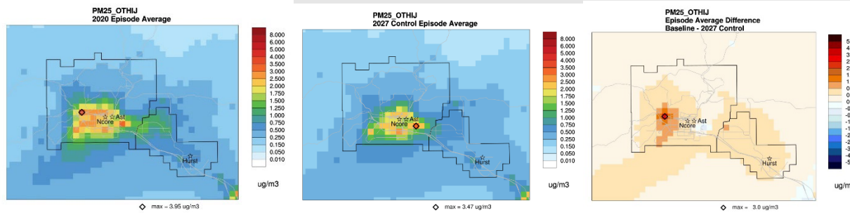
Figure 7.8.16-2 Base Year 2020, 2027 (Control Run), Difference PM Other Plots
