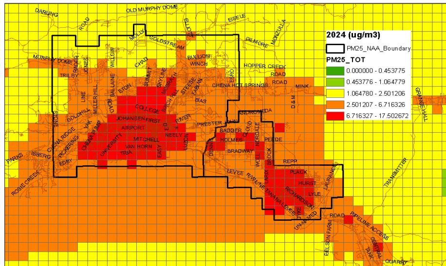
Figure 7.8.14.2-1 Non-attainment area grid cell plot for the modeling year 2024 24-hr average PM 2.5 ( \mu\text{g}/\text{m}^3 ) for all episode days
