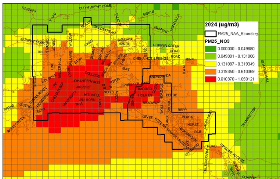
Figure 7.8.14.2-5 Non-attainment area grid cell plot for the modeling year 2024 24-hr average nitrate ( \mu\text{g}/\text{m}^3 ) for all episode days
