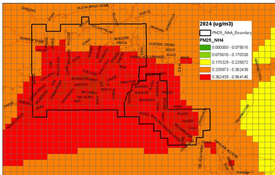
Figure 7.8.14.2-6 Non-attainment area grid cell plot for the modeling year 2024 24-hr average ammonium ( \mu\text{g}/\text{m}^3 ) for all episode days
