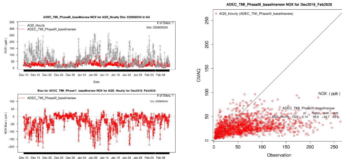
Figure 7.8.15-32 Modeled NOx vs Observed NOy Hourly from the NCore Analyzer in Time Series and Scatter Plots
