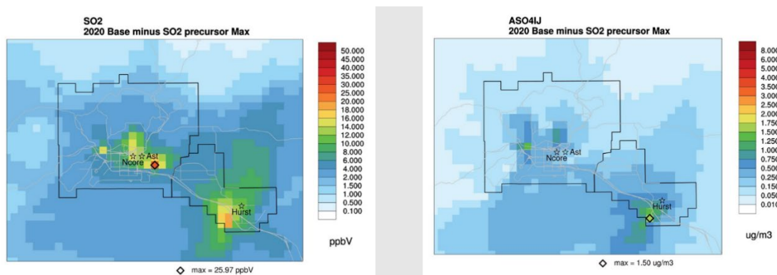
Figure 7.8.18-2 Showing the Max Cell and Max Day in the Entire Nonattainment Area, Grid 91,114 for the SO 2 , and Grid 84,121 for the Sulfate on Jan 28 th , 2020
