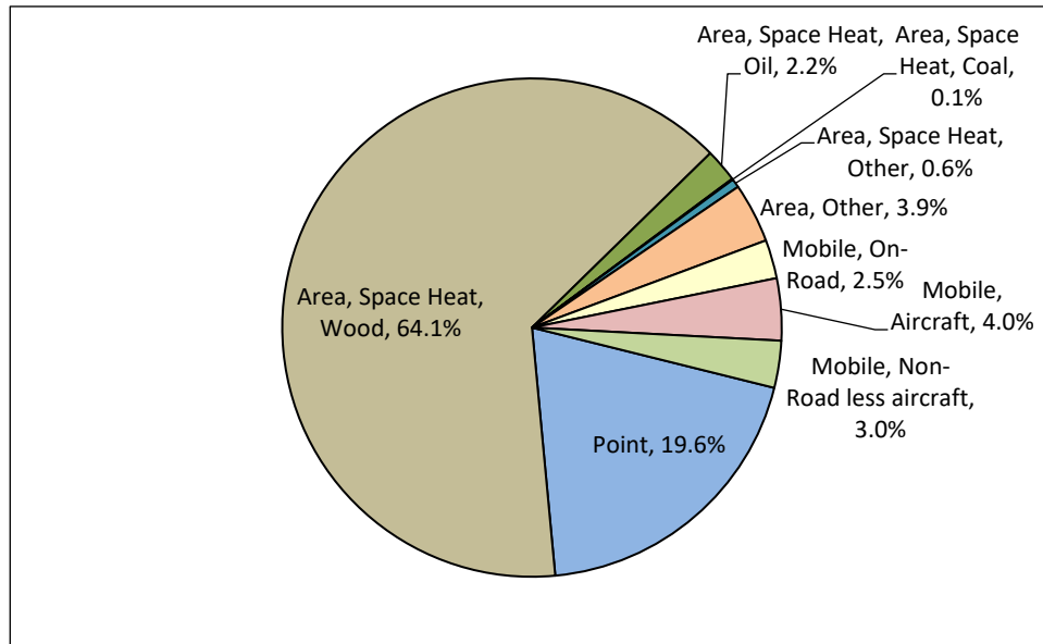
Figure 7.6-6. 2020 Baseline Episodic Nonattainment Area Emissions, Relative PM 2.5 Contributions (%)
