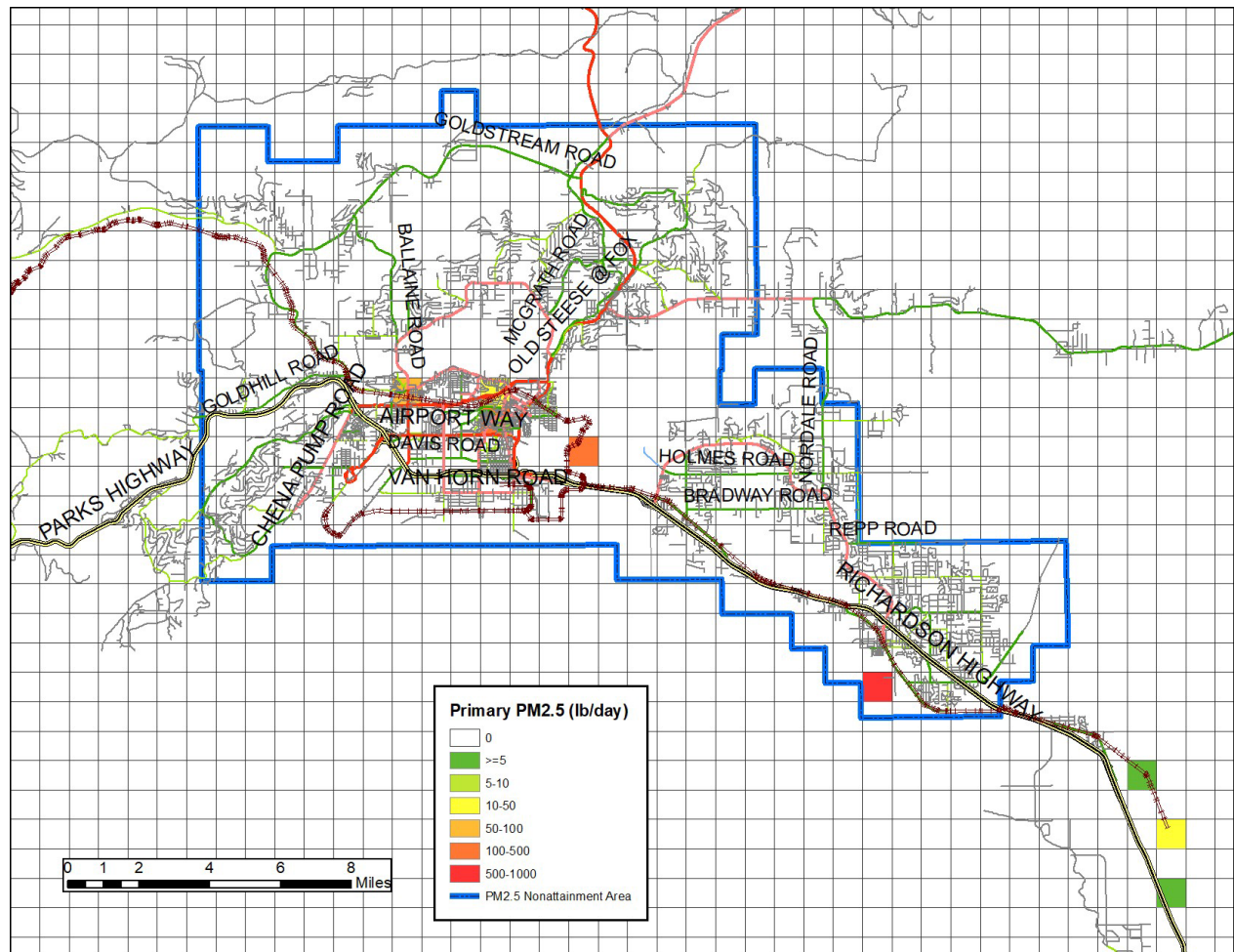
Figure 7.6-39. 2019 Baseline Gridded PM 2.5 Emissions, Point Sources
