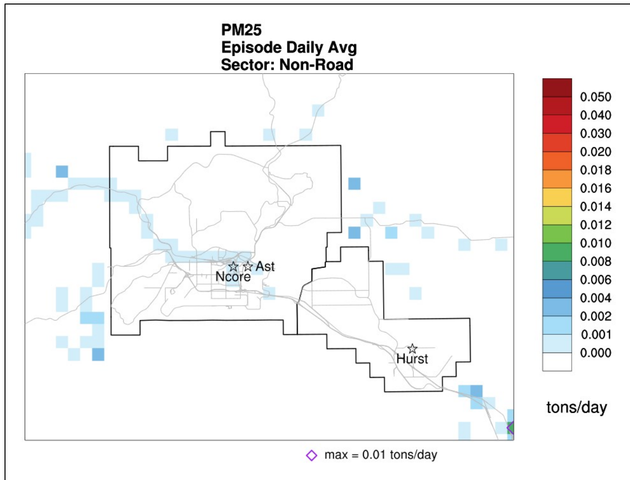
Figure 7.6-16. 2020 Baseline Gridded PM 2.5 Emissions, Nonroad Mobile Sources (including Locotmotives)
