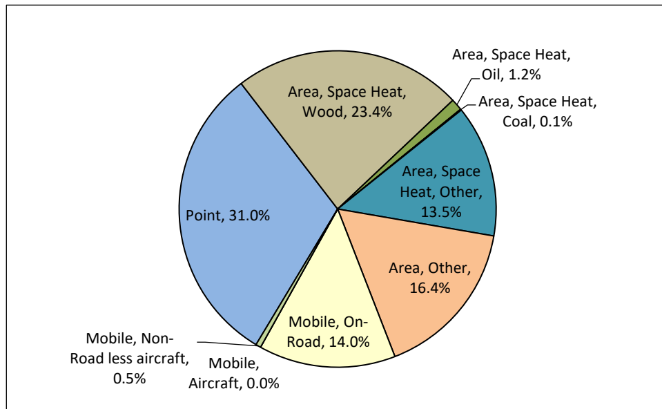
Figure 7.6-10. 2020 Baseline Episodic Nonattainment Area Emissions, Relative NH 3 Contributions (%)
