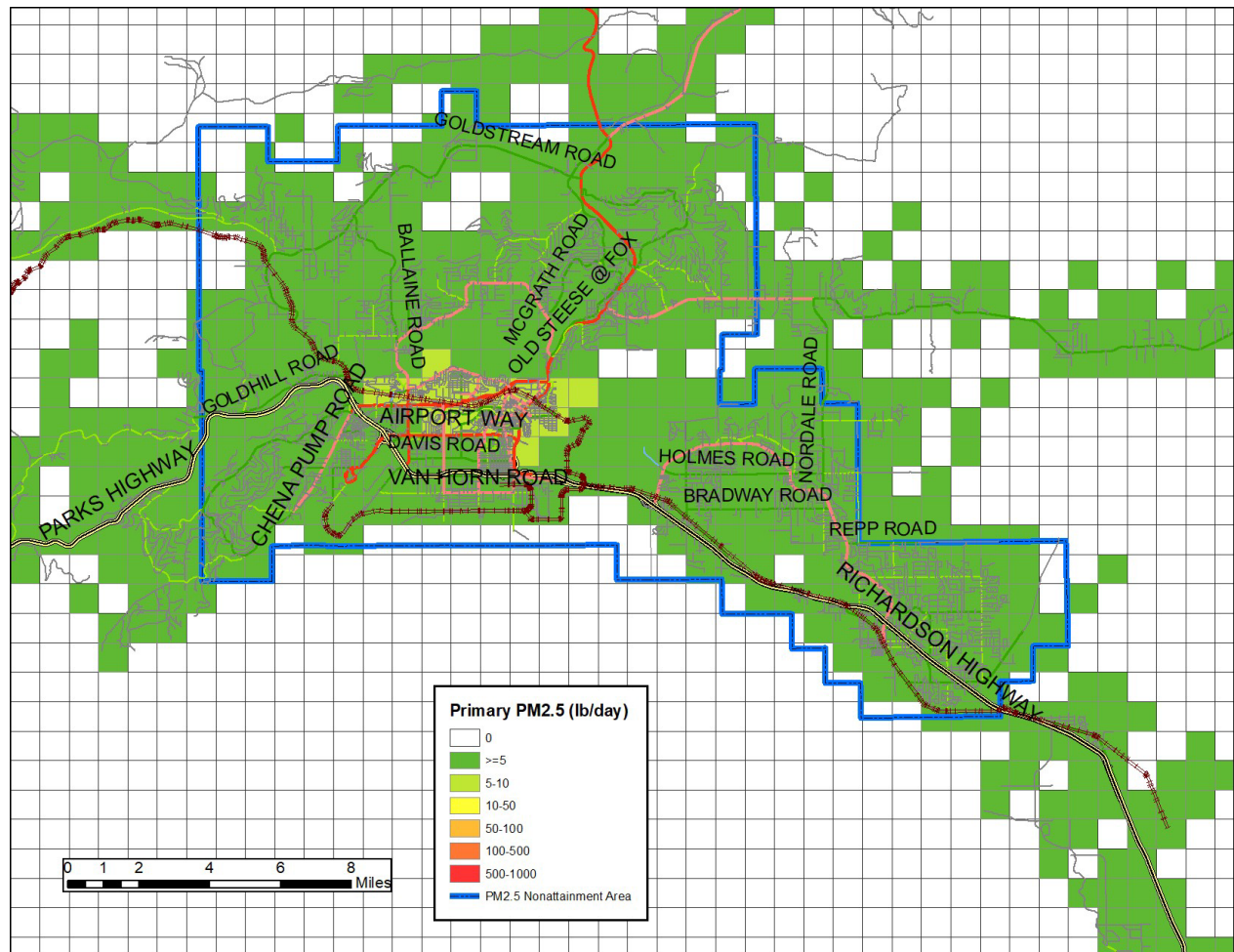
Figure 7.6-40. 2019 Baseline Gridded PM 2.5 Emissions, On-Road Sources
