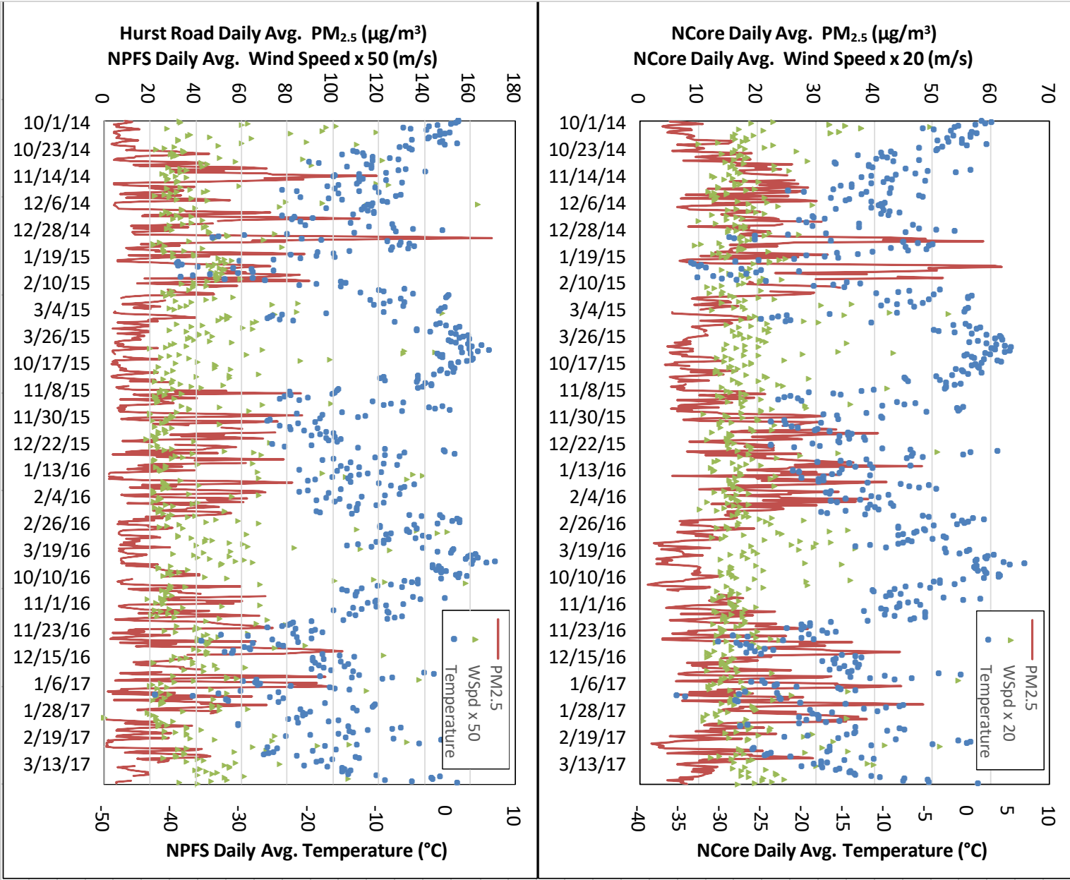
Figure 7.6-7. Fairbanks Winter 2014-2017 Time Series
