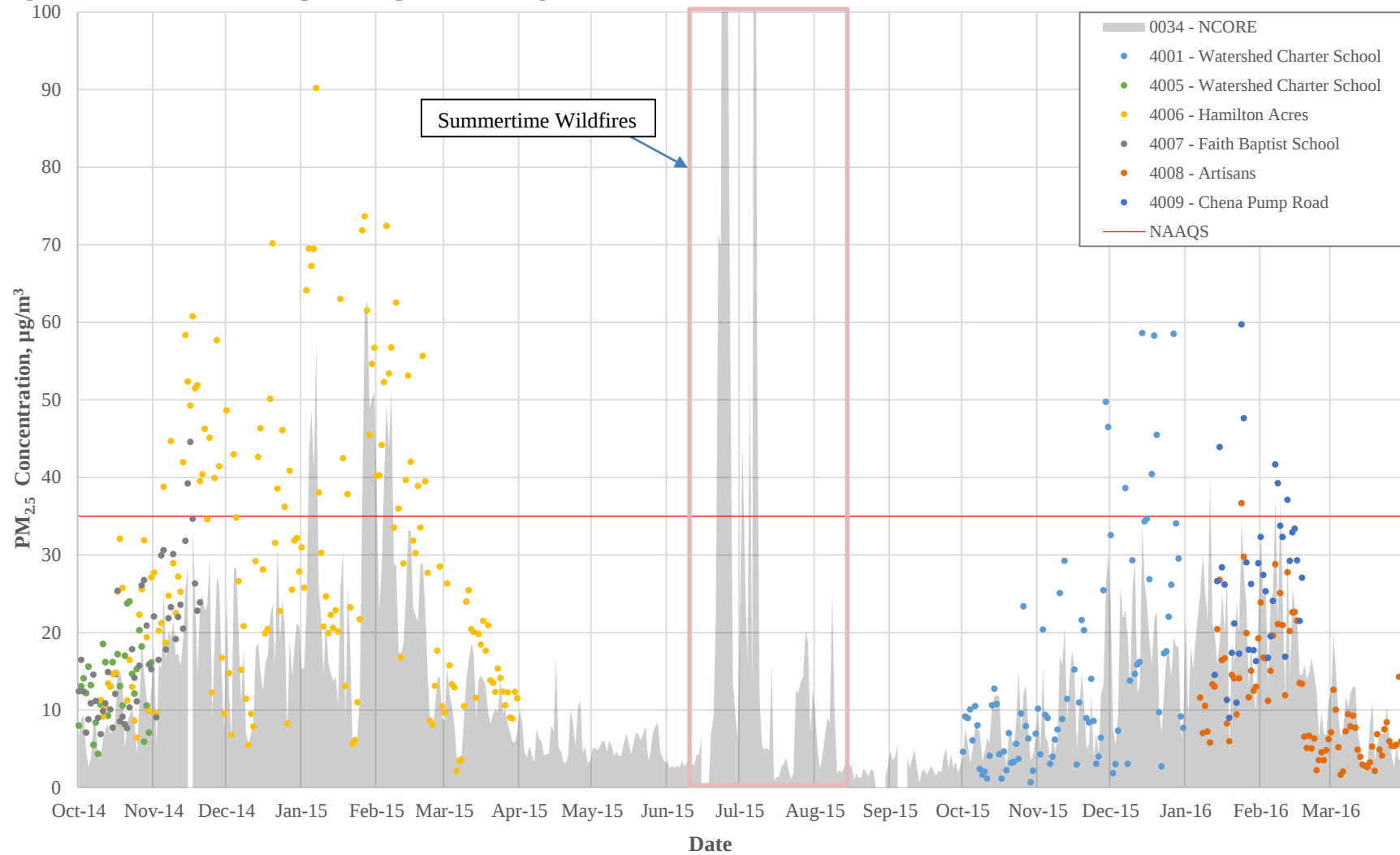
Figure 3-26. Fairbanks PM 2.5 Special Purpose Monitoring Data, 24-hour PM 2.5 Concentrations, October 2014 - March 2016
