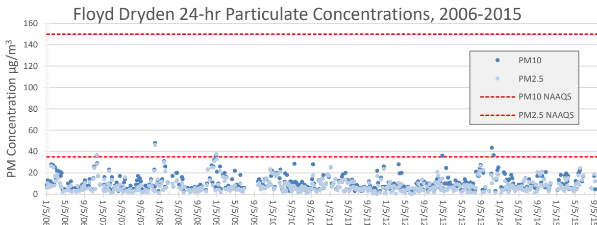
Figure 5-5-1: Floyd Dryden 24-hr Particulate Matter Concentrations from 2006 to 2015. Concentration pairs <3\mu\text{g}/\text{m}^3 were excluded.
