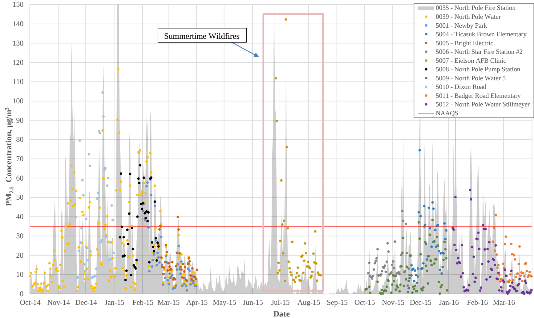
Figure 3-27. North Pole PM 2.5 Special Purpose Monitoring Data, 24-hour PM 2.5 Concentrations, October 2014 - March 2016
