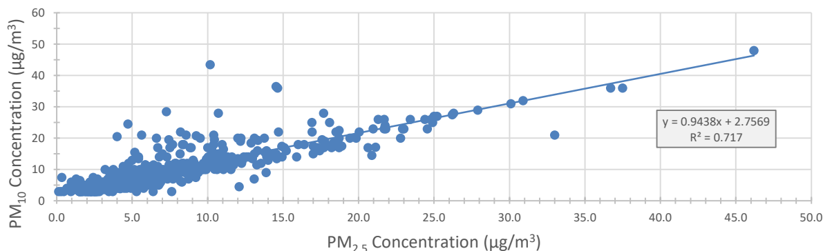
Figure 5-5-3: Correlation between PM 2.5 and PM 10 at Floyd Dryden from 2006-2015. Concentrations <3µg/m 3 were excluded.
