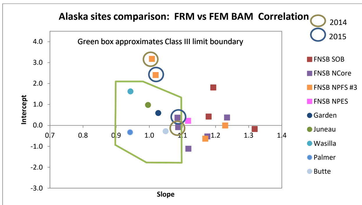
Figure 3-28: Alaska FRM FEM Correlations; the green box shows Class III performance criteria
