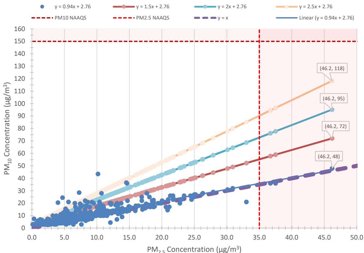
Figure 5-5-4: Comparing actual PM10 and PM2.5 concentrations (equation 1) to the predicted PM10 concentrations using proposed models (equations 2-4).
